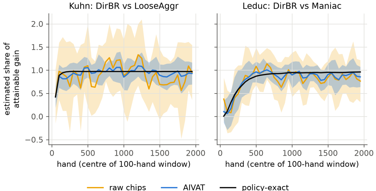
Figure 4: Share of the attainable gain estimated in 100-hand windows from raw chips, from AIVAT and from the exact policy values, for DirBR against LooseAggr (Kuhn) and Maniac (Leduc). Lines are means and bands \pm 1 SD over 20 matches.
