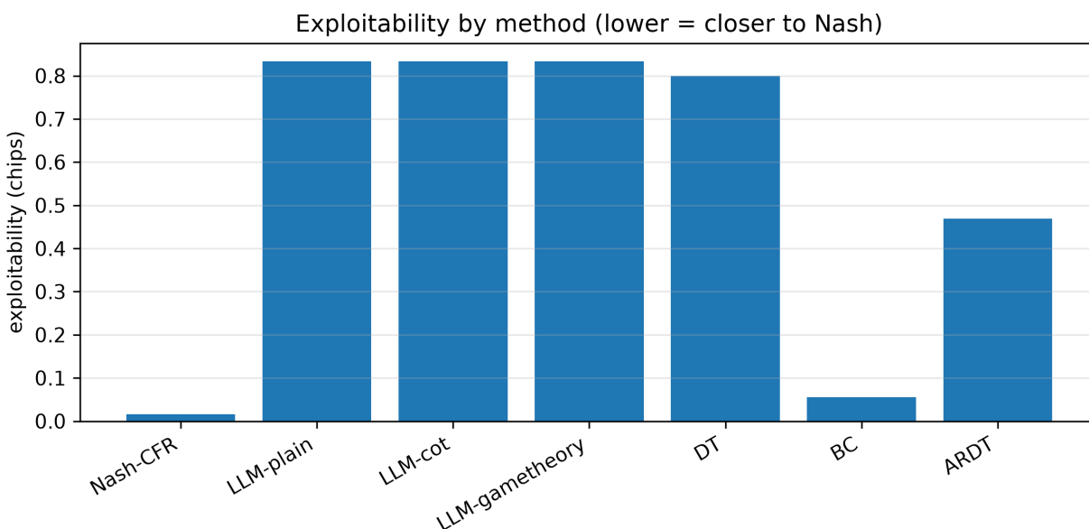
Figure 41: Exploitability by method on the exact Kuhn metric — plain behavioural cloning, included only as a contrast baseline, beats both of the methods this chapter is named after. The LLM row is the scripted offline stub, not a language model.
