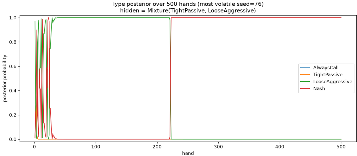
Figure 21: Hidden = Mixture, 500 hands (most volatile seed): a wrong type can dominate for 200 hands before Nash overtakes; once locked, Nash never falls.
