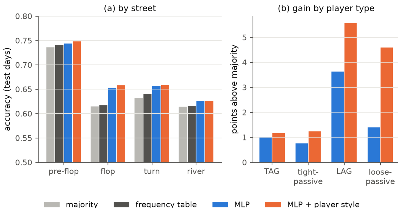
Figure 80: Behavioral cloning on the iPoker test days: (a) accuracy by street for the majority baseline, the frequency table, the MLP and the MLP with the player’s style vector (3-seed means); (b) accuracy above the majority baseline by player type. Knowing the player helps most for the loose players.
