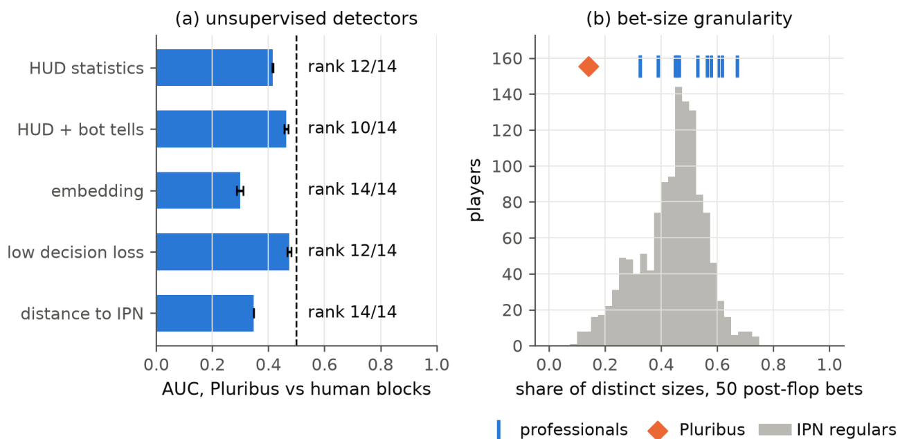
Figure 85: (a) Five unsupervised detectors on 250-hand blocks of the Pluribus games: AUC of Pluribus’s blocks against the professionals’ (3 seeds) and Pluribus’s rank among 14 players by mean score; (b) share of distinct bet sizes among 50 random post-flop bets of each player: iPoker regulars (histogram), the 13 professionals (ticks) and Pluribus.
