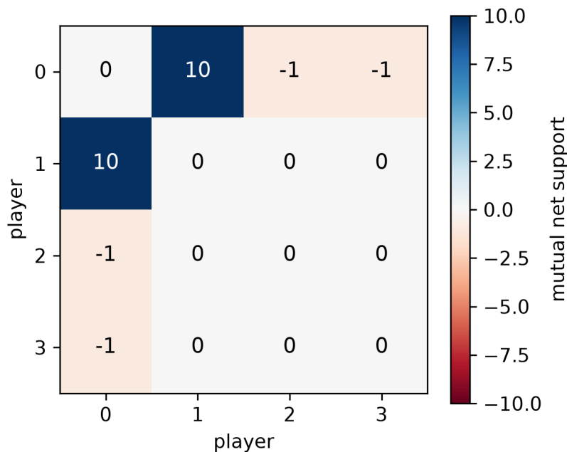
Figure 64: Coalition-score matrix inferred purely from chip placement: the planted alliance between players 0 and 1 shows as strong mutual support (10), while the other pairs are neutral (0) or hostile (-1). The detector recovers a coalition it was never told about.
