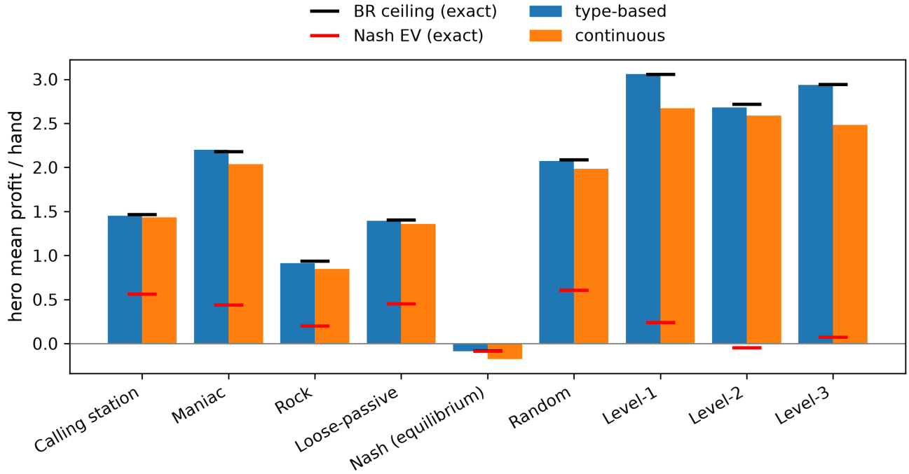
Figure 36: Exploitation against each Leduc opponent: the type-based model (which fits these opponents) hugs the exact best-response ceiling, while the continuous model tracks close but sits below for the hardest-to-fit types — and dips below the safe baseline against Nash.
