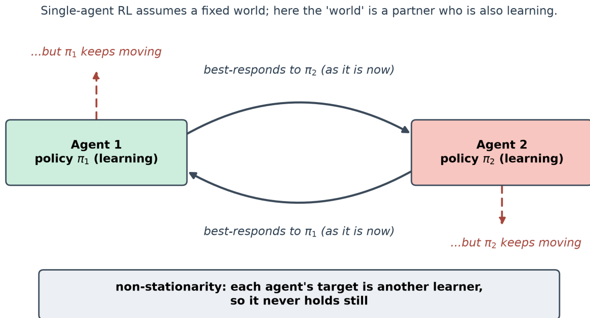
Figure 44: Non-stationarity as two partners learning to dance at once. Each agent optimizes against the other’s current policy (the solid arrows), but that policy is itself moving because the other agent is optimizing back (the dashed arrows). The target each one chases is never still, so naive learners cycle or over-correct rather than converge. Every method in this chapter is a different way to make the moving target hold still long enough to learn against.
