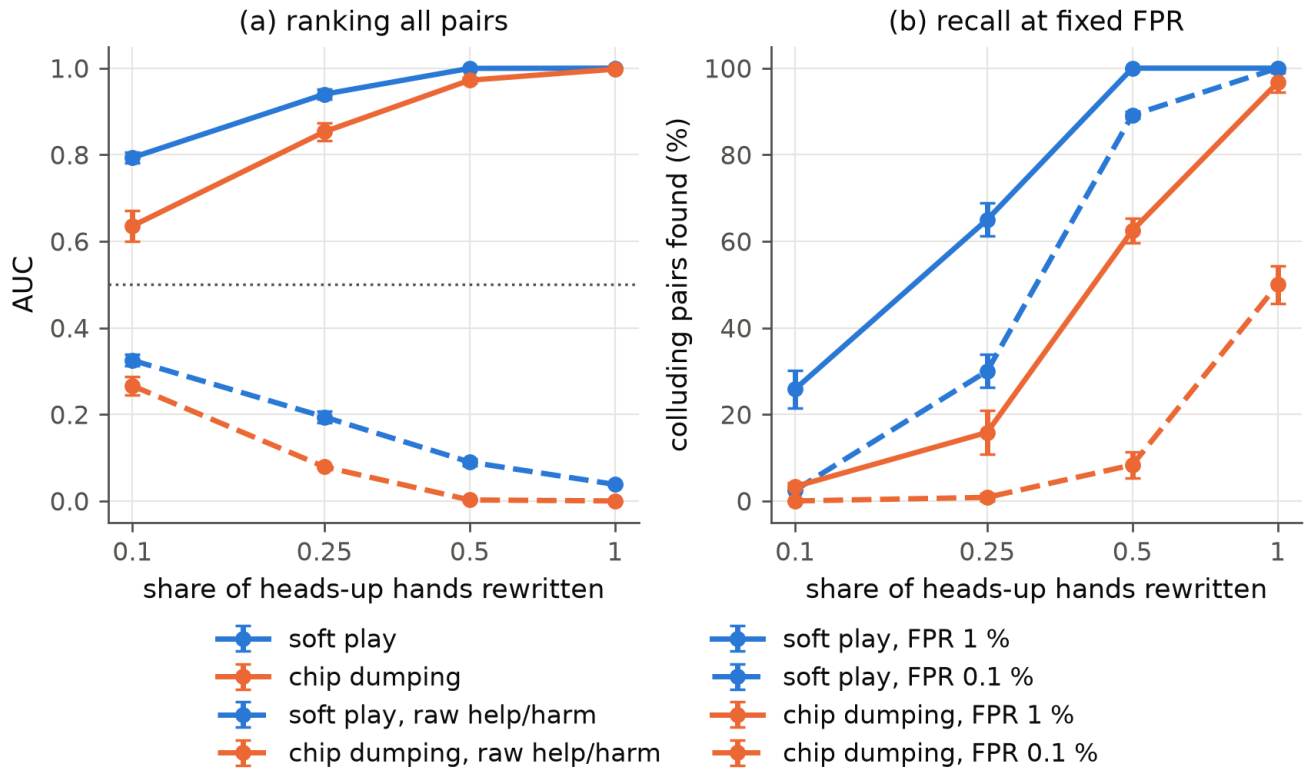
Figure 84: Collusion injected into real iPoker sessions (multiway tables, 3 seeds, \pm 1 SE): (a) AUC of the union detector and of Chapter 11’s raw help/harm score against the share of heads-up hands rewritten; (b) share of colluding pairs found at a false-positive rate of 1 % and 0.1 % among 2,802 real pairs.
