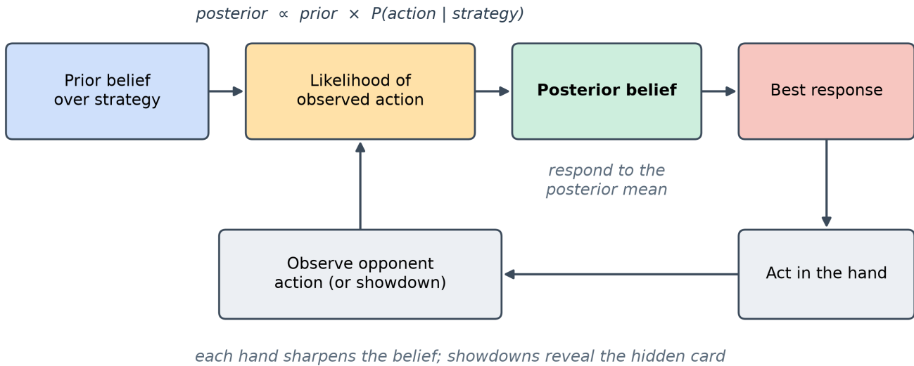
Figure 32: The opponent-modeling loop: a prior belief is multiplied by the likelihood of each observed action to give a posterior, which drives a best response; the outcome feeds the next observation.
