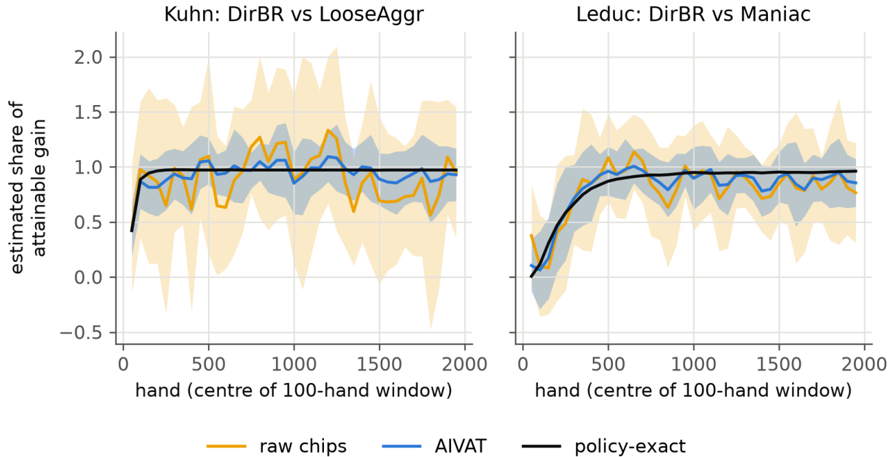
Figure 89: Share of the attainable gain estimated in 100-hand windows from raw chips, from AIVAT and from the exact policy values, for DirBR against LooseAggr (Kuhn) and Maniac (Leduc). Lines are means and bands \pm 1 SD over 20 matches.
