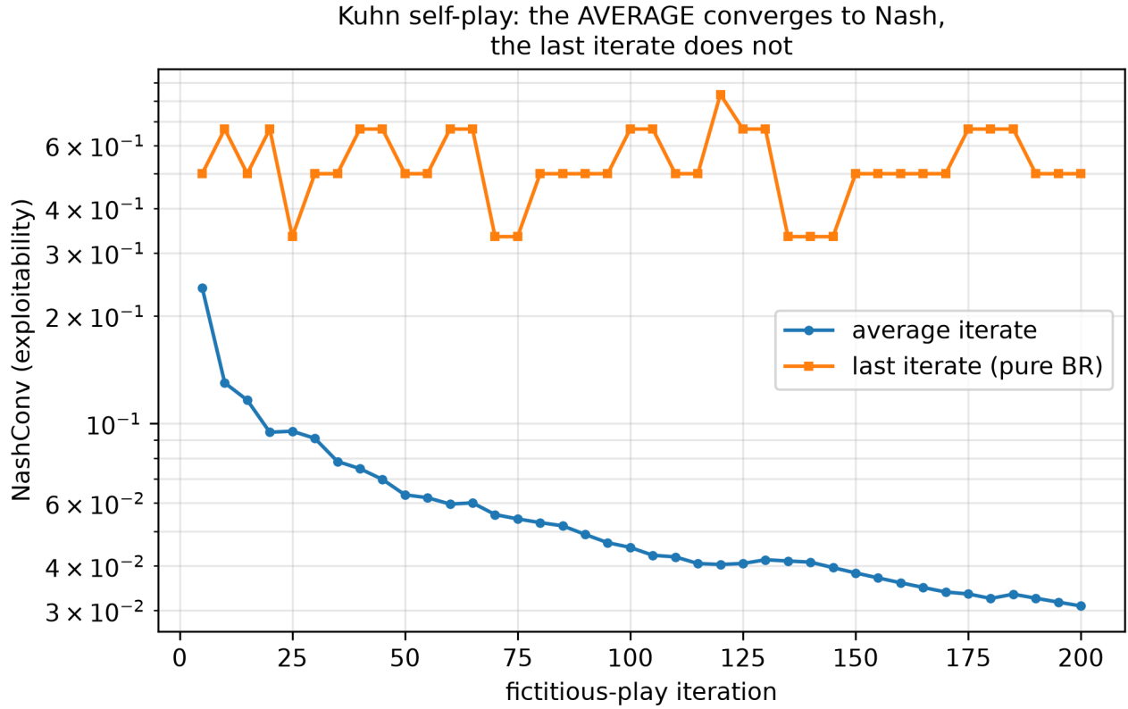
Figure 52: Self-play on Kuhn: the average-iterate exploitability (NashConv) falls steadily toward zero while the last-iterate exploitability keeps oscillating. This is why self-play and PSRO rely on averaging over a population rather than trusting the most recent policy.
