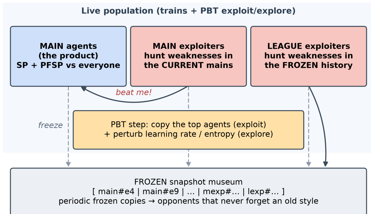
Figure 58: The league: main agents (the product), main exploiters (hunt weaknesses in the current mains), and league exploiters (hunt weaknesses in the frozen history), with periodic freezing into a snapshot museum and PFSP matchmaking that focuses training where the agent is losing. PBT copies the top agents and perturbs their hyper-parameters.
