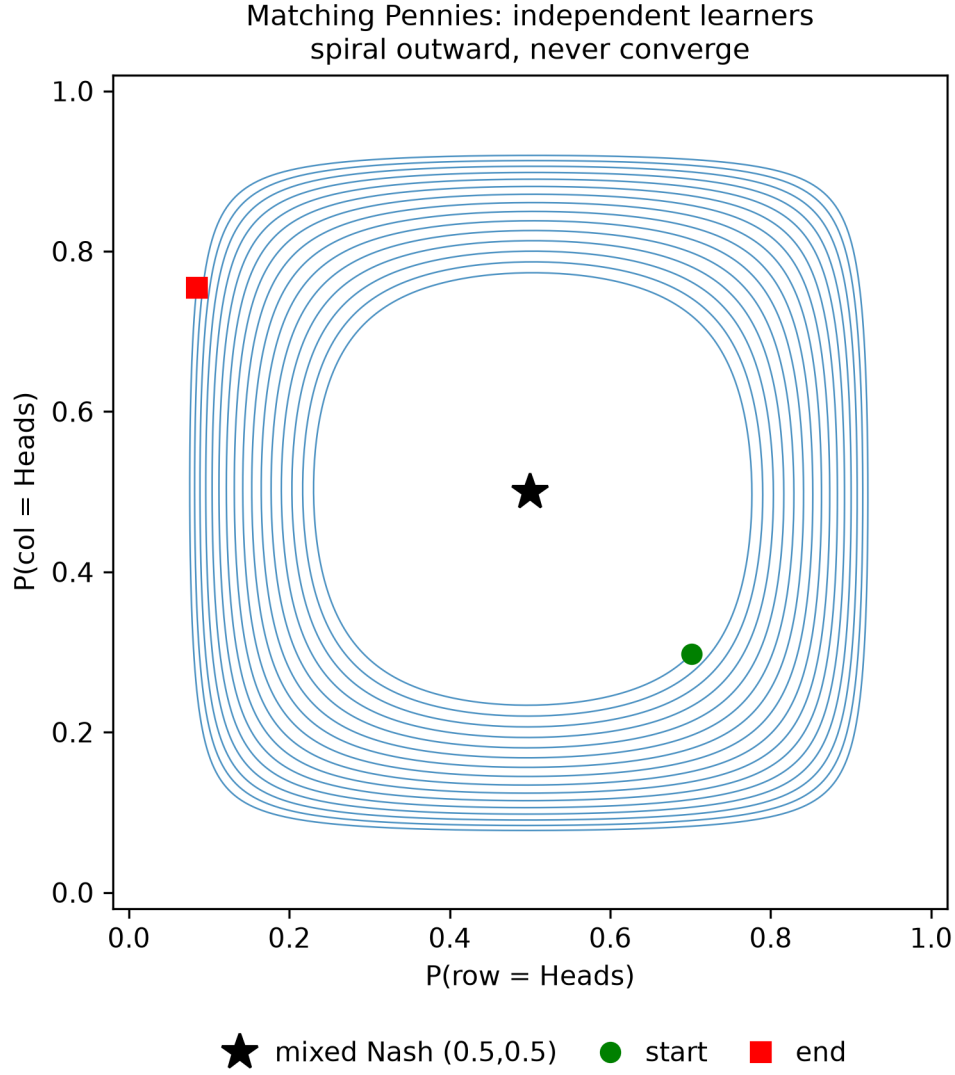
Figure 47: Zoom on non-stationarity: in Matching Pennies the distance to the mixed Nash does not shrink but grows across successive time-windows (from 0.30 to 0.48); the trajectory spirals slowly outward to the boundary. The last iterate does not converge however long training runs.
