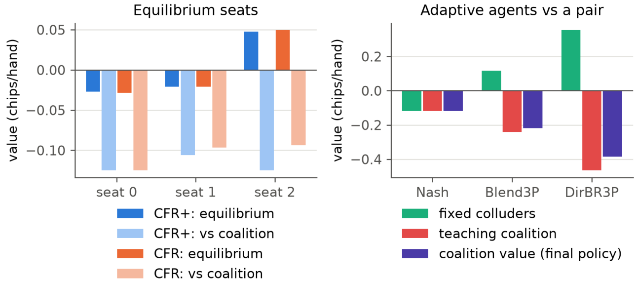
Figure 93: Left: each seat’s value in the CFR+ and CFR equilibria and its coalition value (the worst a coordinated pair can do to that seat’s equilibrium strategy). Right: the mean value of Nash, Blend3P and DirBR3P against a fixed colluding pair (the coalition best response to the blueprint), under a coalition teaching attack after the switch, and the coalition value of each agent’s final policy; 3 seats \times 5 seeds.
