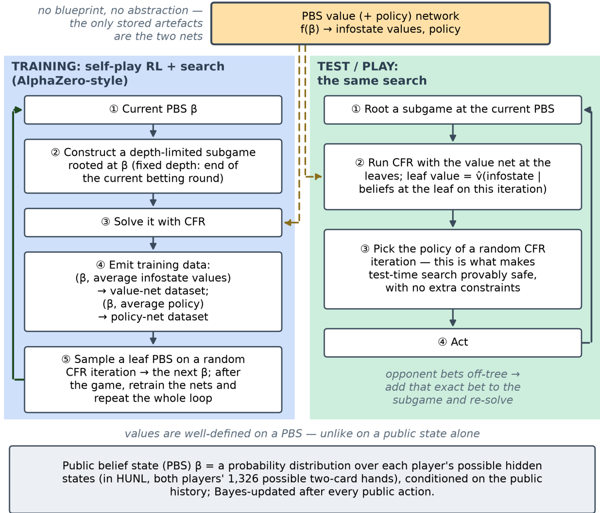
Figure 27: ReBeL’s AlphaZero-style loop: self-play training (left) and test-time play (right) share one PBS value/policy network, both solving depth-limited subgames rooted at the public belief state (shared definition box, bottom).
