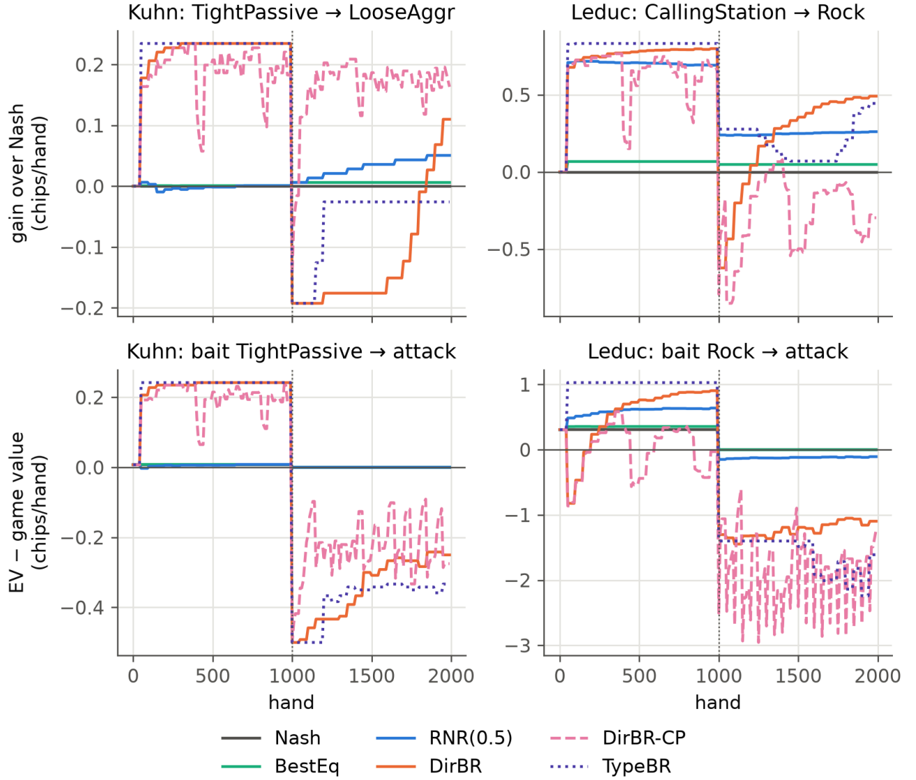
Figure 91: Top: gain over Nash when the opponent switches at hand 1,000 (Kuhn: TightPassive to LooseAggr; Leduc: CallingStation to Rock). Bottom: expected payoff minus the game value under a teaching attack — bait until hand 1,000, then the exact best response to the agent’s current policy, refreshed every 50 hands.
