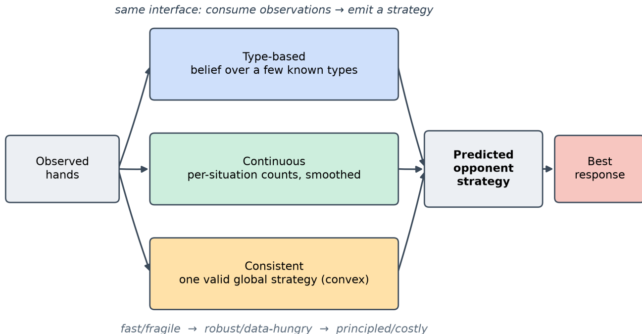
Figure 34: Three models on one interface: a discrete belief over types, a free-form per-situation count, and a globally-consistent sequence-form estimate — all emit a predicted opponent strategy consumed by the same best-response step.
