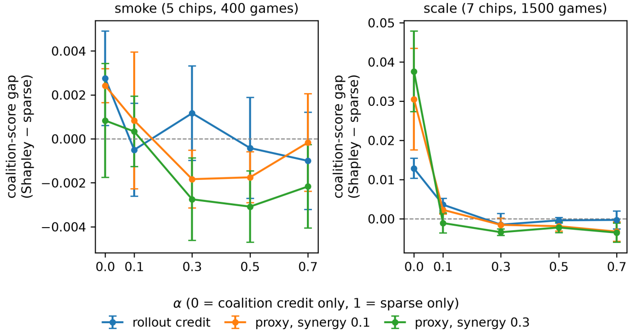
Figure 68: Paired coalition-score gap across the alpha x credit x synergy sweep (5 seeds, error bars = 1 SE): large and significant only in the low-alpha regime (peaking at +0.038 with the proxy at alpha=0); in the scale tier it is negative for every alpha \geq 0.3 . The earlier null came from measuring in the alpha=0.3 dead zone.
