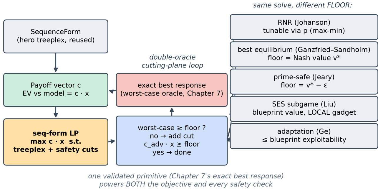
Figure 39: One LP engine, five safety floors. The sequence-form treeplex gives a linear objective (EV vs the model); a constraint-generation loop calls an exact best response as the worst-case oracle and adds a safety cut until the floor is met. RNR, best equilibrium (the Ganzfried–Sandholm baseline), prime-safe, SES and adaptation are the SAME solve with a different floor — and one validated primitive (Chapter 7’s best response) powers both the objective and every safety check.
