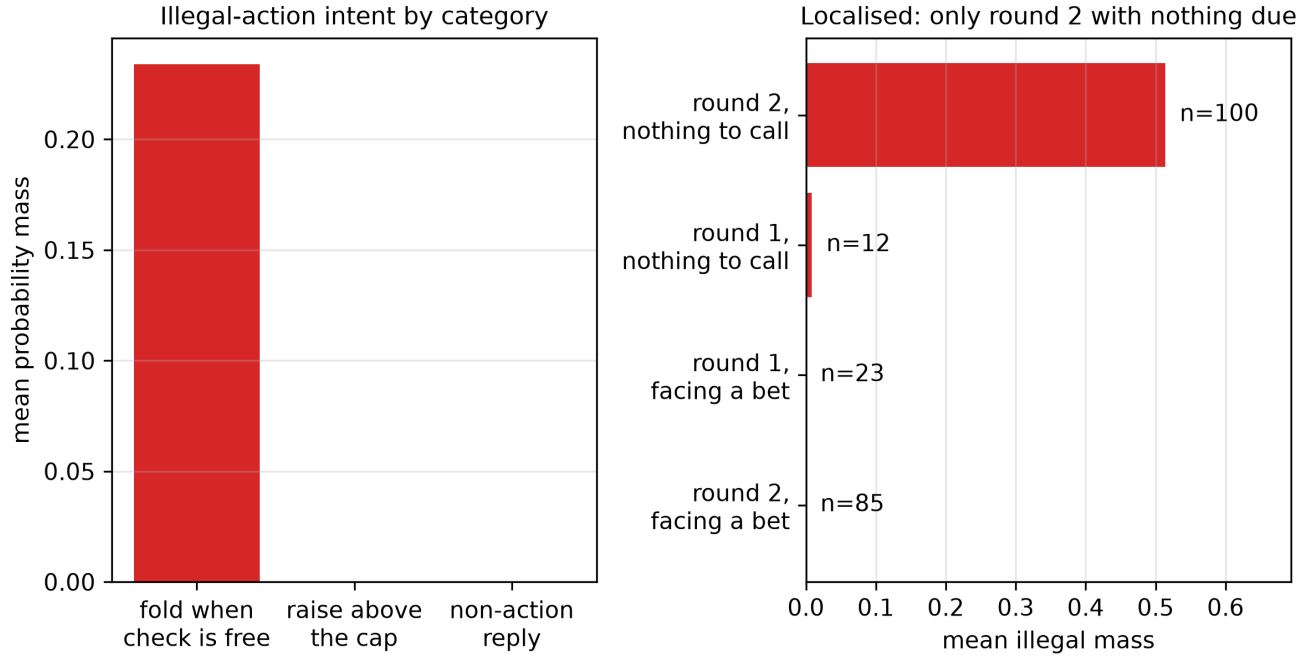
Figure 75: Illegal-action intent on Leduc Hold'em (Qwen2.5-7B-Instruct) by category and by situation (on average 0.234 of the probability mass over 220 information sets): almost all of it is folding when a check is free, in the second betting round.
