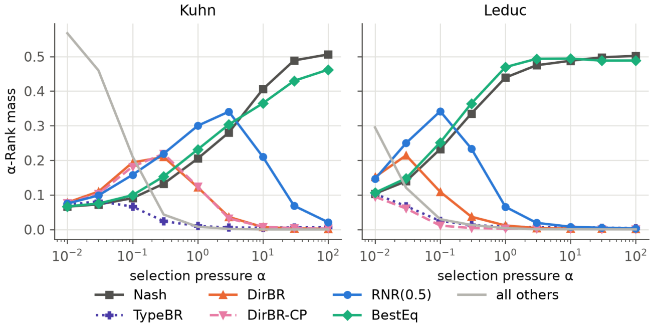
Figure 88: \alpha -Rank mass of the main agents as the selection pressure \alpha grows. On Kuhn the top agent is DirBR for \alpha \leq 0.1 , RNR(0.5) for 0.3 \leq \alpha \leq 3 and Nash for \alpha \geq 10 ; on Leduc it moves from DirBR to RNR(0.5), to BestEq and finally to Nash.
