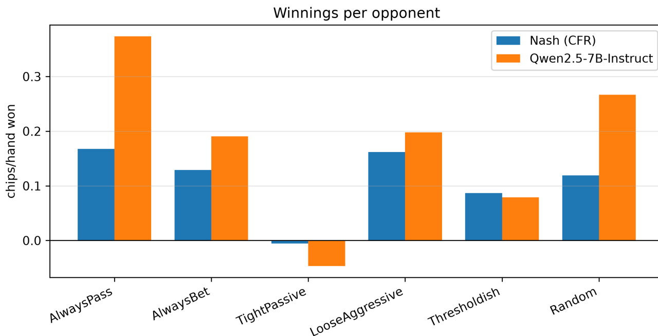
Figure 74: Winnings against each opponent in the zoo: Qwen2.5-7B-Instruct wins 0.177 chips per hand on average (equilibrium: 0.110) at an exploitability of 0.357 chips (equilibrium: 0.006).
