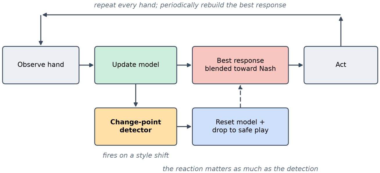
Figure 37: The adaptive exploitation loop: observe, update the model, best-respond (blended toward Nash for safety), and act; a change-point detector can reset the model when the opponent’s style shifts.
