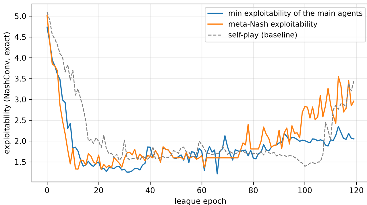
Figure 59: League exploitability (NashConv) over 120 epochs (scale): the minimum over the main agents and the meta-Nash exploitability fall steeply within the first ~15 epochs, are lowest around epochs 20-40, and rise again late in training. The frozen snapshots keep the strong agents of the first half of the run; the live agents degrade late. The dashed grey line is self-play (baseline), which also degrades after epoch 100.
