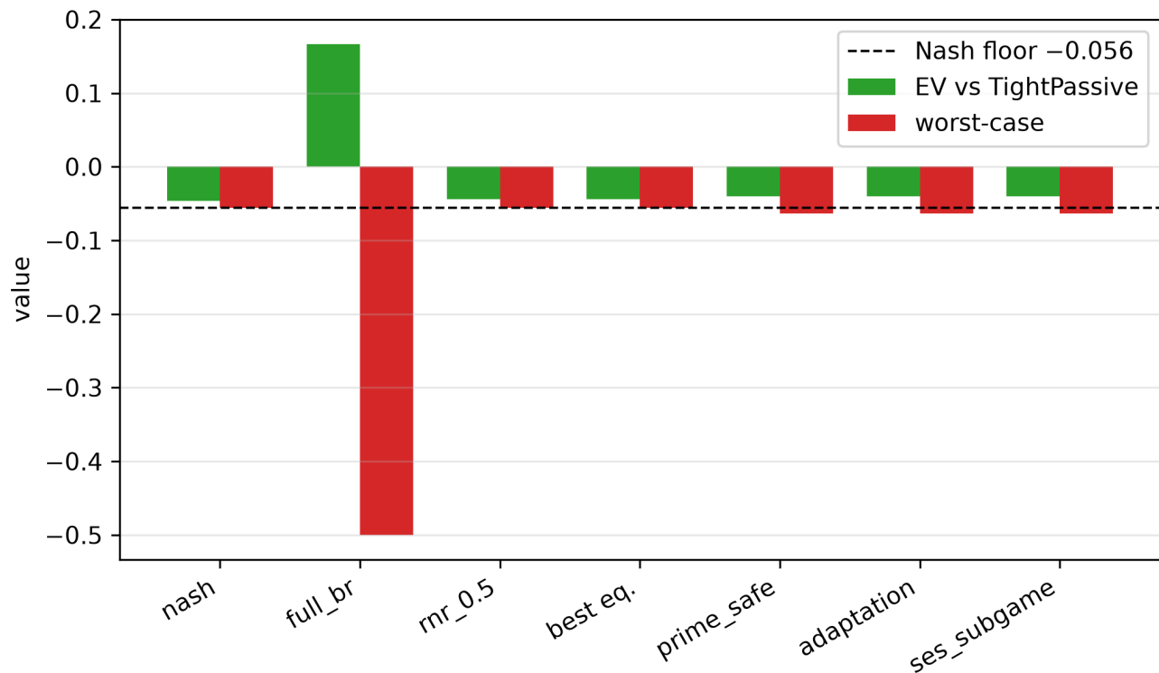
Figure 41: Methods versus the Rock on Kuhn: green is EV against the opponent, red is worst-case value, the dashed line is the Nash floor. Only the full best response’s worst-case (red) plunges to -0.5 , far below the floor; every principled method stays near the floor and earns as much as Nash or slightly more.
