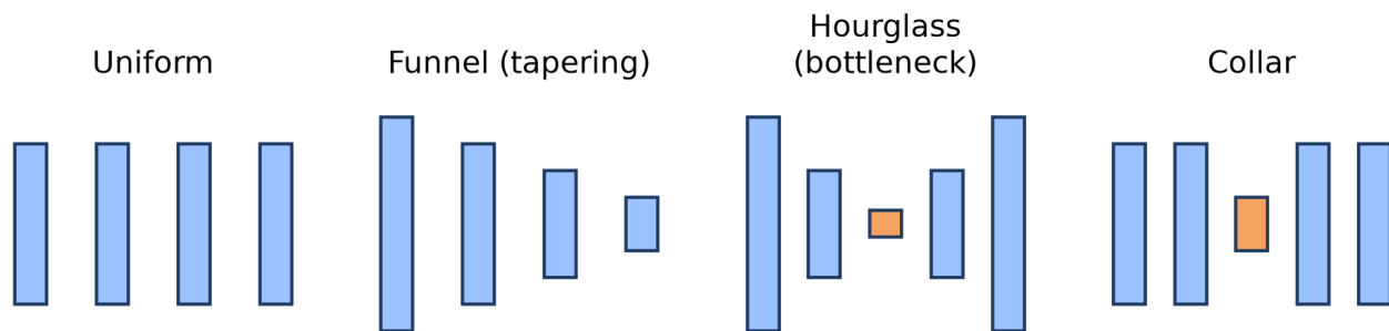
Figure 20: Common network shapes: a uniform stack, a tapering funnel, an hourglass with a central bottleneck (orange), and a uniform stack with a single narrow collar (orange). Bar height represents layer width.
