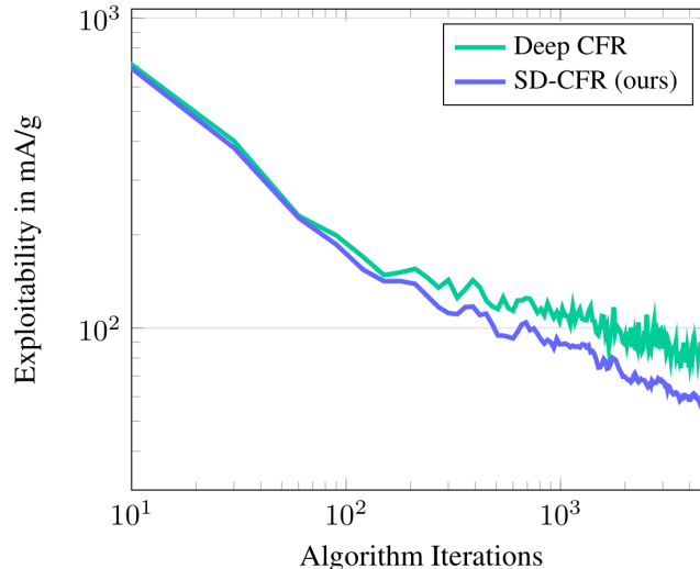
Figure 21: Single Deep CFR (SD-CFR) reaches the same or slightly lower exploitability than Deep CFR on Leduc (in milli-antes per game, mA/g) without training an average-strategy network. Reproduced from Steinberger (2019), Fig. 1a — not an experiment from this work.
