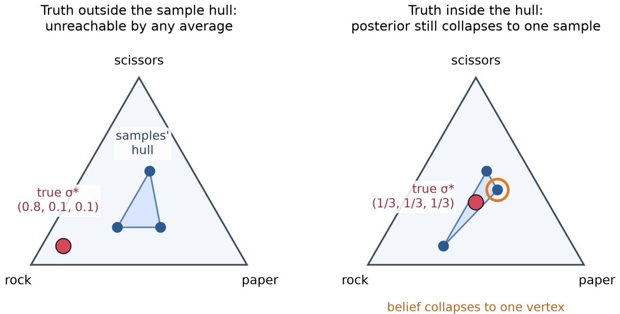
Figure 35: Why fitting the mean can miss the truth: the modeler can only ever produce points in the shaded hull of its samples. A true strategy outside the hull is unreachable; even one inside is abandoned as the posterior collapses onto a single vertex.
