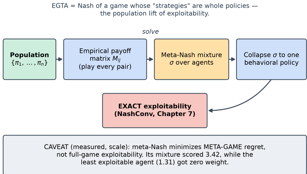
Figure 61: The EGTA pipeline: play every pair of agents to build an empirical payoff matrix, solve its meta-Nash mixture, collapse the mixture to a single behavioral policy, and measure its EXACT full-game exploitability. The measured caveat: the meta-Nash minimizes meta-game regret, not full-game exploitability, so the mixture can be more exploitable than the population’s best member, which may not even be in it.
