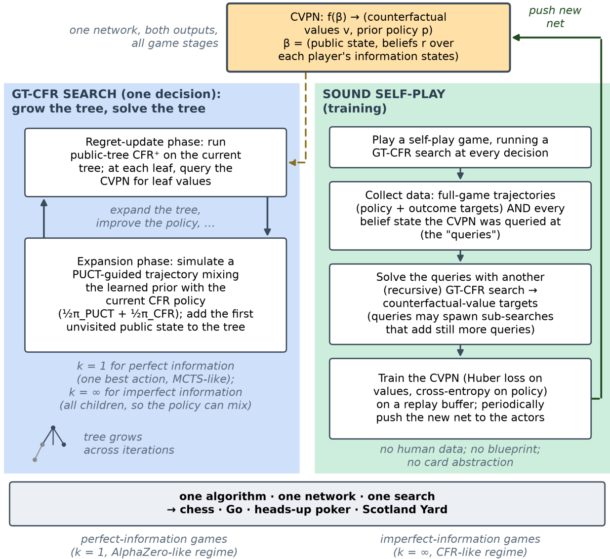
Figure 28: Student of Games: the GT-CFR search loop (left) and the sound self-play training loop that feeds it (right) share one CVPN; the footer strip names the unification across perfect- and imperfect-information games.
