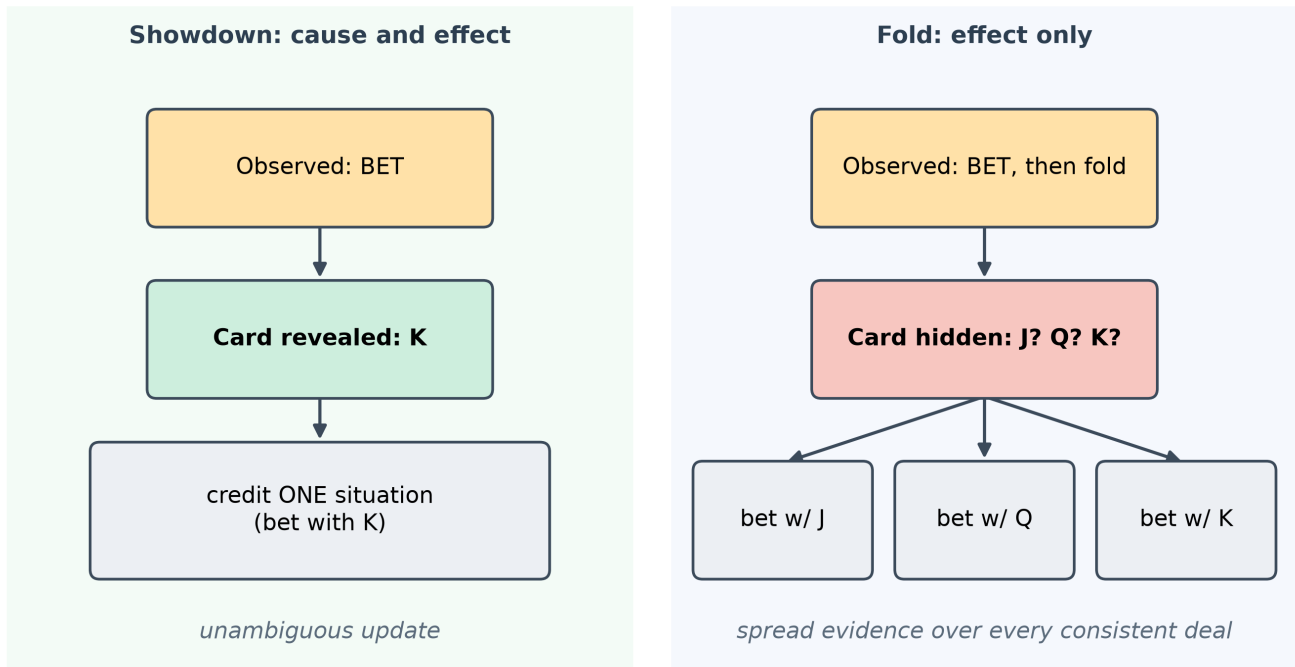
Figure 33: Partial observability: a showdown reveals the opponent’s private card, pinning the action to one situation; a fold hides it, forcing the model to spread the evidence across every hand the opponent might have held.
