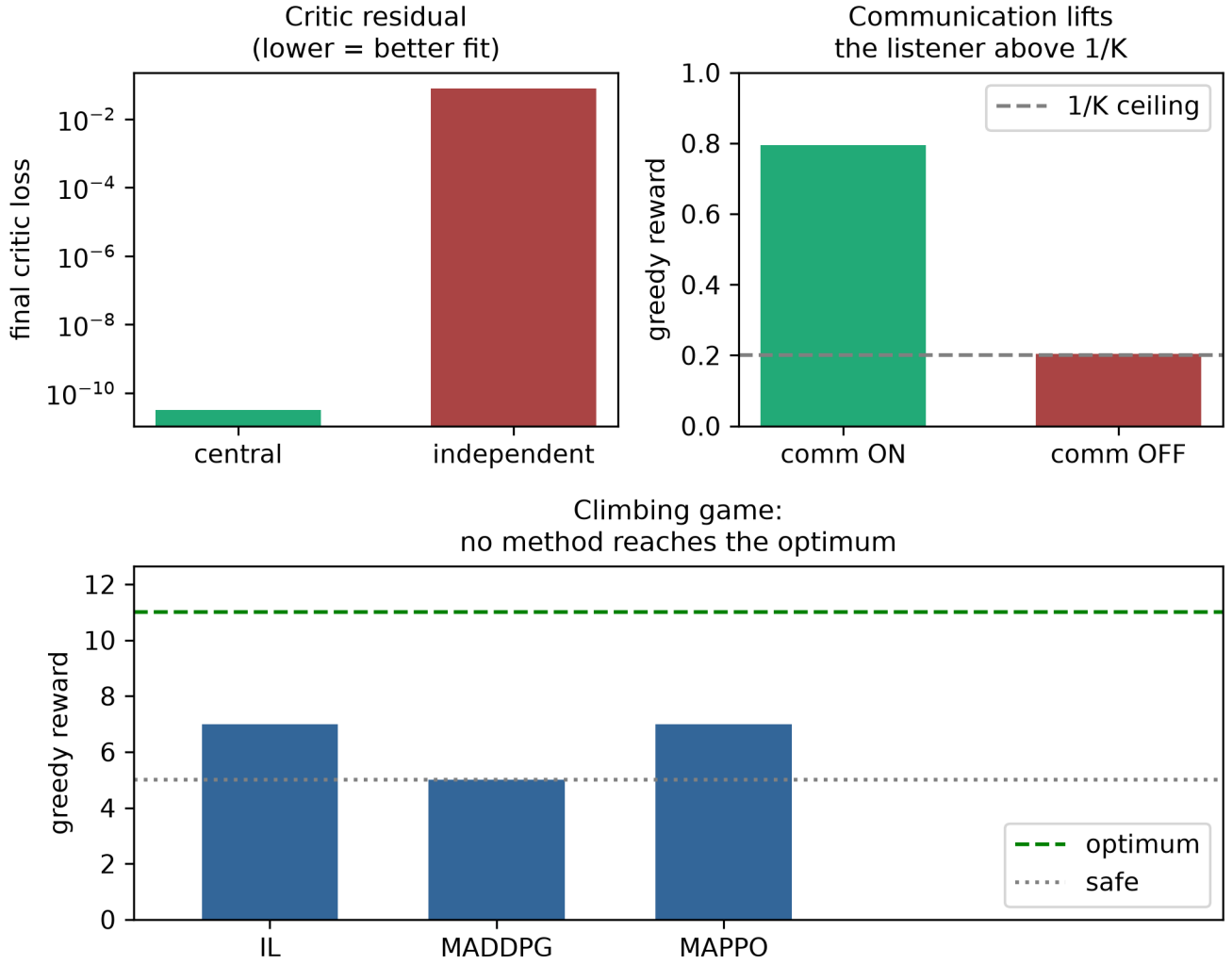
Figure 49: Cooperative CTDE and communication results (scale config). Top left: the centralized critic’s residual is orders of magnitude below the independent critic’s (log scale). Top right: communication lifts the listener far above the 1/K guessing ceiling (see Section 9.7). Bottom: on the climbing game, no method reaches the optimum (11); MADDPG (5) trails IL and MAPPO (7) — CTDE reduces critic variance but does not by itself solve hard-exploration coordination.
