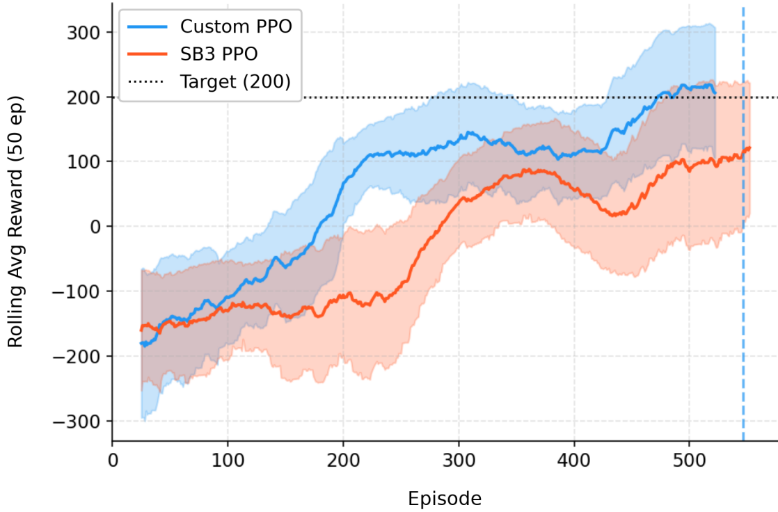
Figure 2: PPO on LunarLander-v3: our implementation (the final run, stopped at episode 547) against SB3 (the first 577 of its 1,224 episodes are shown). Rolling 50-episode average of the reward (shaded: \pm one standard deviation within the window); the dotted line is the 200 target, the dashed vertical line the end of our agent’s training.
