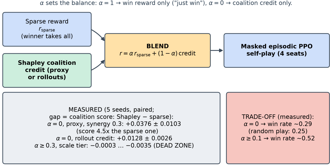
Figure 67: Coalition-aware MAPPO reward blend: the sparse winner-takes-all signal is mixed with the Shapley coalition credit by weight alpha (alpha = 1: sparse only, alpha = 0: credit only). Measured, alpha is the dominant knob: the coalition score rises significantly only at low alpha, and every alpha \geq 0.3 suppresses the signal. The cheap critic-value proxy has a larger effect than the rollout credit.
