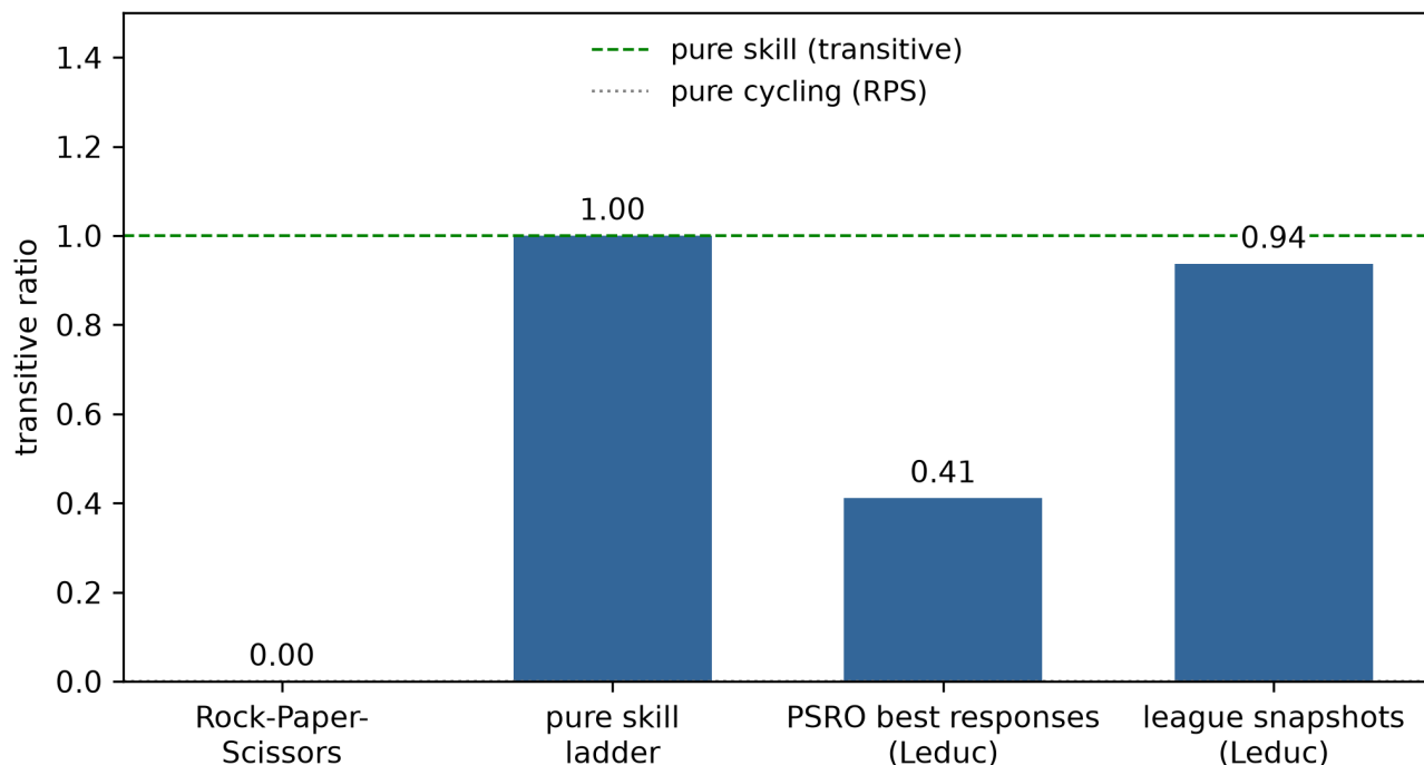
Figure 57: Transitive ratio across four populations: RPS (0.0, purely cyclic), a pure skill ladder (1.0), the PSRO-Leduc best-response meta-game ( \sim 0.41 - 0.46 , mostly cyclic), and the league snapshot meta-game ( \sim 0.94 - 0.98 , mostly transitive). Same game, opposite structure, depending on how the population is built.
