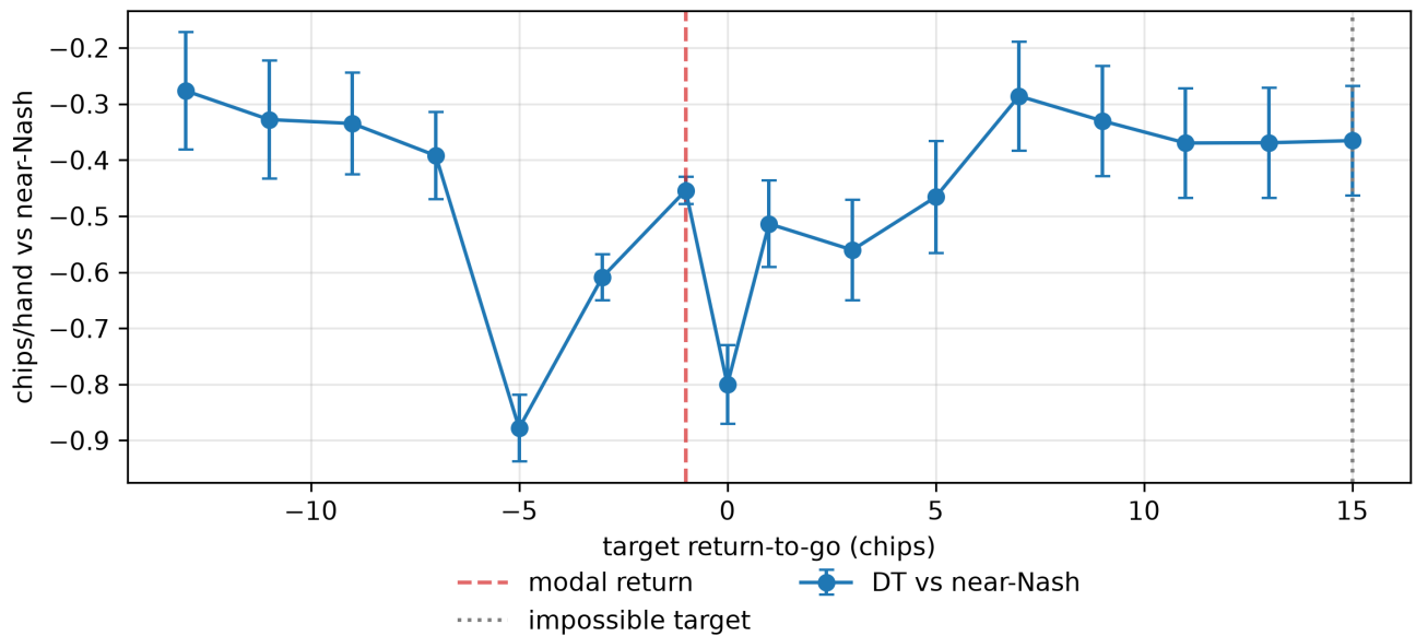
Figure 71: Decision Transformer performance on Leduc Hold’em (chips per hand against a near-Nash opponent) against the conditioned target return, with standard errors (Pearson r = +0.062 ). Dashed line: the most common return ( -1 ); dotted line: the impossible target ( +15 ).
