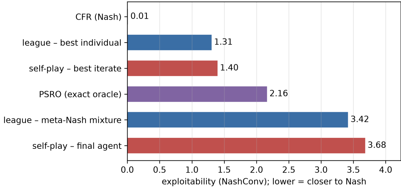
Figure 62: Leduc exploitability (NashConv) by method (scale): CFR-Nash floor \sim 0.01 ; the league’s best individual (1.31, best of the whole run) is comparable to self-play’s best iterate (1.40) and below PSRO (2.16), the league’s meta-Nash mixture (3.42) and the final self-play agent (3.68).
