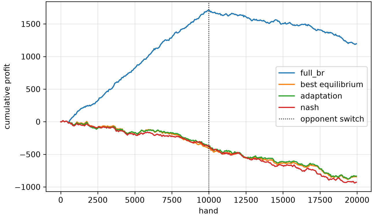
Figure 43: Teaching attack on Kuhn, cumulative profit (the run with seed 0). The full best response (blue) climbs on the bait to about +1700, then only drifts down after the switch — it ends far ahead, because a Nash “revealer” claws back only about the game value per hand. The safe methods refuse the bait and pay the first-player tax throughout.
