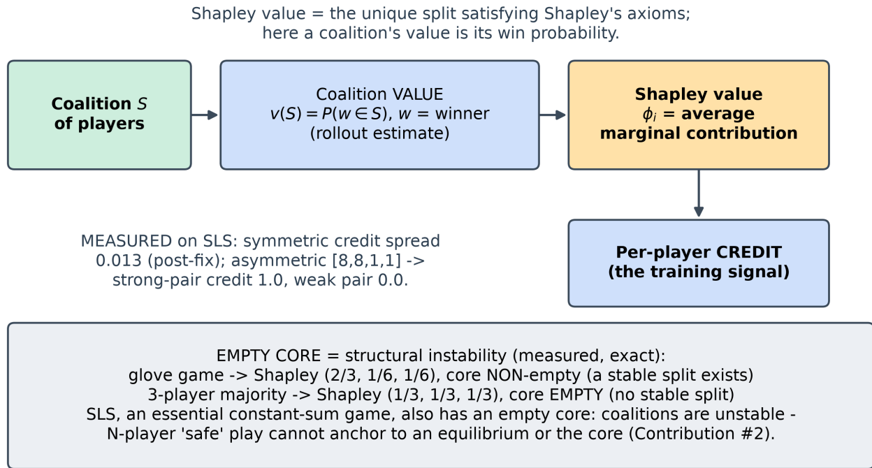
Figure 65: Shapley credit adapted to a purely competitive game: the coalition’s “value” is redefined as the PROBABILITY a coalition member wins (estimated by rollouts), and each player’s Shapley value of that win-probability function is their credit. The empty core of the majority game (no stable allocation) is the structural signature of SLS coalitions - they will break.
