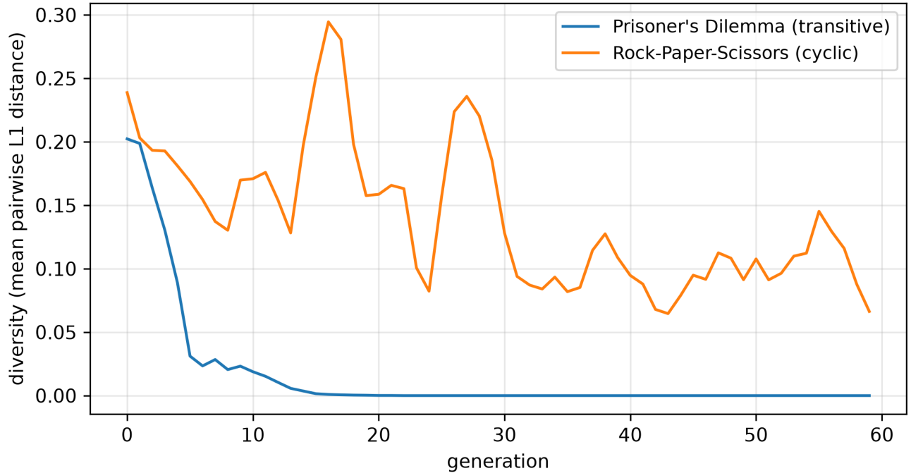
Figure 60: Mini-PBT diversity: on the transitive Prisoner's Dilemma the population collapses to a single strategy (diversity \rightarrow 0), while on cyclic Rock-Paper-Scissors it churns indefinitely (0.07-0.29) as it chases the wheel of counters. Game structure decides whether diversity survives.
