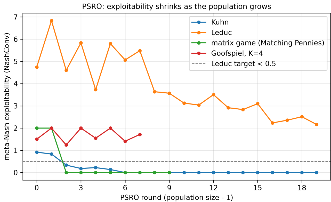
Figure 51: PSRO exploitability vs population size across games (scale config). Kuhn and the matrix game collapse to (near) zero within a handful of rounds; Leduc oscillates for the first eight rounds, then declines but stays well above the 0.5 target after 20 rounds (a scaling wall for a pure-strategy population); Goofspiel K=4 oscillates rather than settling (a flagged anomaly). The exact best-response oracle guarantees convergence in principle; the rate is what size controls.
