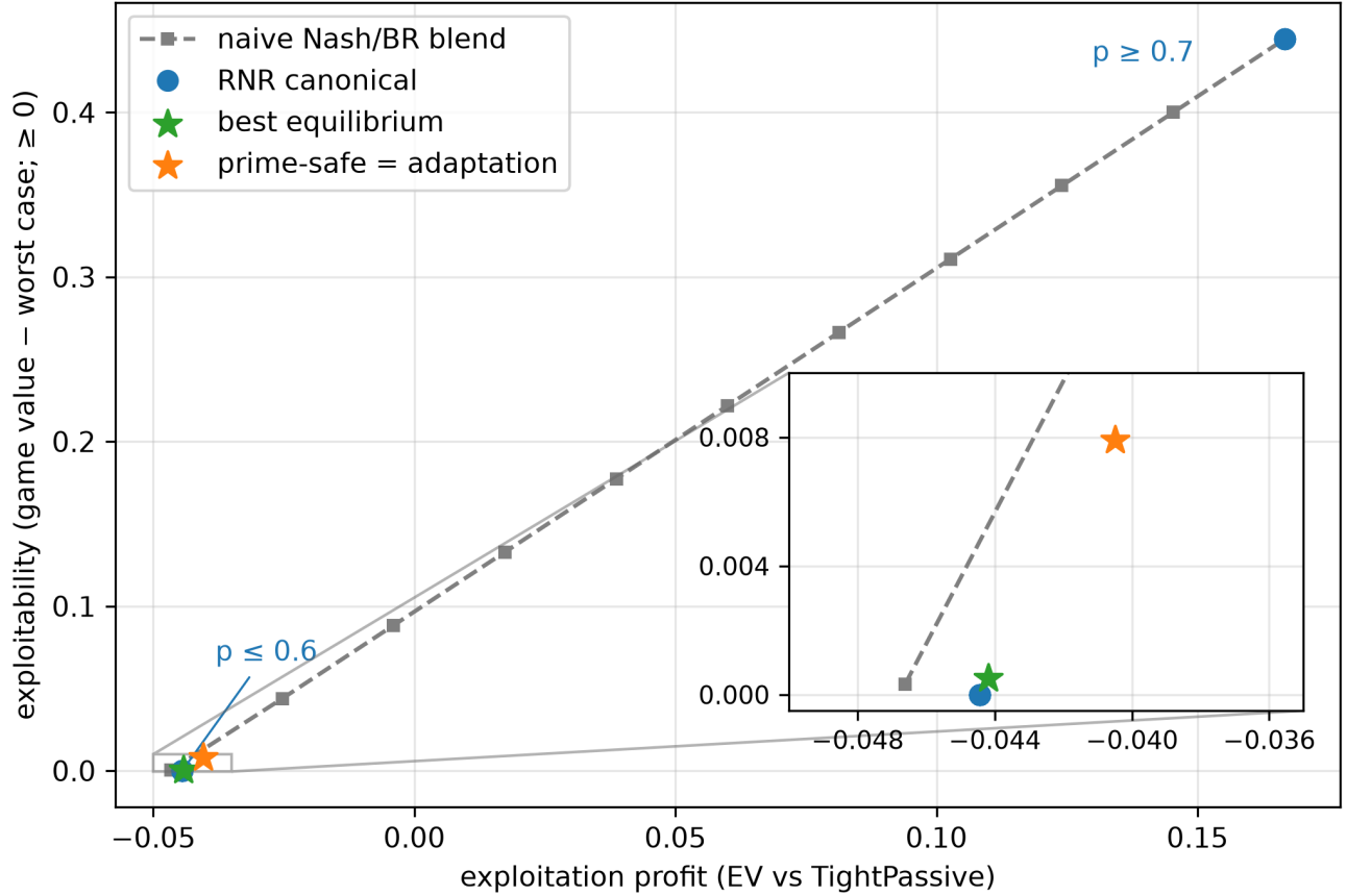
Figure 40: The exploitation-safety frontier on Kuhn with the LP operating points. Canonical RNR returns only two clusters of points (the safe corner for p \leq 0.6 and the full-BR corner for p \geq 0.7 ); the grey line is the dominated naive blend; the stars (best equilibrium, and prime-safe and adaptation, which coincide) sit at the efficient safe corner, enlarged in the inset.
