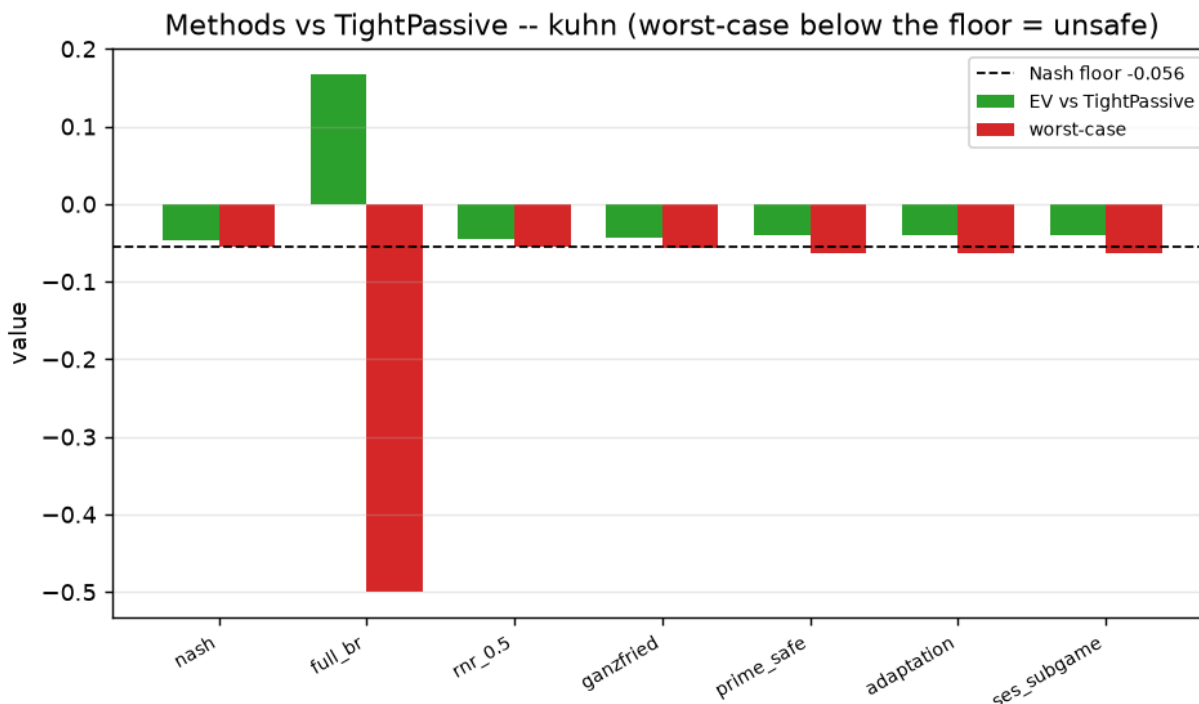
Фигура 29: Methods vs TightPassive (Kuhn): green = EV vs the opponent, red = worst-case value, dashed = the Nash floor. Only full_br's worst-case (red) plunges far below the floor; every other method hugs it.
