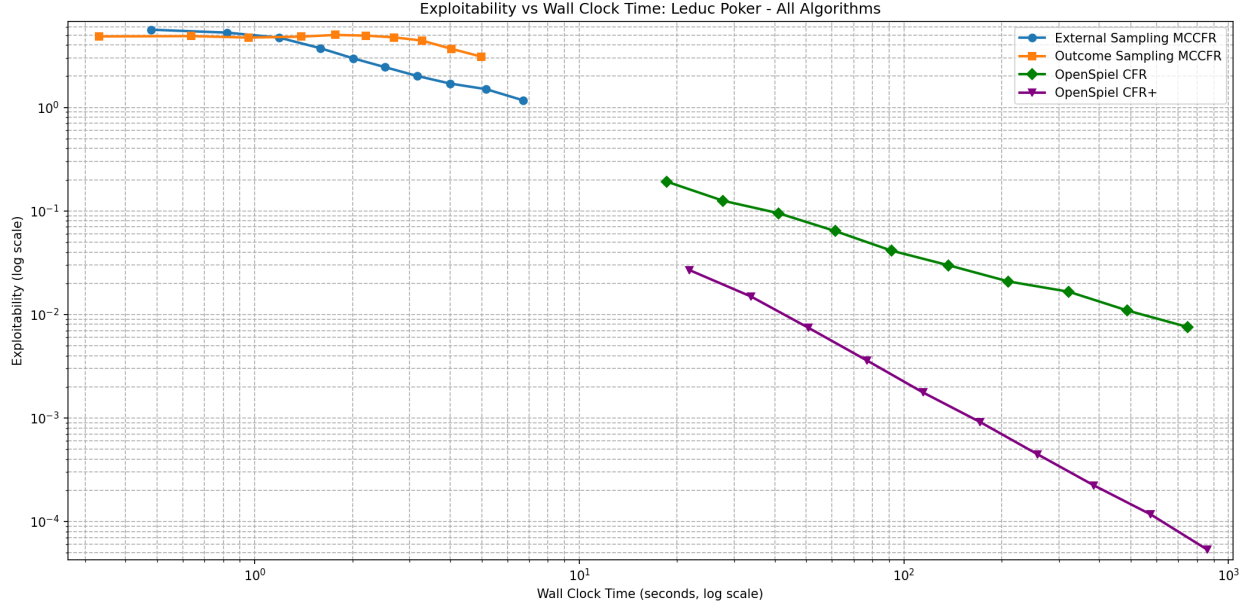
Figure 10: Leduc — Exploitability vs Wall-Clock Time
