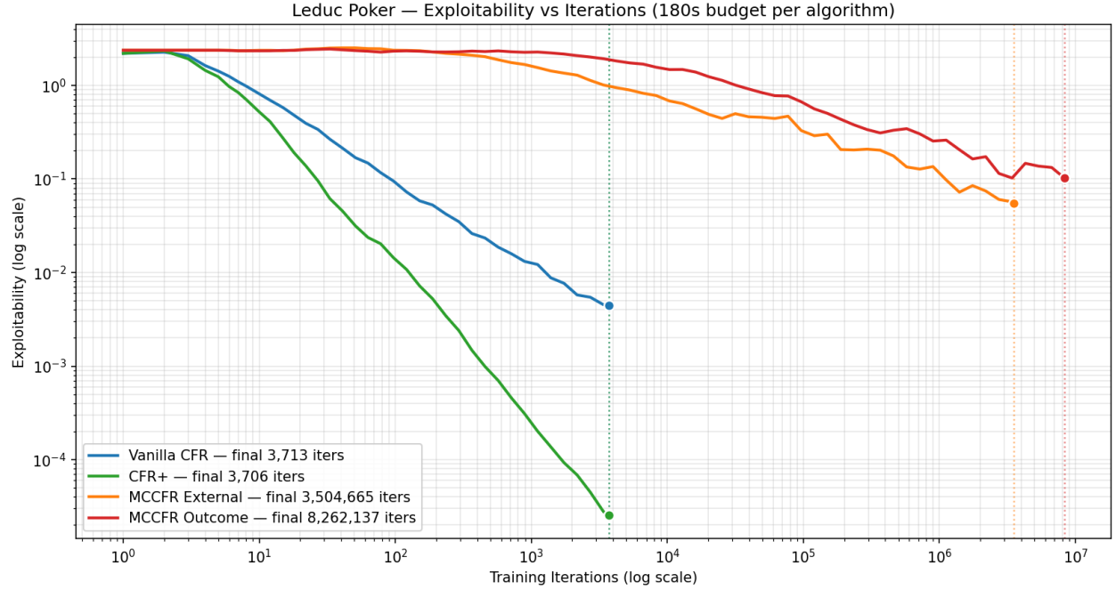
Figure 11: Exploitability vs Iterations (log-log)
