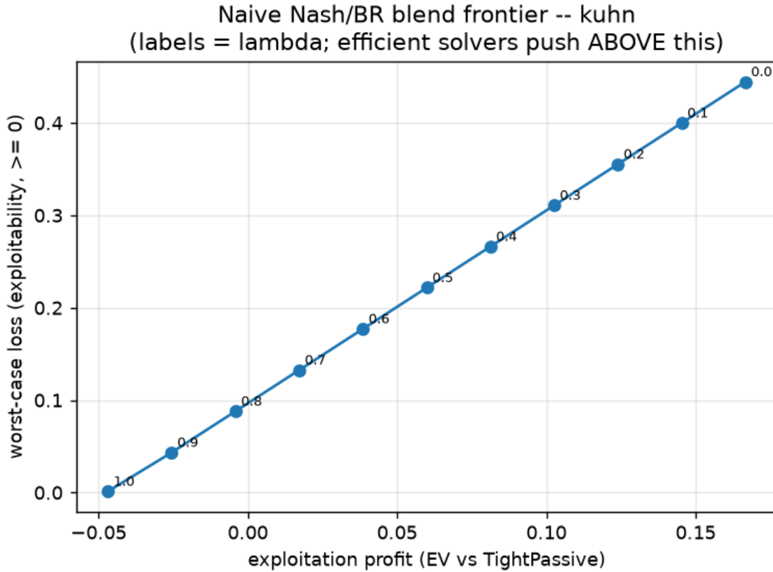
Figure 27: The naive Nash/best-response blend traces a smooth exploitation-safety frontier on Kuhn: every step toward more profit buys a near-proportional increase in your own worst-case loss.
