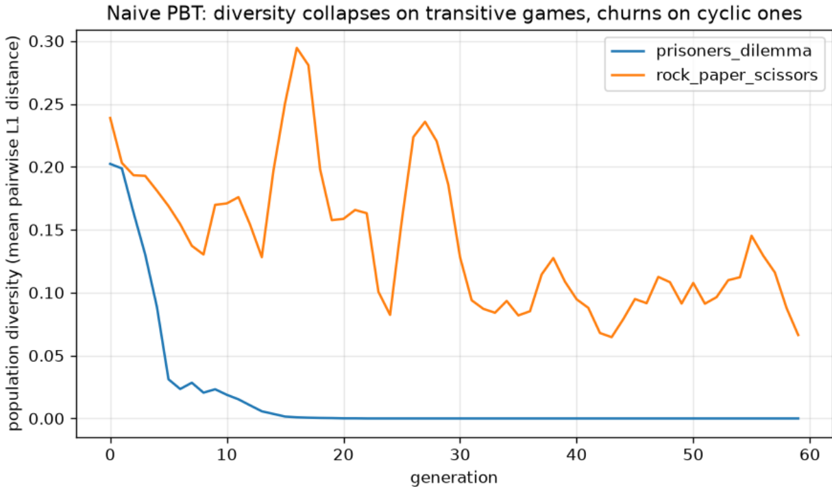
Figure 35: Mini-PBT diversity over generations: on the transitive Prisoner’s Dilemma the population’s strategy diversity collapses to zero (everyone converges to Defect), while on cyclic Rock-Paper-Scissors it churns indefinitely (0.07-0.29) as the population chases the wheel of counters. Game structure, not population size, sets whether diversity survives.
