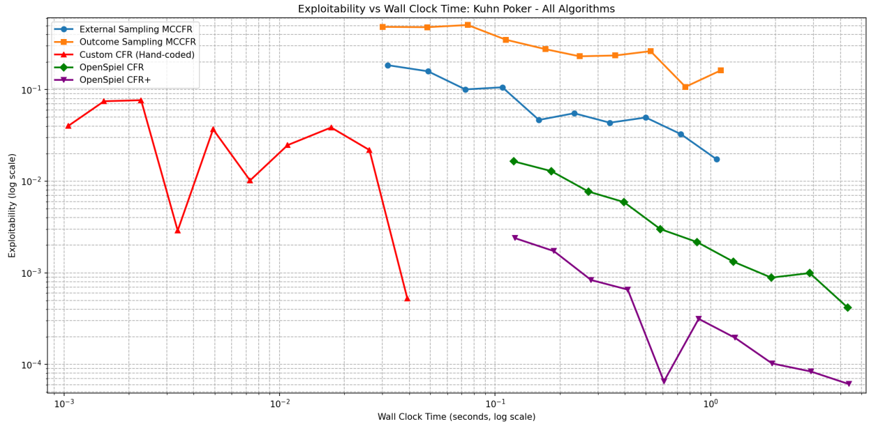
Figure 8: Kuhn — Exploitability vs Wall-Clock Time
