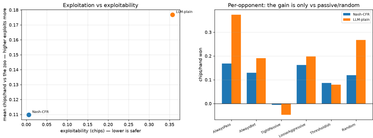
Figure 47: Exploitation against exploitability, and the per-opponent breakdown showing the gain is confined to passive and random opponents.
