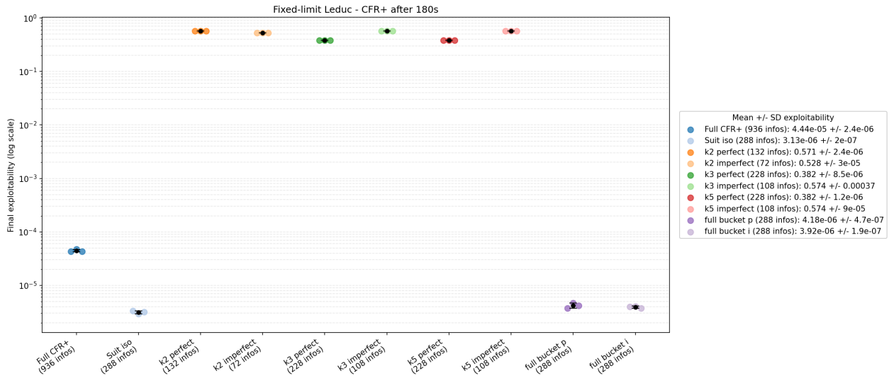
Figure 13: Fixed-limit Leduc CFR+ abstraction results
