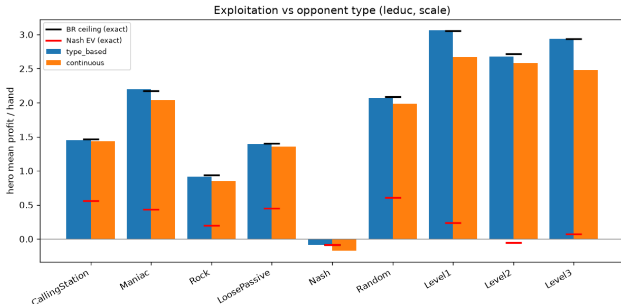
Figure 24: Exploitation vs opponent type (Leduc): type-based (blue) hugs the exact BR ceiling for every type; continuous (orange) tracks close but sits below for the hardest-to-fit types; both drop below zero against Nash.
