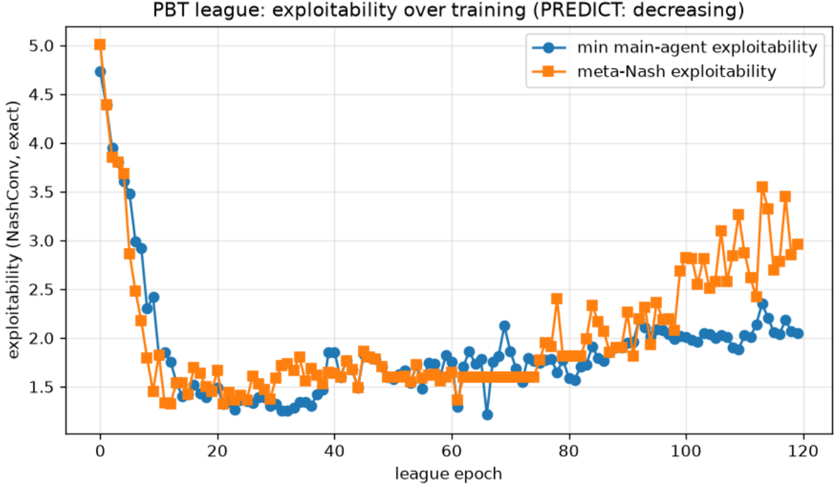
Figure 34: League exploitability over training (scale, 120 epochs): min-main and meta-Nash exploitability both fall steeply to a minimum near epoch 60 (min-main \sim 1.21 , meta-Nash \sim 1.32 ) and then regress upward ( \sim 2.05 / \sim 2.96 ) by epoch 119. A running league is not a monotonically improving one; the best agents are frozen snapshots from mid-run.
