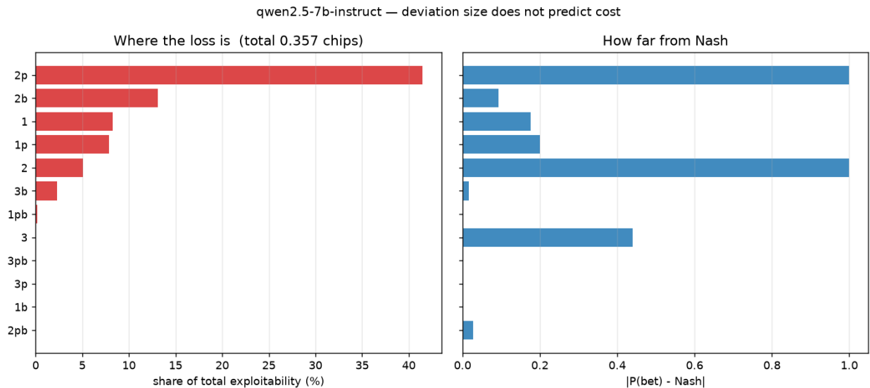
Figure 45: Each information set’s share of total exploitability, beside how far it deviates from Nash. The two orderings barely correspond.
