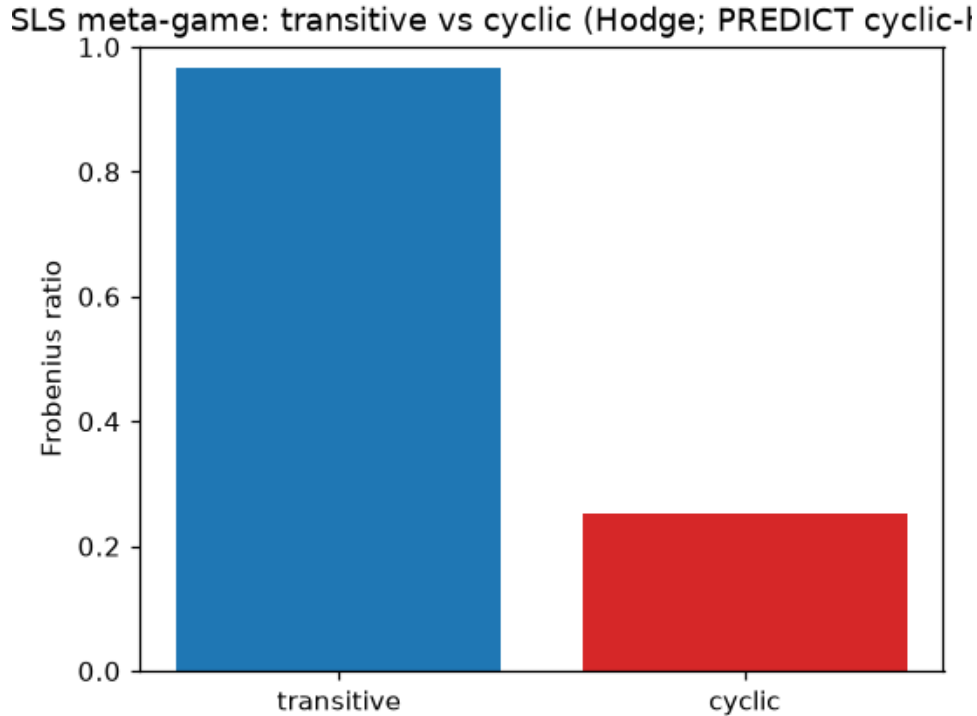
Figure 41: Spinning-top transitive/cyclic ratios across SLS populations: the skill-ladder baseline pool is transitive-dominant (cyclic \sim 0.25 - 0.31 ), while the coalition pool (fixed-ally + betrayer strategies) is strongly cyclic ( \sim 0.57 - 0.69 ). Coalition play injects large non-transitivity, confirming the direction of the Step-10 prediction, though it stays just under strict cyclic dominance.
