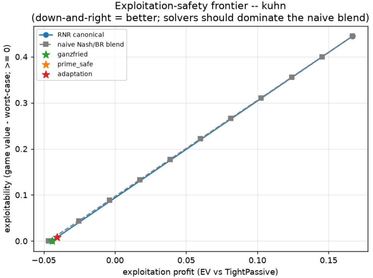
Figure 30: Exploitation-safety frontier (Kuhn). The canonical RNR “curve” is an interpolation between just two achieved clusters (safe corner and full-BR corner); the naive blend traces the smooth line; the LP operating points (stars) sit at the efficient safe corner.
