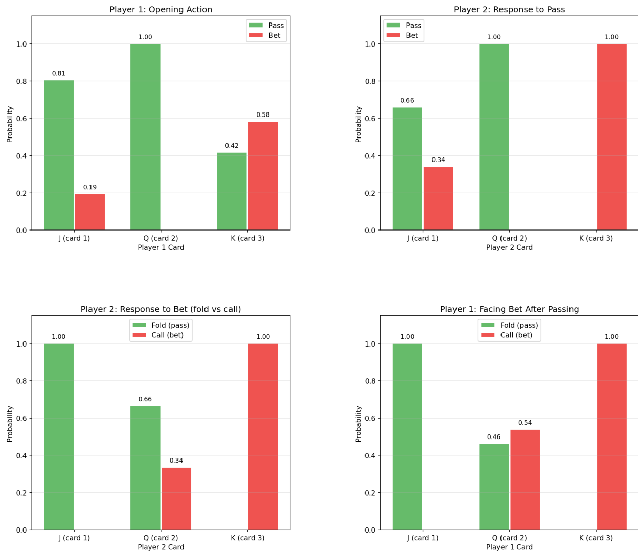
Figure 6: Strategy Analysis
