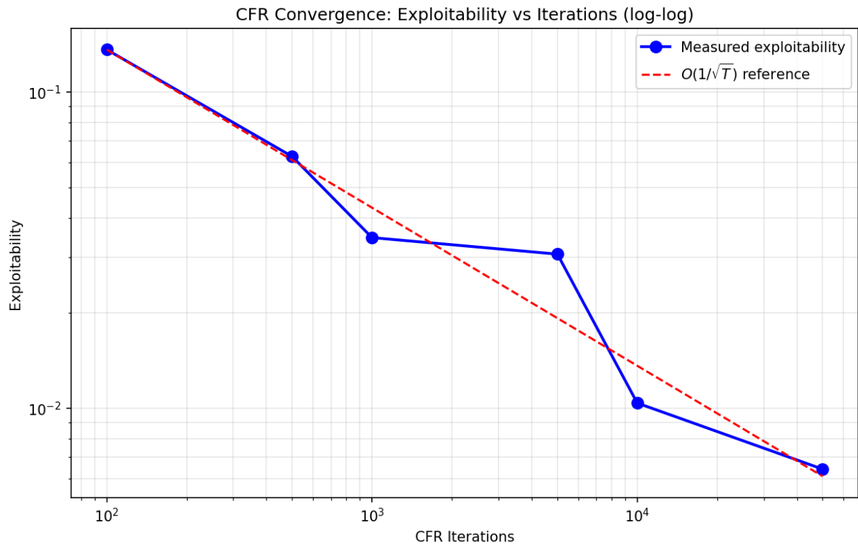
Figure 5: Exploitability Convergence
