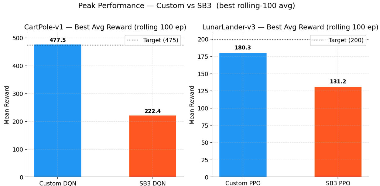
Figure 3: Peak Performance
