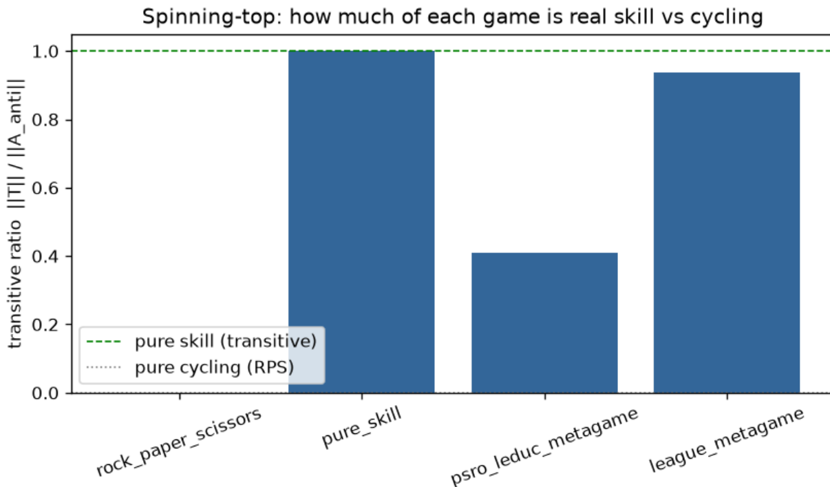
Figure 33: Transitive-ratio bar chart: Rock-Paper-Scissors (0.0, purely cyclic), a pure skill ladder (1.0, purely transitive), the PSRO-Leduc best-response meta-game ( \sim 0.41 - 0.46 , mostly cyclic with 27 three-cycles), and the league snapshot meta-game ( \sim 0.94 - 0.98 , mostly transitive). Which population you decompose decides whether Leduc looks like a wheel or a ladder.
