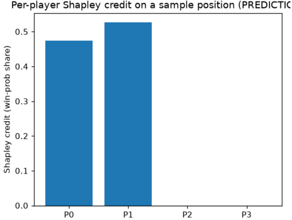
Figure 39: Shapley credit attribution on SLS positions: per-player Shapley value of the win-probability characteristic function. In the symmetric position credit is near-flat across the four seats (spread 0.013, post-fix); in the asymmetric [8,8,1,1] position the strong pair absorbs all credit (1.0) and the weak pair gets 0.0. Credit assignment tracks real contribution once the engine tie-break is unbiased.
