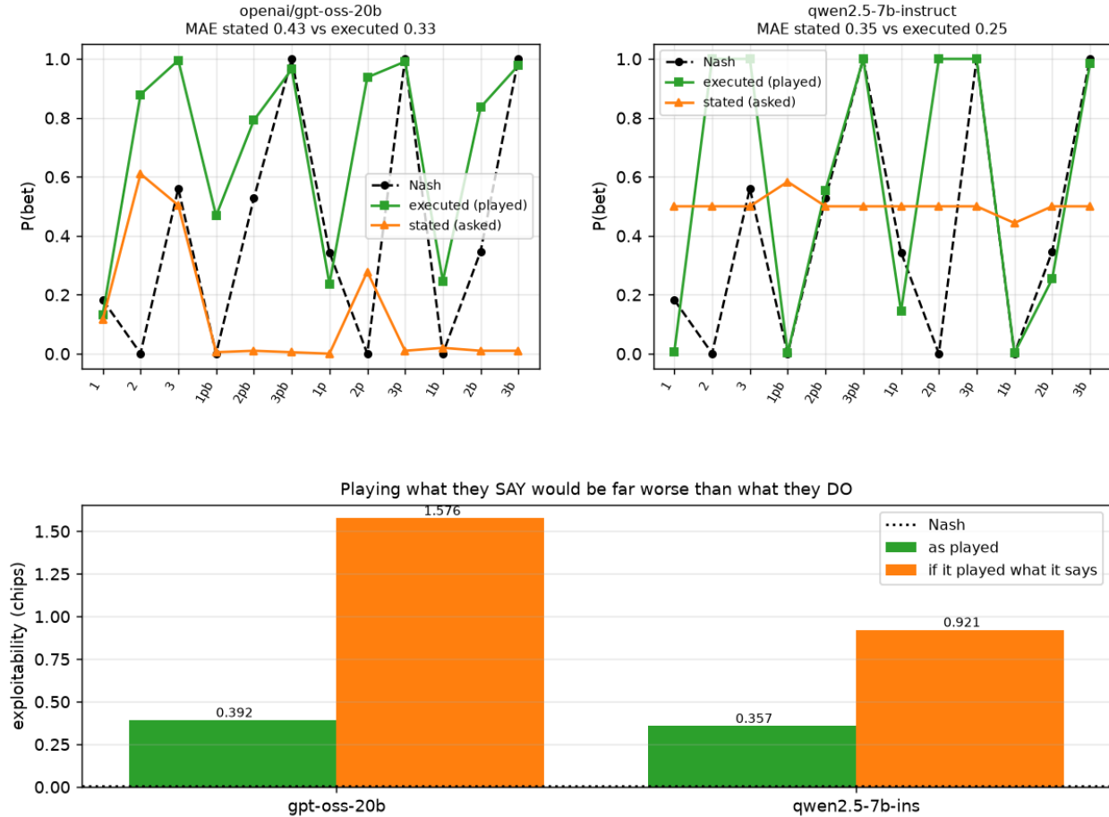
Figure 46: Stated versus executed betting frequency at each information set for both models, with Nash for reference, and the exploitability of each model's played strategy against a strategy built from its own stated frequencies.
