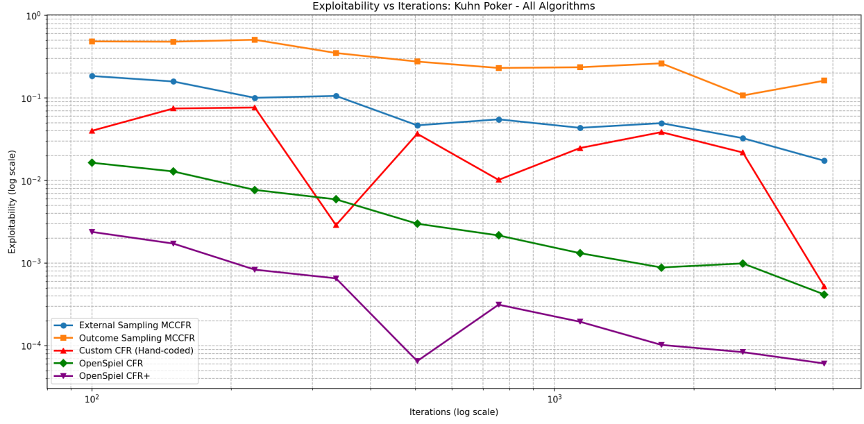
Figure 7: Kuhn — Exploitability vs Iterations
