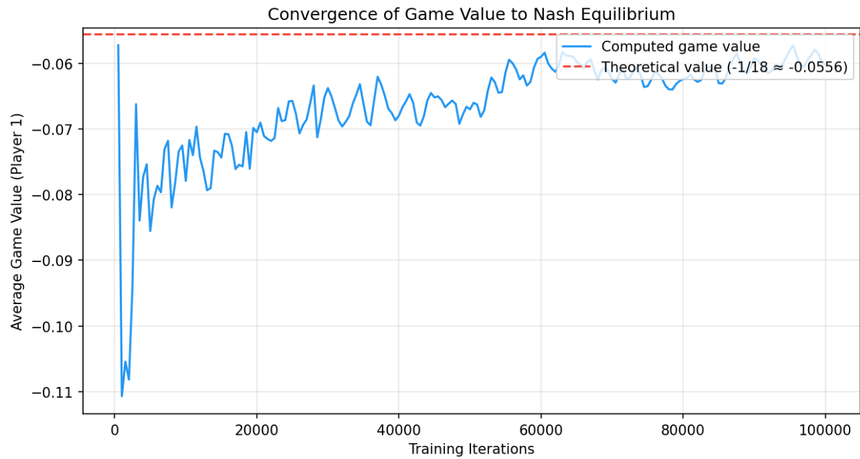
Figure 4: Game Value Convergence
