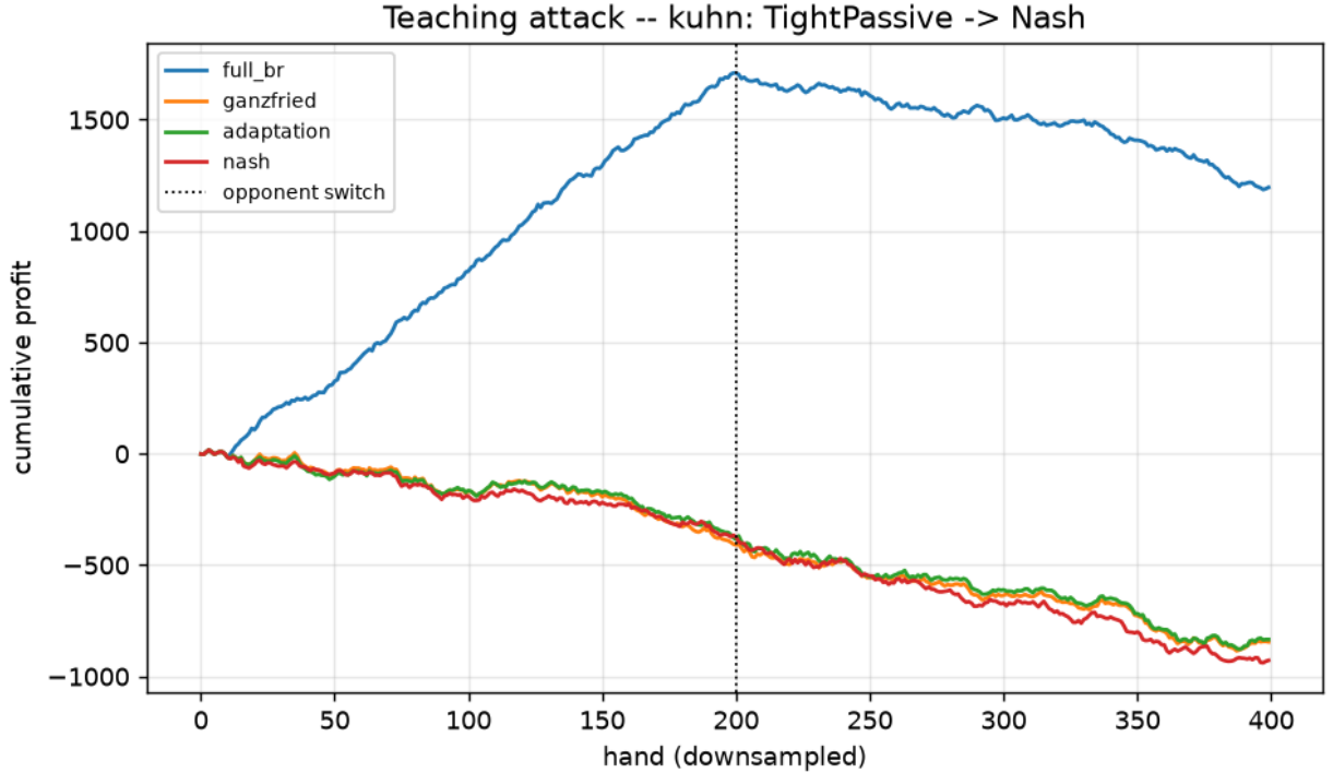
Figure 31: Teaching attack (Kuhn), cumulative profit. full_br (blue) climbs on the bait to \approx +1700 , then only drifts down after the switch — it ends far ahead because a Nash “revealer” claws back only \approx the game value per hand. The safe methods refuse the bait and pay the P0 tax throughout.
