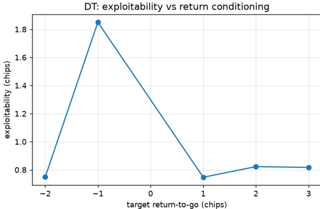
Figure 43: DT exploitability against the conditioned target return, including an impossible +3. The curve is flat across the real range with a sharp collapse at R = -1 , the modal payoff and the payoff of folding.
