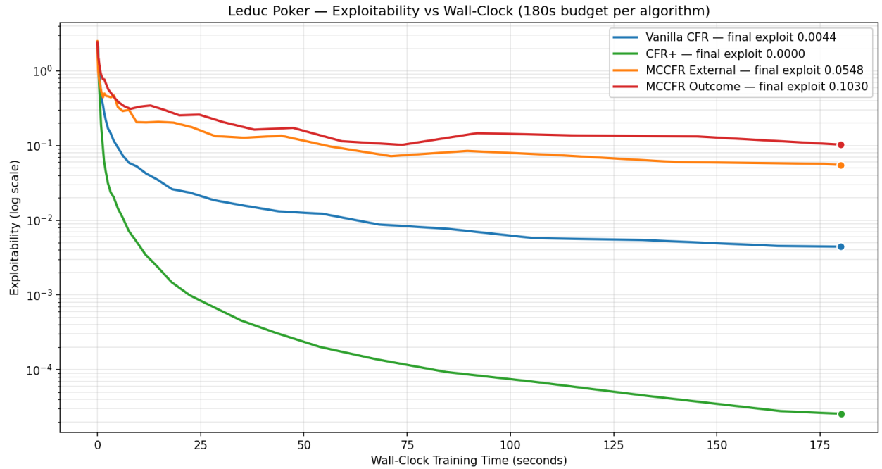
Figure 12: Exploitability vs Wall-Clock Time (log-y)
