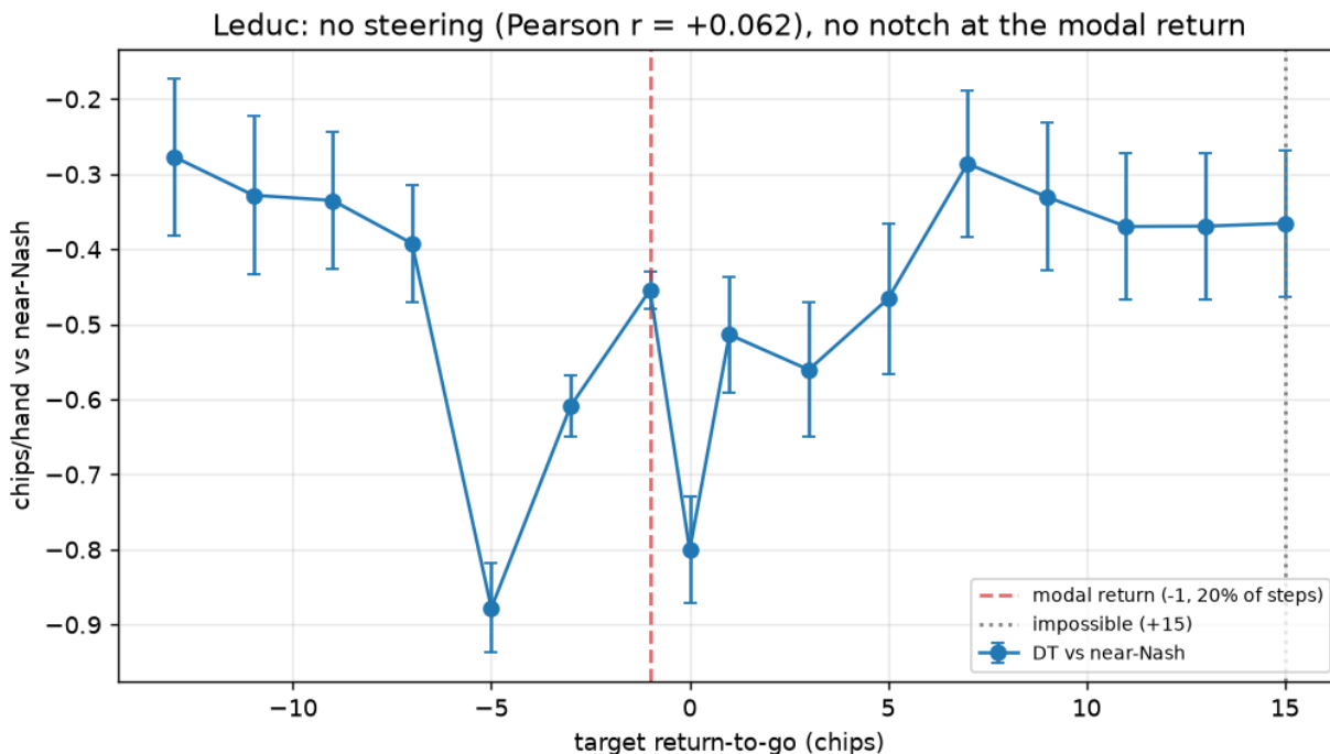
Figure 48: DT performance against the conditioned target return on Leduc, with standard errors. There is no collapse at the modal return and no monotone trend.
