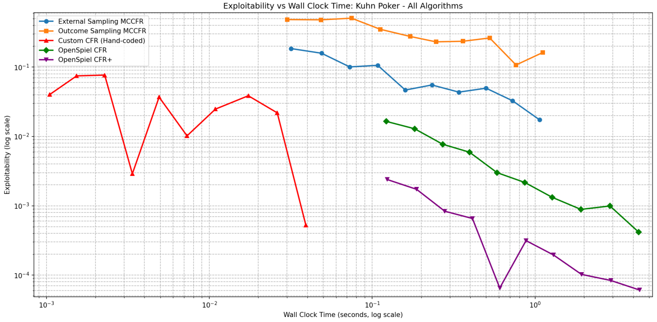
Figure 9: Kuhn Poker — Exploitability vs Wall-Clock Time
