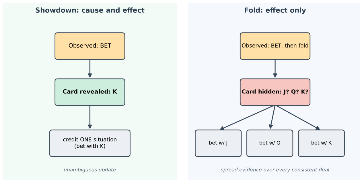
Figure 33: Partial observability: a showdown reveals the opponent’s private card, pinning the action to one situation; a fold hides it, forcing the model to spread the evidence across every hand the opponent might have held.
