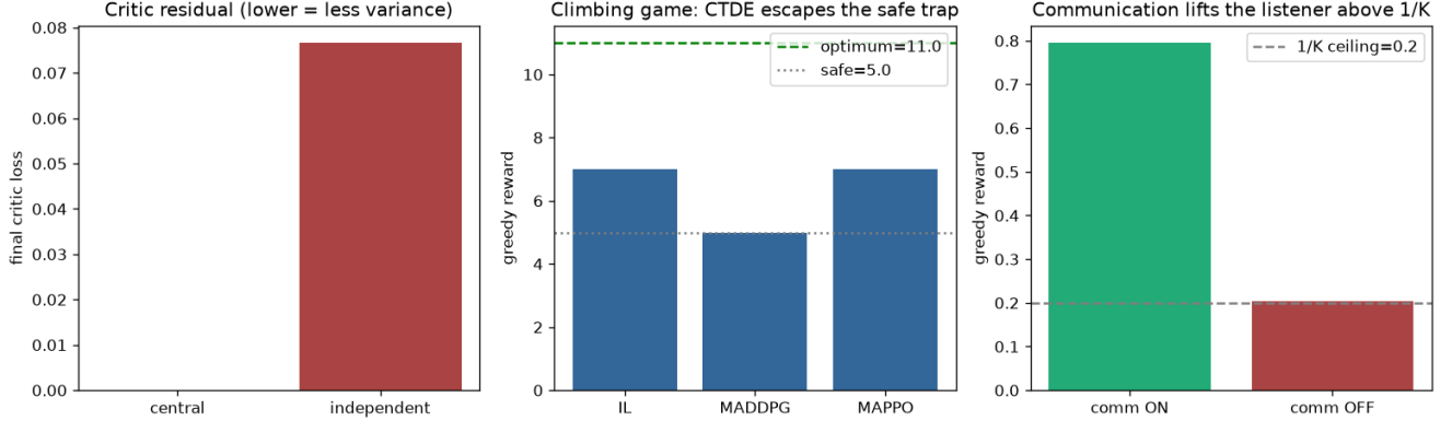
Figure 50: Cooperative CTDE and communication results (scale config). Left: the centralized critic’s residual is orders of magnitude below the independent critic’s. Middle: on the climbing game, no method reaches the optimum (11); MADDPG (5) trails IL and MAPPO (7) — CTDE reduces critic variance but does not by itself solve hard-exploration coordination. Right: communication lifts the listener far above the 1/K guessing ceiling (see §7).
