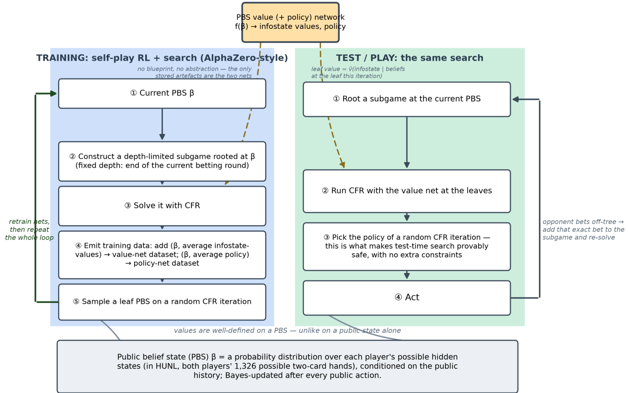
Figure 27: ReBeL’s AlphaZero-style loop: self-play training (left) and test-time play (right) share one PBS value/policy network, both solving depth-limited subgames rooted at the public belief state (shared definition box, bottom).
