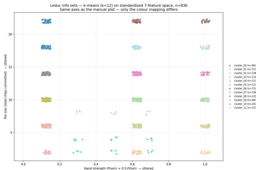
Figure 12: Infoset grouping via K-means
