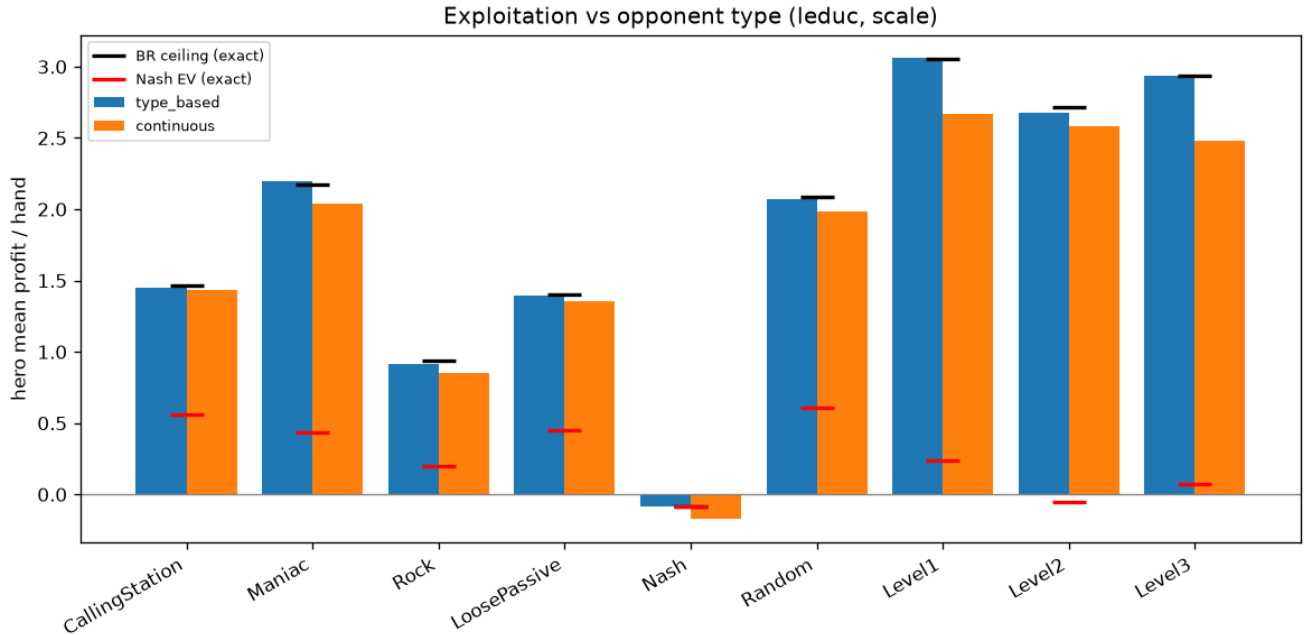
Figure 36: Exploitation against each Leduc opponent: the type-based model (which fits these opponents) hugs the exact best-response ceiling, while the continuous model tracks close but sits below for the hardest-to-fit types — and dips below the safe baseline against Nash.
