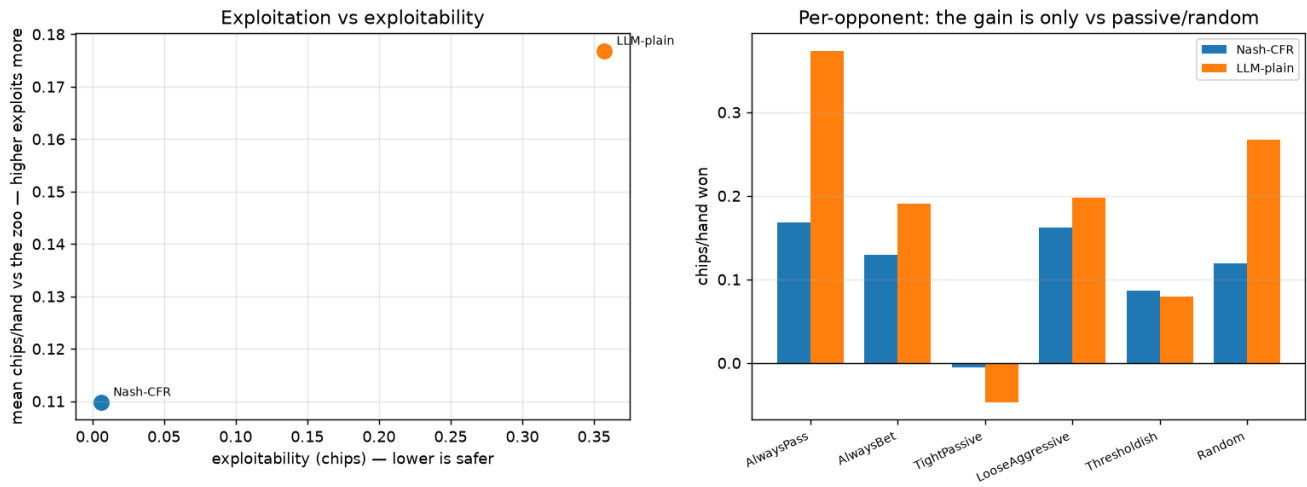
Figure 76: Exploitation against exploitability, with the per-opponent breakdown.
