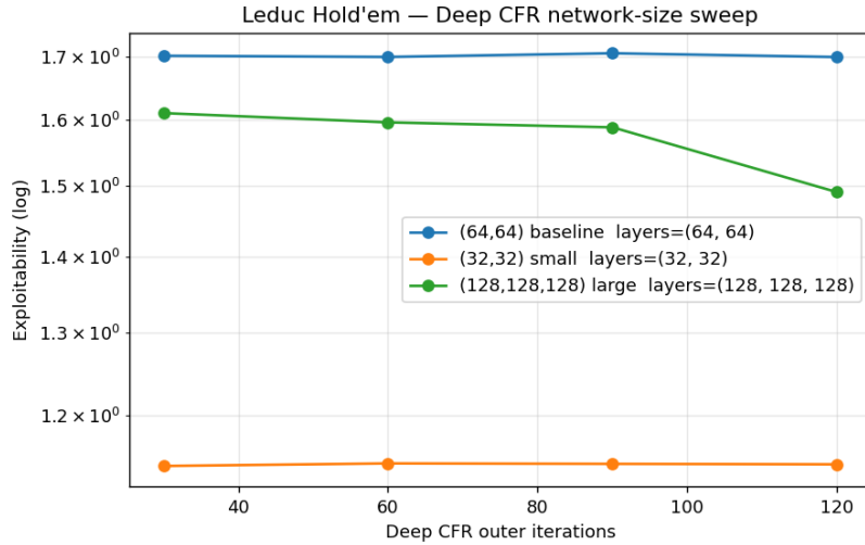
Figure 19: Deep CFR exploitability on Leduc across network sizes (32x32, 64x64, 128x128x128).
