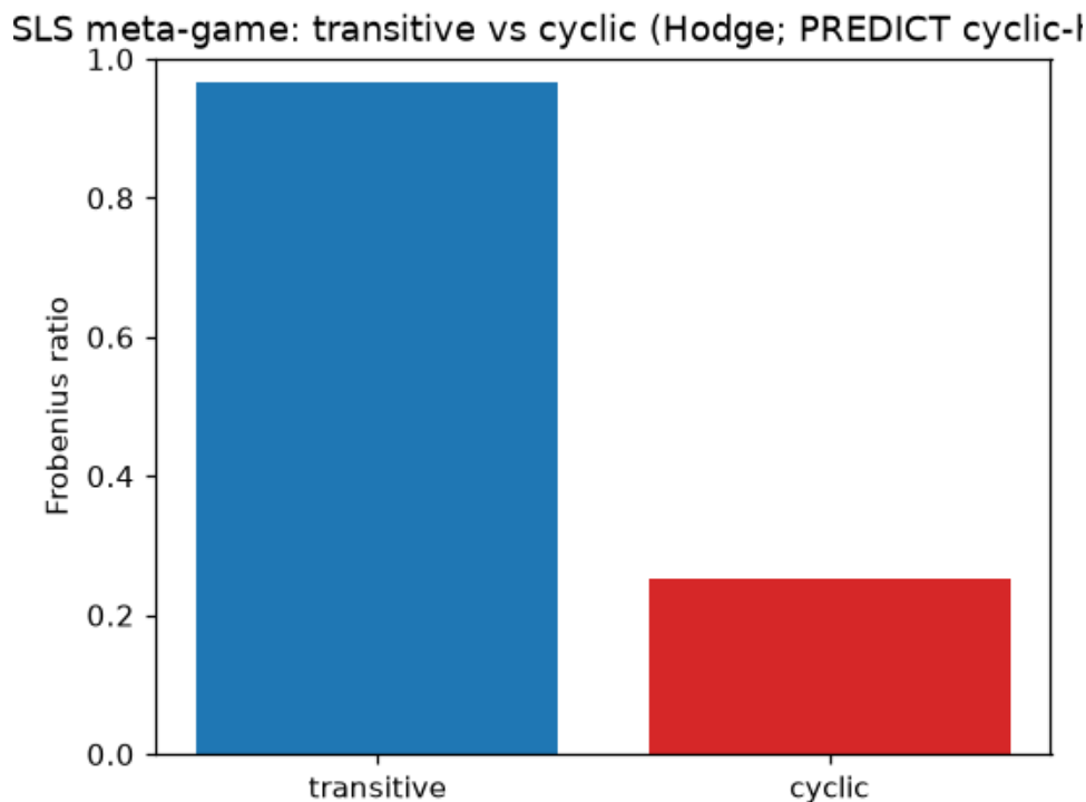
Figure 71: Spinning-top transitive/cyclic ratios: the skill-ladder pool is transitive-dominant (cyclic \sim 0.25 - 0.31 ), while the coalition pool is strongly cyclic ( \sim 0.57 - 0.69 ). Coalition play injects large non-transitivity, confirming the Step-10 direction while staying just under strict cyclic dominance.
