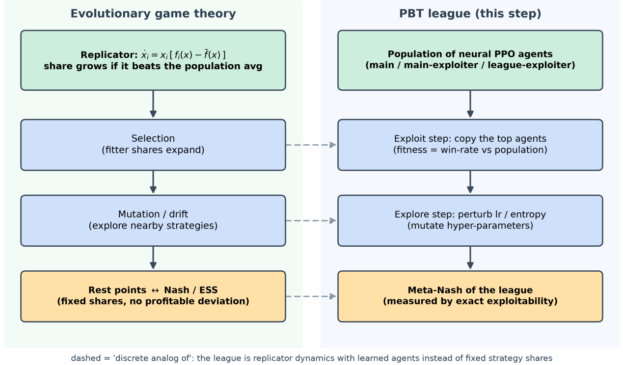
Figure 55: Evolutionary game theory as the continuous idealization of a PBT league: replicator selection \leftrightarrow copying the fitter agents, mutation/drift \leftrightarrow perturbing learning rate and entropy, and replicator rest points \leftrightarrow the meta-Nash / ESS the league is trying to reach. The league is replicator dynamics with learned agents instead of fixed strategy shares.
