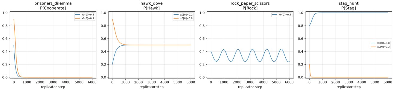
Figure 56: Replicator phase portraits: Prisoner’s Dilemma → all-Defect, Hawk-Dove → the 0.5 interior ESS, Rock-Paper-Scissors → a closed orbit that never converges, and Stag Hunt → two basins (all-Stag or all-Hare). The non-converging RPS orbit is why populations in cyclic games need explicit machinery to avoid spinning.
