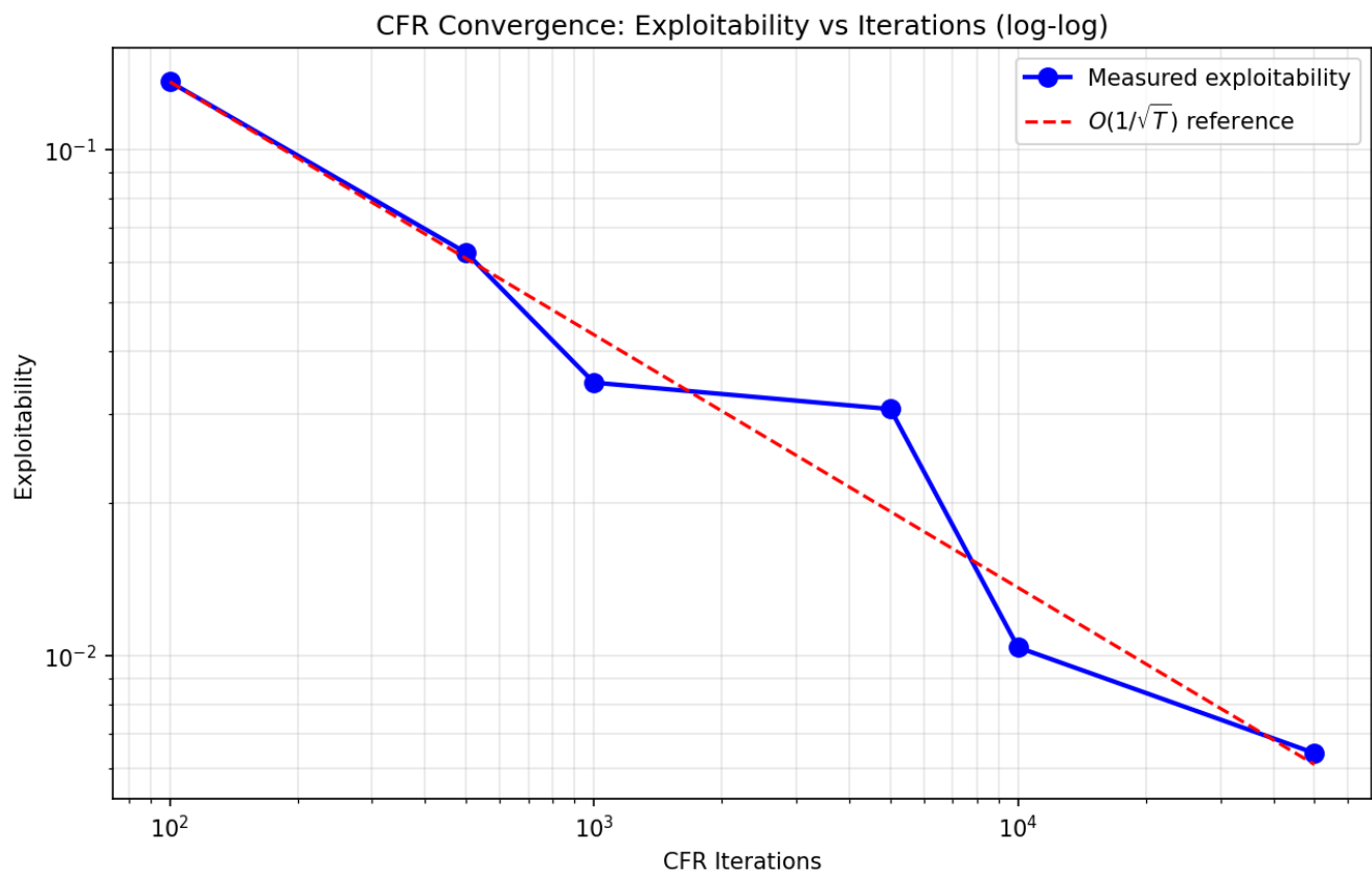
Figure 4: Exploitability Convergence
