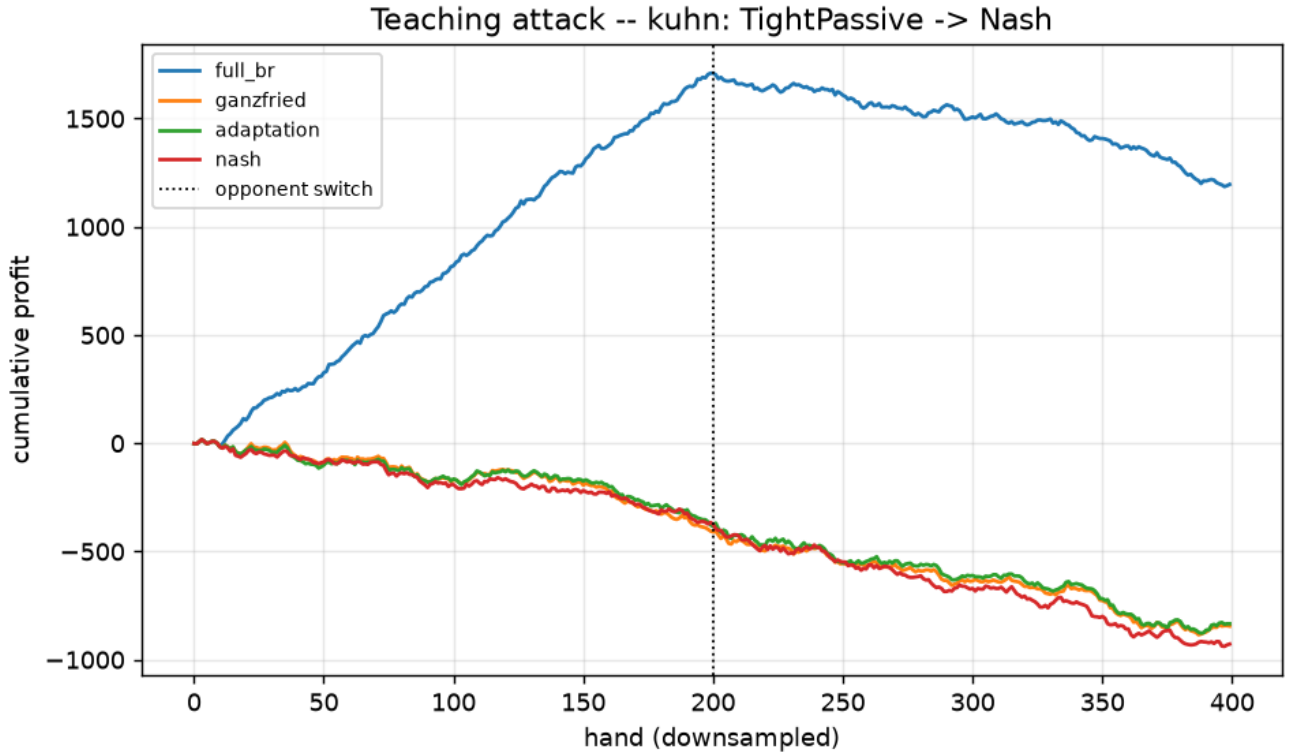
Figure 44: Teaching attack on Kuhn, cumulative profit. The full best response (blue) climbs on the bait to about +1700, then only drifts down after the switch — it ends far ahead, because a Nash “revealer” claws back only about the game value per hand. The safe methods refuse the bait and pay the first-player tax throughout.
