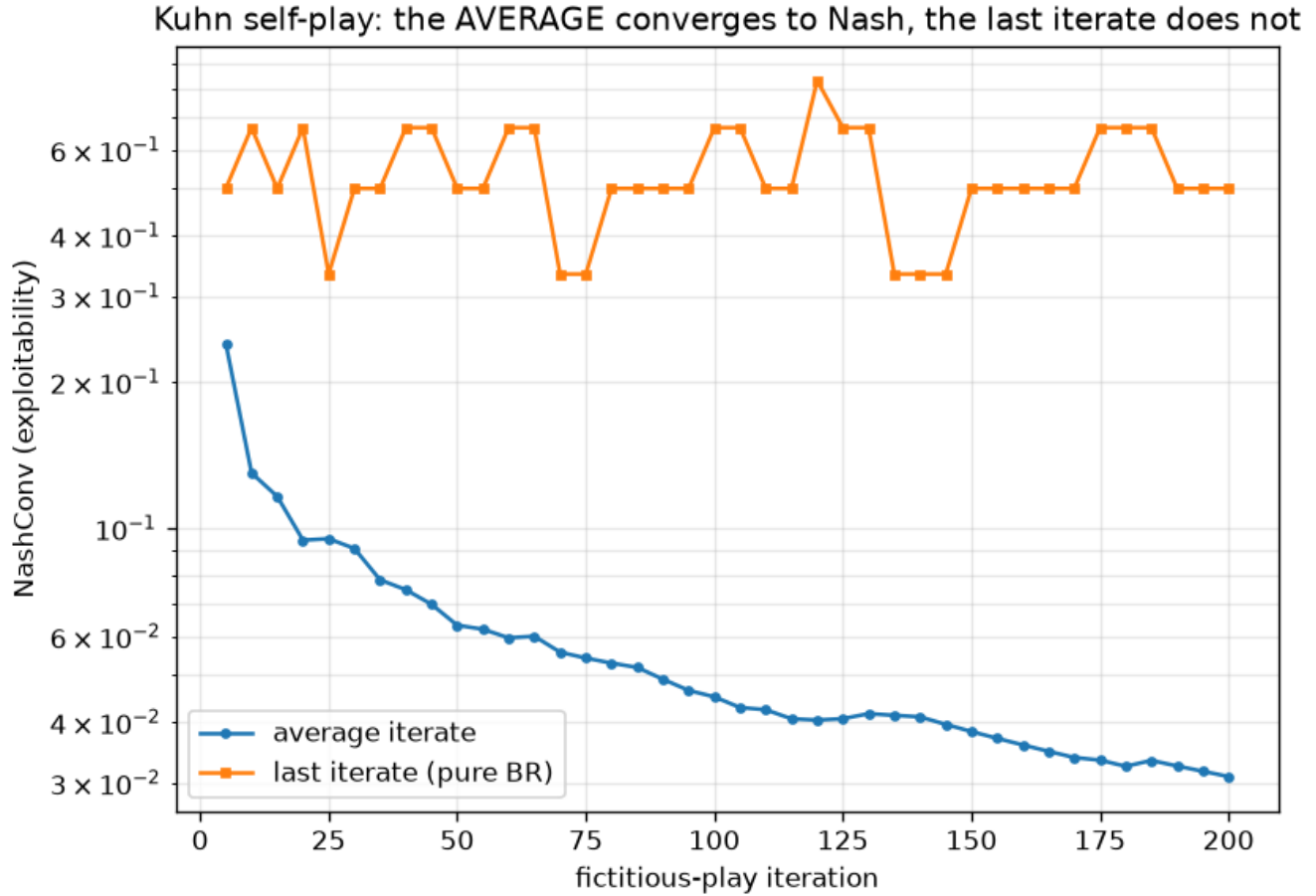
Figure 53: Self-play on Kuhn: the average-iterate exploitability (NashConv) falls steadily toward zero while the last-iterate exploitability keeps oscillating. This is why self-play and PSRO rely on averaging over a population rather than trusting the most recent policy.
