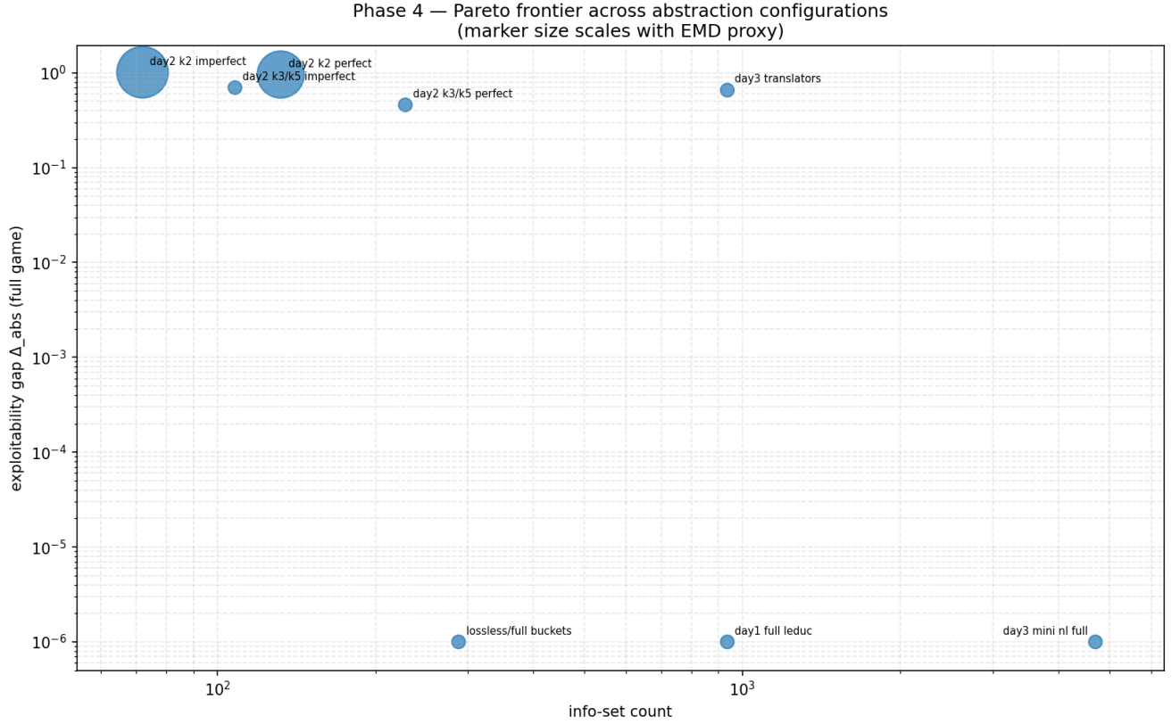
Figure 16: Abstraction Pareto frontier
