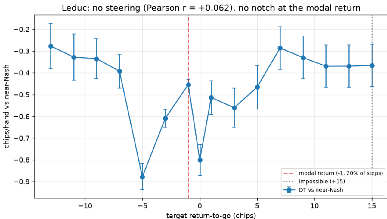
Figure 73: Decision Transformer performance against the conditioned target return on Leduc Hold’em, with standard errors.
