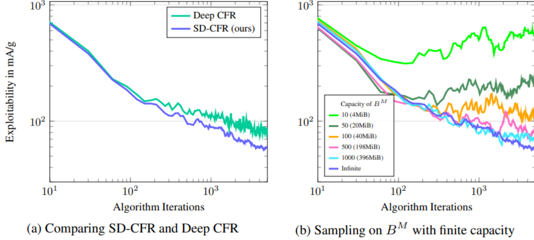
Figure 21: Single Deep CFR (SD-CFR) matches or slightly beats Deep CFR while training only one network (left); the right panel shows how reservoir-buffer capacity affects convergence. From the Single Deep CFR paper — not an experiment from this work.
