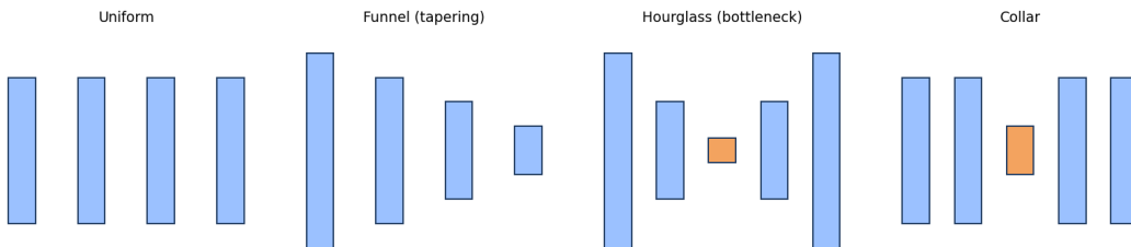
Figure 20: Common network shapes: a uniform stack, a tapering funnel, an hourglass with a central bottleneck (orange), and a uniform stack with a single narrow collar (orange). Bar height represents layer width.
