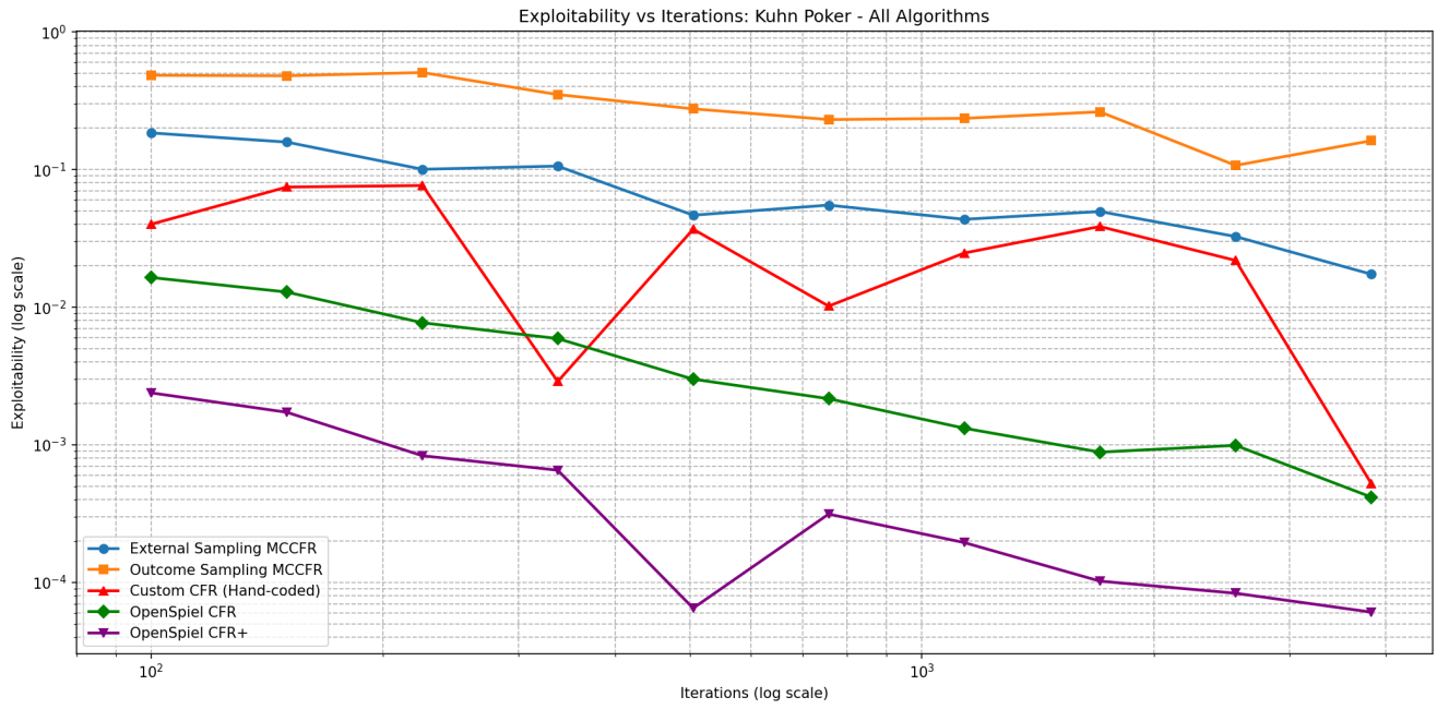
Figure 8: Kuhn Poker — Exploitability vs Iterations
