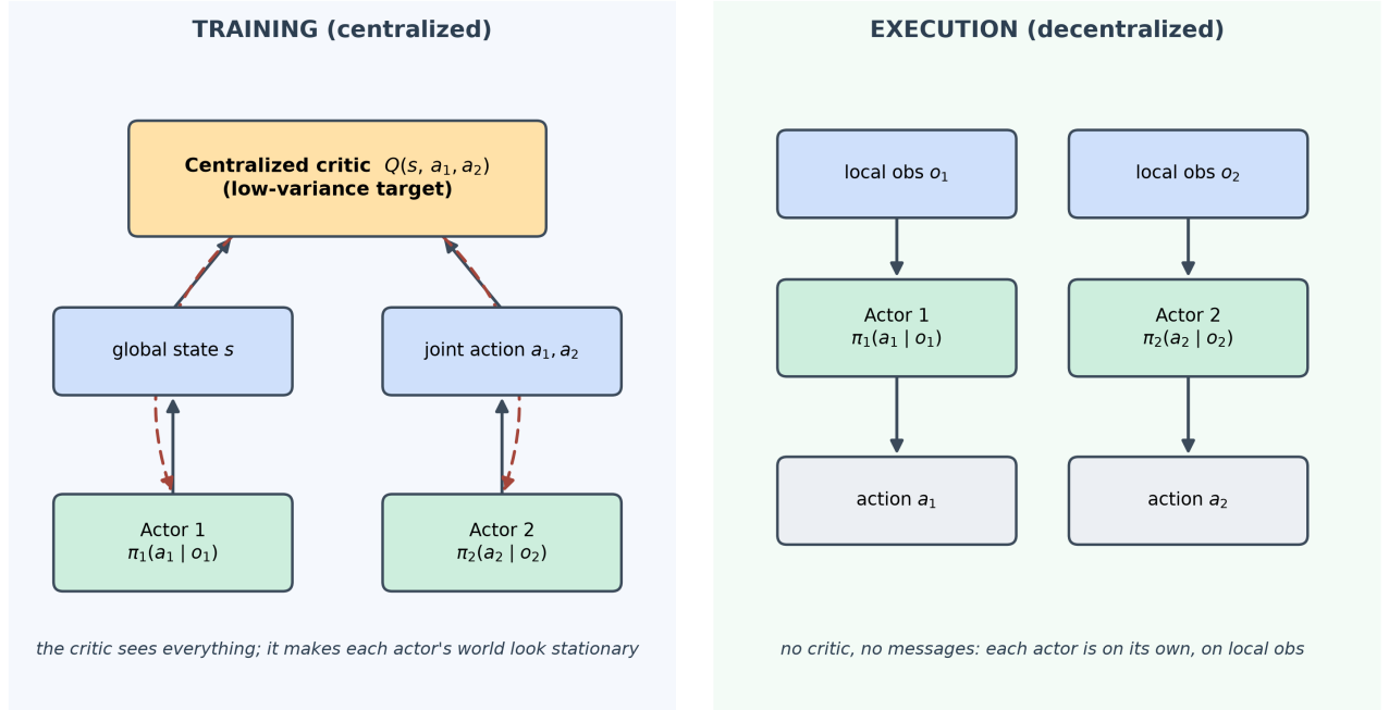
Figure 49: CTDE architecture. During training a centralized critic (or value function) sees the global state and the joint action and produces low-variance value targets; during execution each actor acts on its own local observation with no access to the critic and no message passing. The training/execution asymmetry is what makes the world look stationary to the learner without cheating at showtime.
