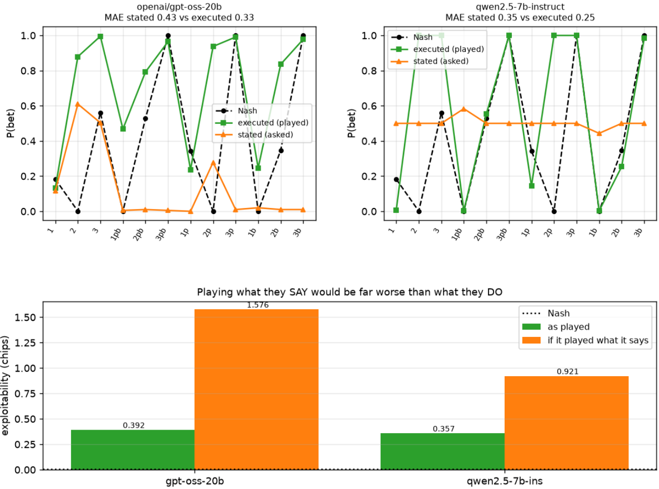
Figure 75: Stated versus executed betting frequencies for two models, with the exploitability of each strategy.
