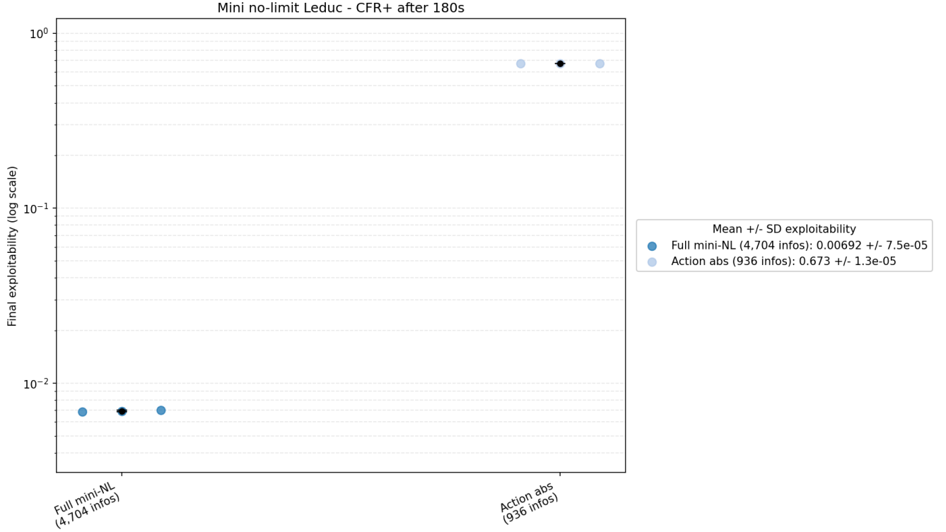
Figure 14: Mini-NL Leduc CFR+ abstraction results
