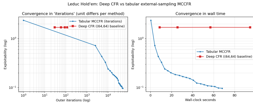
Figure 22: Deep CFR vs. tabular MCCFR exploitability on Leduc.
