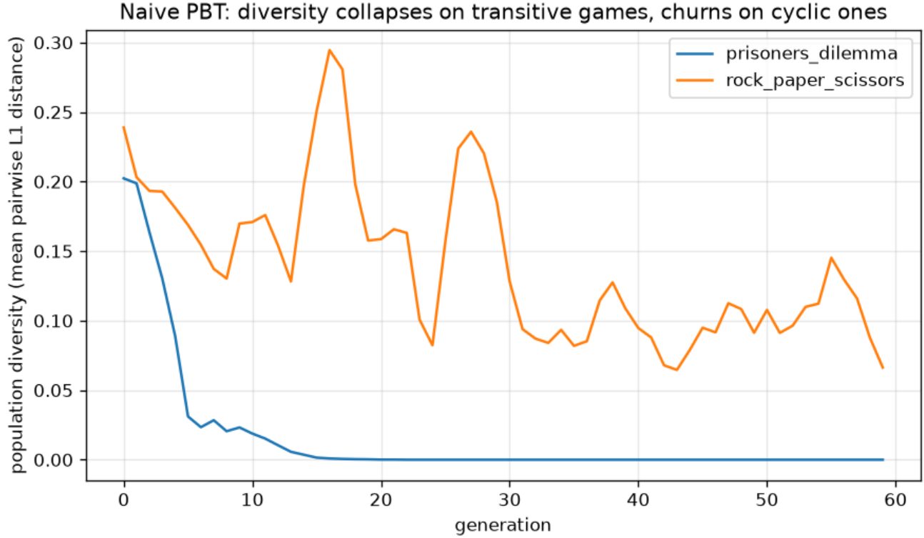
Figure 61: Mini-PBT diversity: on the transitive Prisoner’s Dilemma the population collapses to a single strategy (diversity \rightarrow 0), while on cyclic Rock-Paper-Scissors it churns indefinitely (0.07-0.29) as it chases the wheel of counters. Game structure, not population size, decides whether diversity survives.
