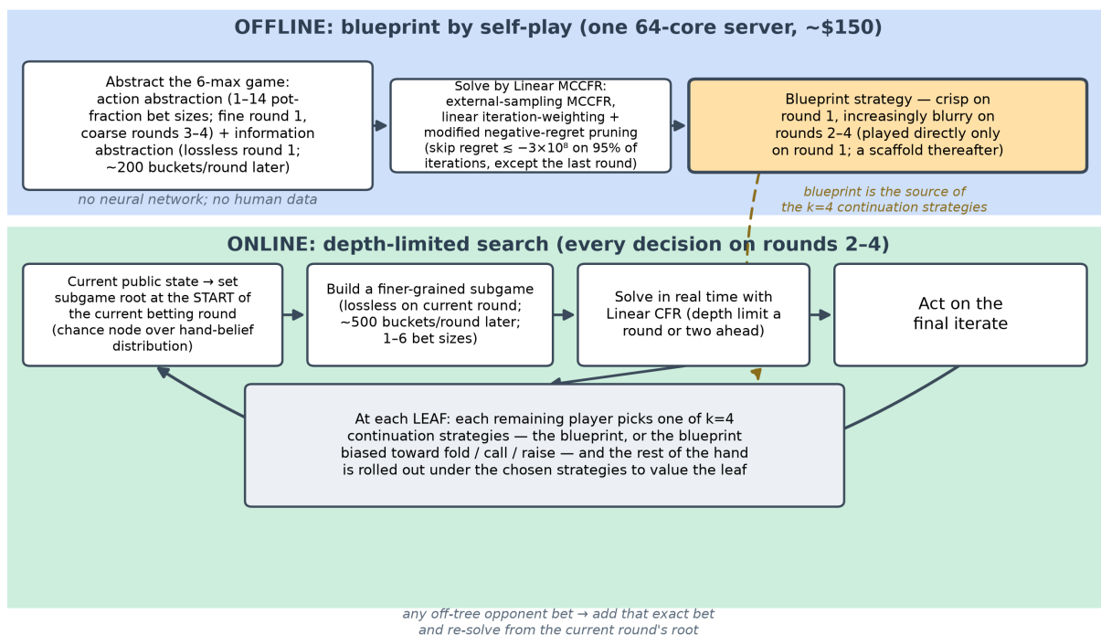
Figure 26: Pluribus’s two-phase architecture: an offline Linear-MCCFR blueprint (top) reused as the source of k=4 continuation strategies inside the online depth-limited search (bottom).
