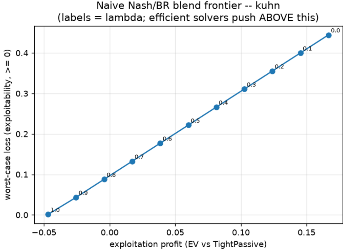
Figure 40: The naive Nash/best-response blend on Kuhn: a smooth exploitation-safety frontier where each increment of profit costs a near-proportional increment of your own worst-case loss.
