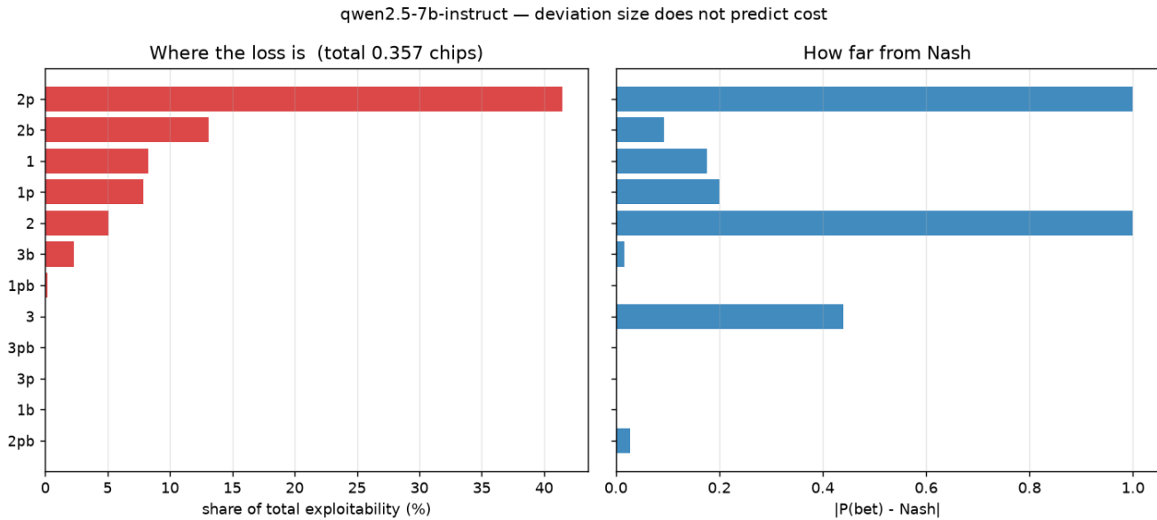
Figure 74: Each information set’s share of total exploitability, beside its deviation from equilibrium.
