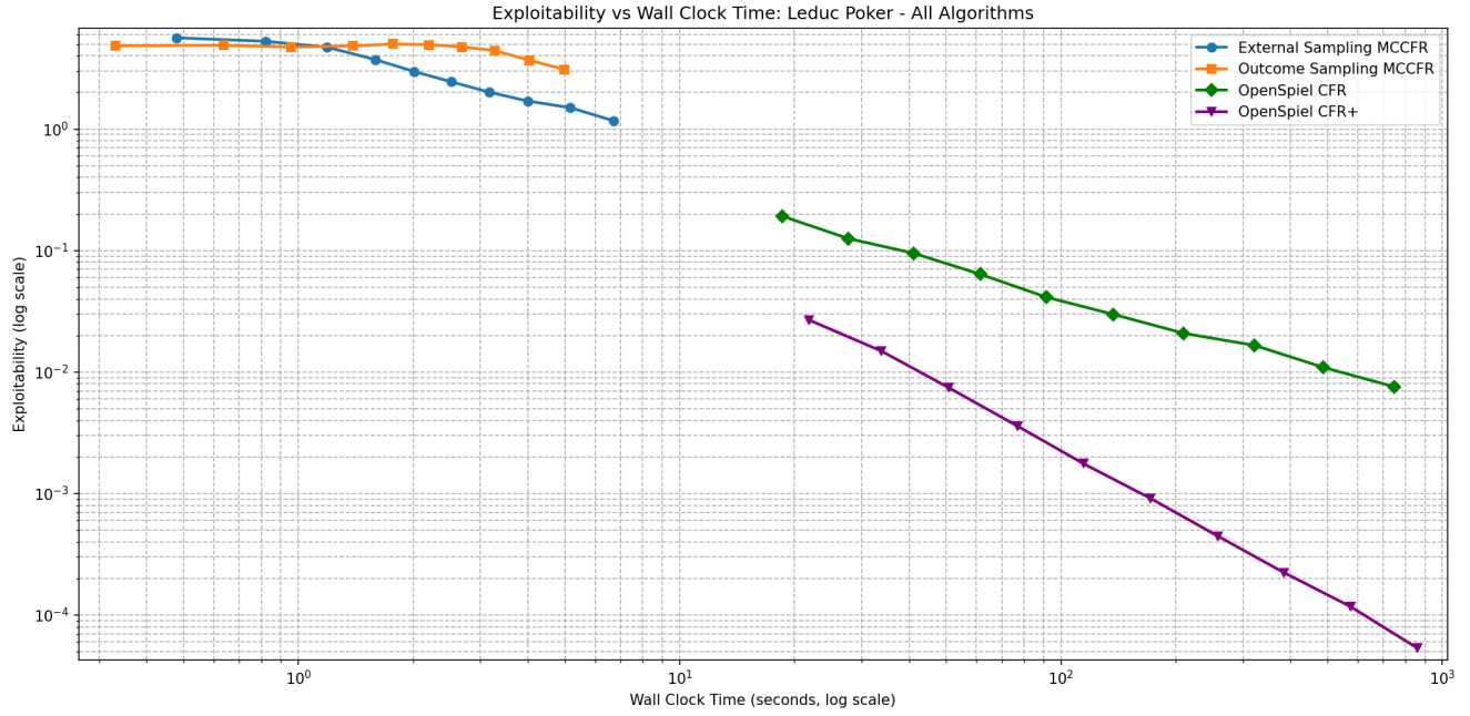
Figure 7: Leduc Poker — Exploitability vs Wall-Clock Time
