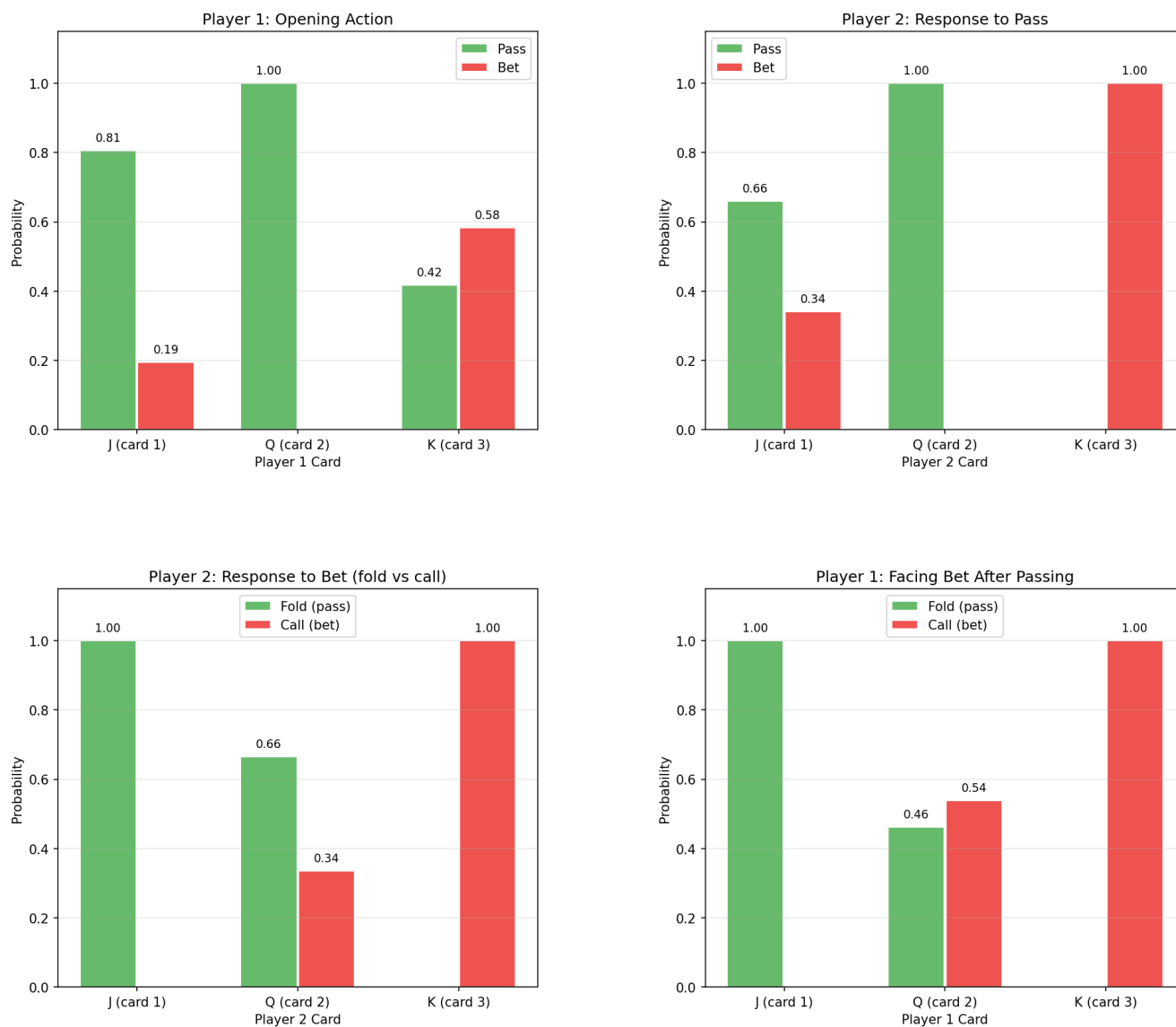
Figure 5: Strategy Analysis
