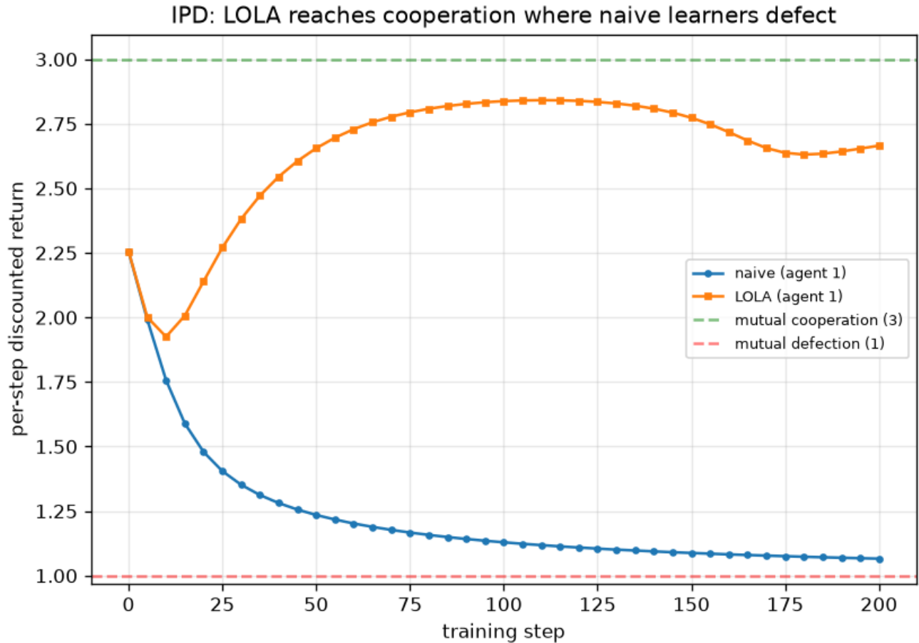
Figure 54: LOLA vs naive learners on the Iterated Prisoner’s Dilemma: naive learners’ per-step return collapses toward mutual defection ( \sim 1 ), while LOLA learners’ return climbs toward mutual cooperation ( \sim 2.8 ). Anticipating the opponent’s next learning step is what reshapes the dynamics from defection to cooperation.
