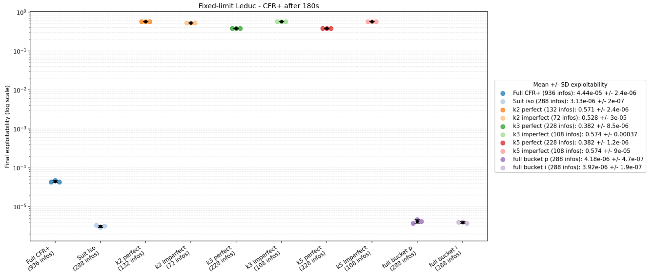
Figure 13: Fixed-limit Leduc CFR+ abstraction results
