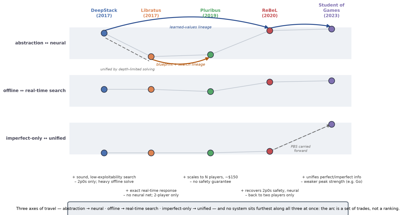
Figure 29: The seven-year arc as trade-offs: the five systems placed along three axes (abstraction \rightarrow neural; offline \rightarrow real-time search; imperfect-only \rightarrow unified), with lineage arrows and a per-system capability-gained/given-up tag.
