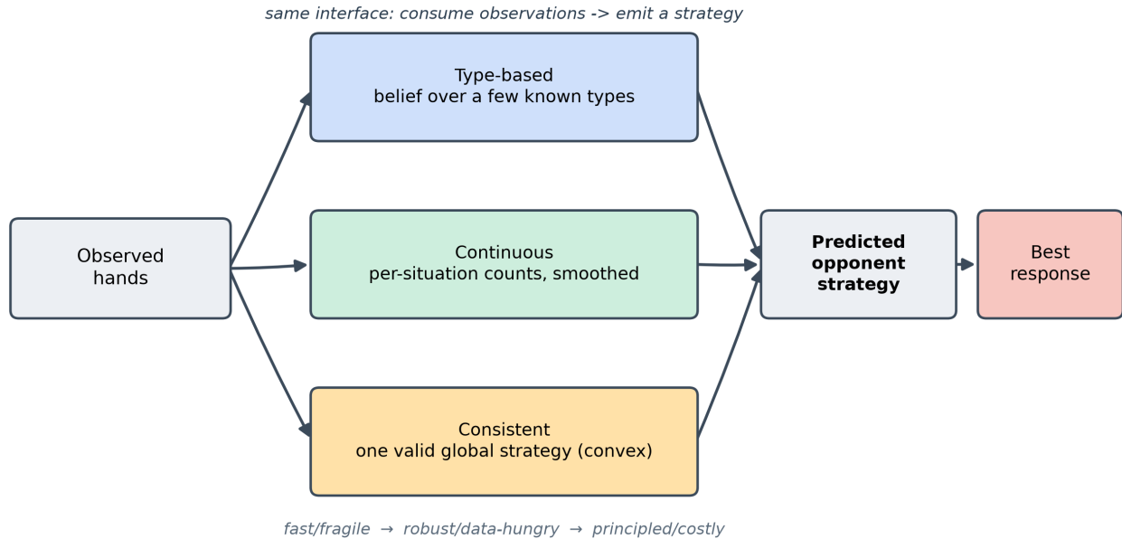
Figure 34: Three models on one interface: a discrete belief over types, a free-form per-situation count, and a globally-consistent sequence-form estimate — all emit a predicted opponent strategy consumed by the same best-response step.
