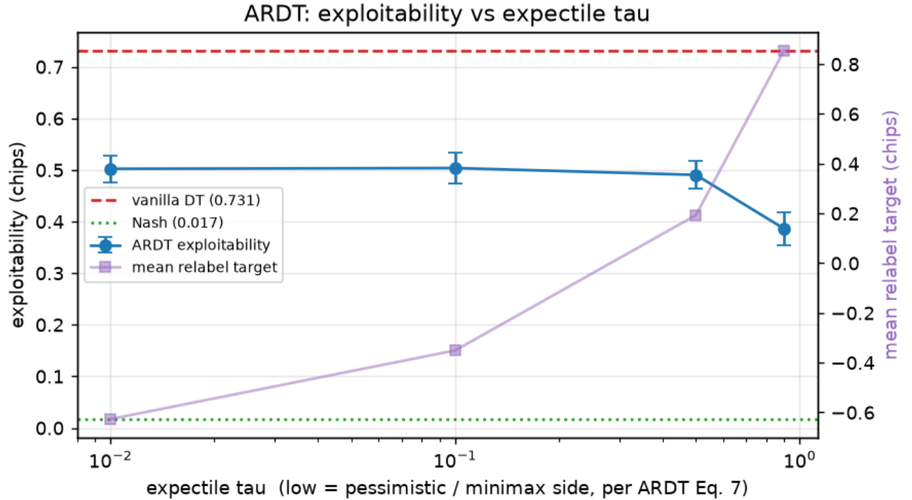
Figure 72: ARDT exploitability against the expectile tau, with the mean relabel target on the second axis.
