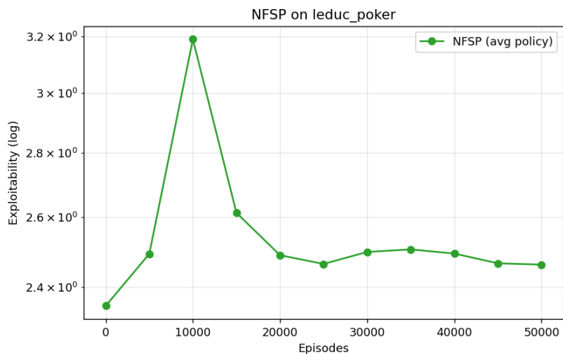
Figure 23: NFSP exploitability on Leduc over training episodes.
