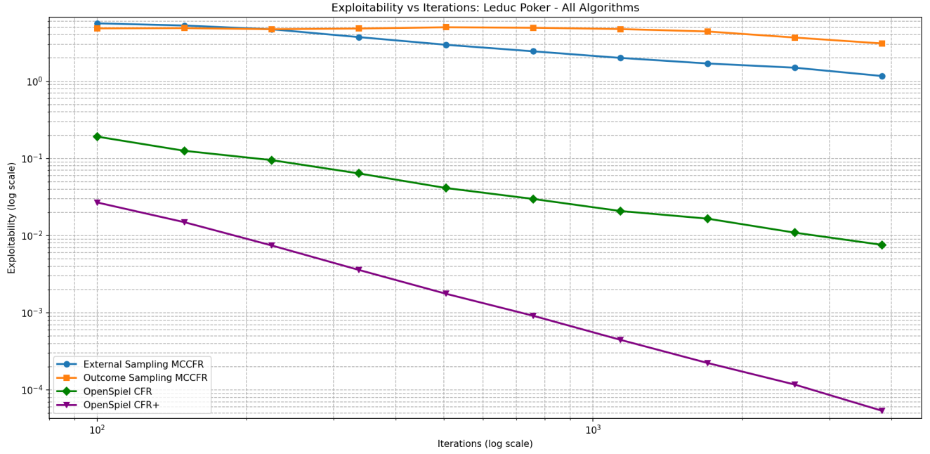
Figure 6: Leduc Poker — Exploitability vs Iterations
