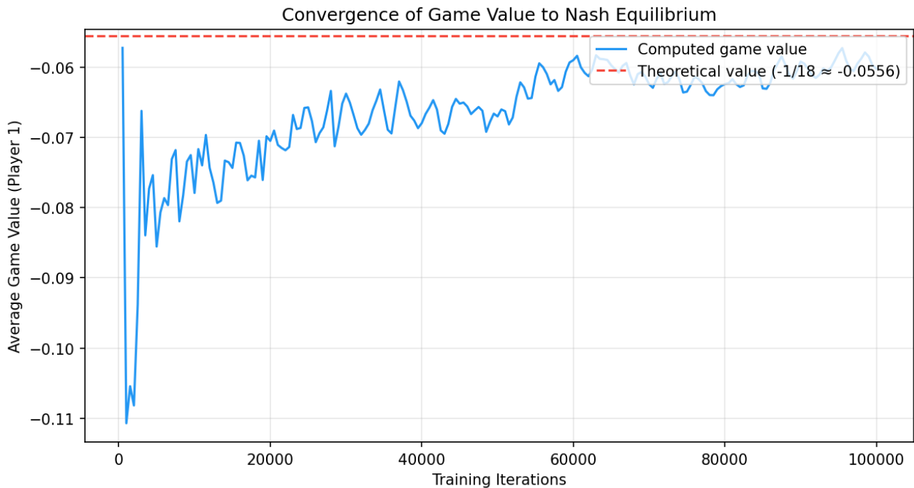
Figure 3: Game Value Convergence
