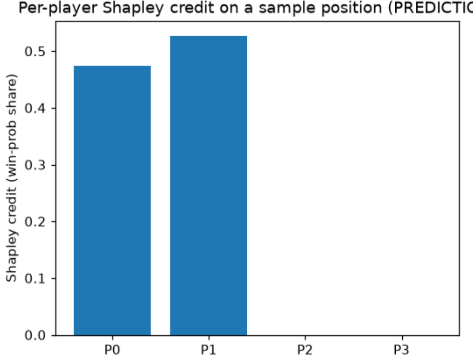
Figure 67: Shapley credit attribution on SLS positions: near-flat across seats in the symmetric case (spread 0.013, post-fix), and fully concentrated on the strong pair in the asymmetric [8,8,1,1] case. Credit tracks real contribution once the engine tie-break is unbiased.
