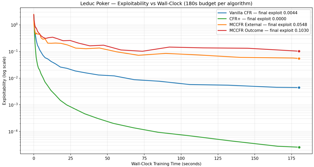
Фигура 6: Exploitability vs Wall-Clock Time
