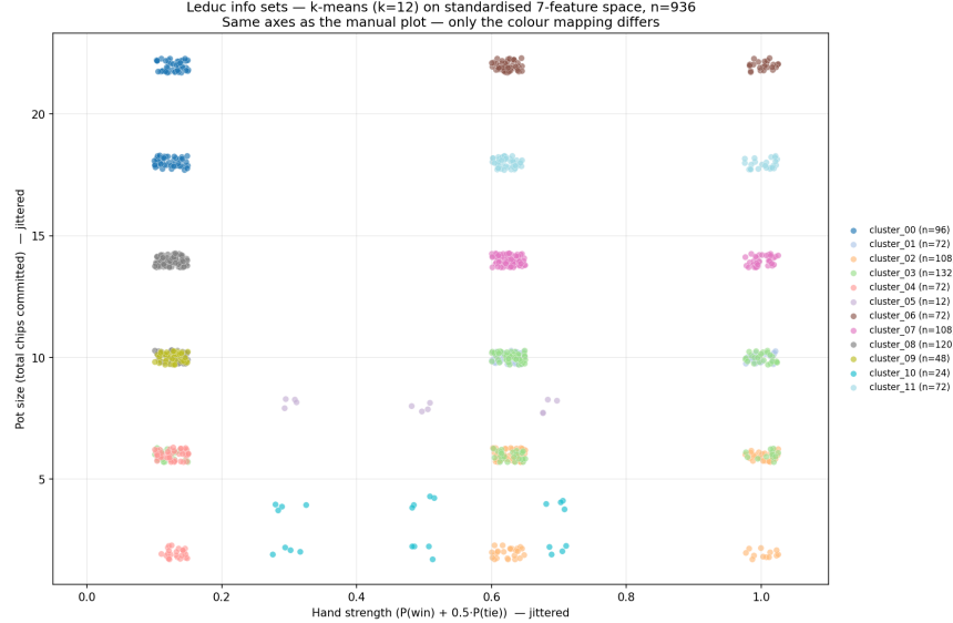
Figure 1: InfoSet grouping via K-means
