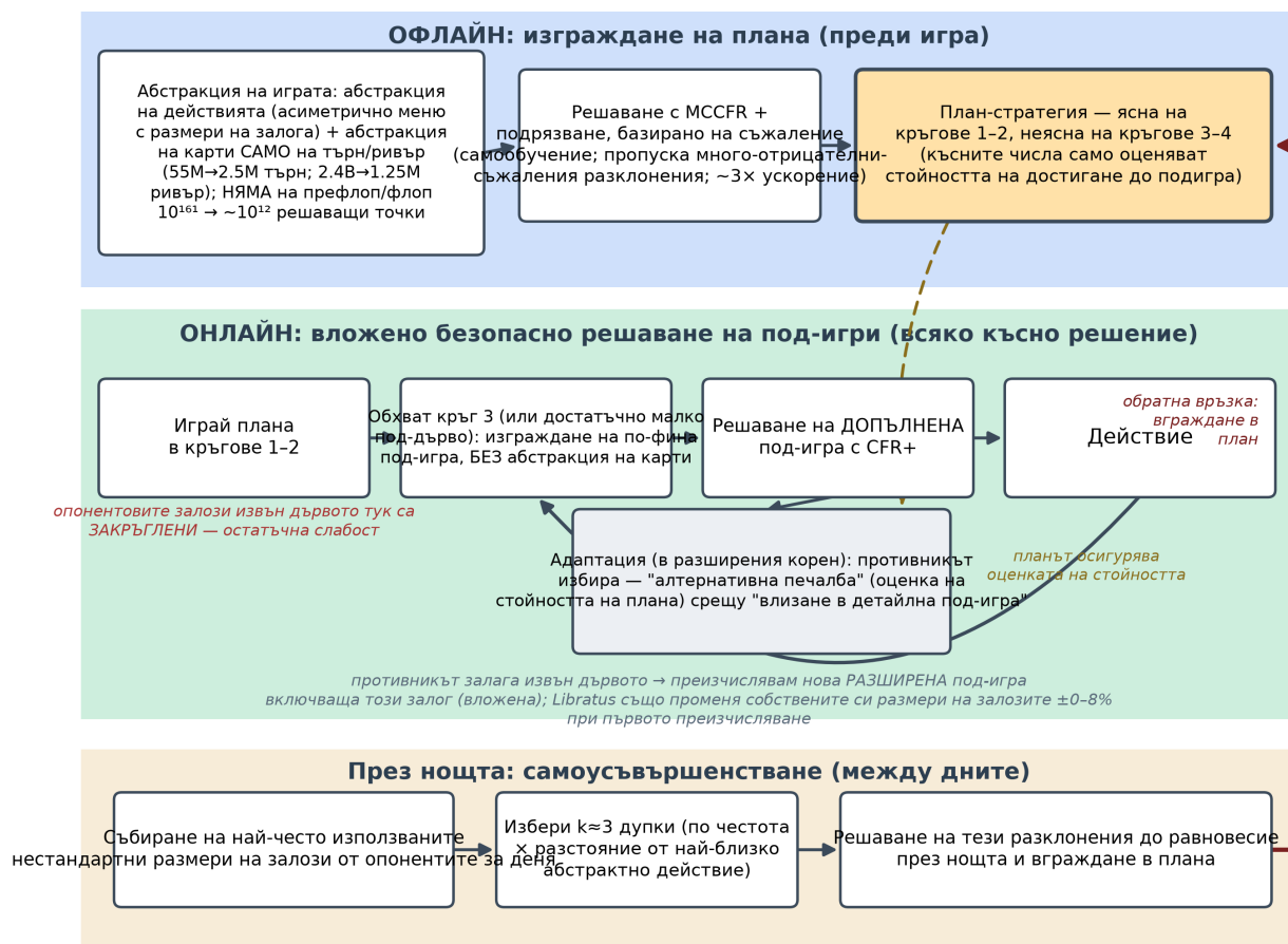
Фигура 2: Libratus's three-module pipeline: an offline blueprint (top), the online nested safe-subgame solver that plays it (middle), and the overnight self-improver that grafts solved holes back into the blueprint (bottom, feedback arrow).
