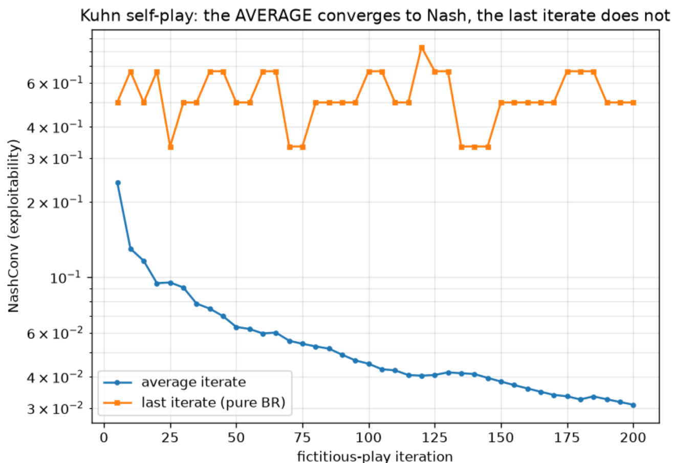
Фигура 9: Self-play on Kuhn: the average-iterate exploitability (NashConv) falls steadily toward zero while the last-iterate exploitability keeps oscillating. This is why self-play and PSRO rely on averaging over a population rather than trusting the most recent policy.
