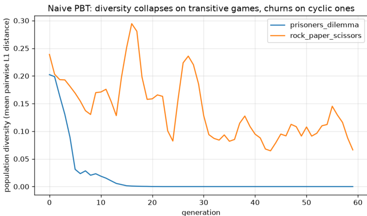
Фигура 7: Mini-PBT diversity: on the transitive Prisoner’s Dilemma the population collapses to a single strategy (diversity → 0), while on cyclic Rock-Paper-Scissors it churns indefinitely (0.07-0.29) as it chases the wheel of counters. Game structure, not population size, decides whether diversity survives.
