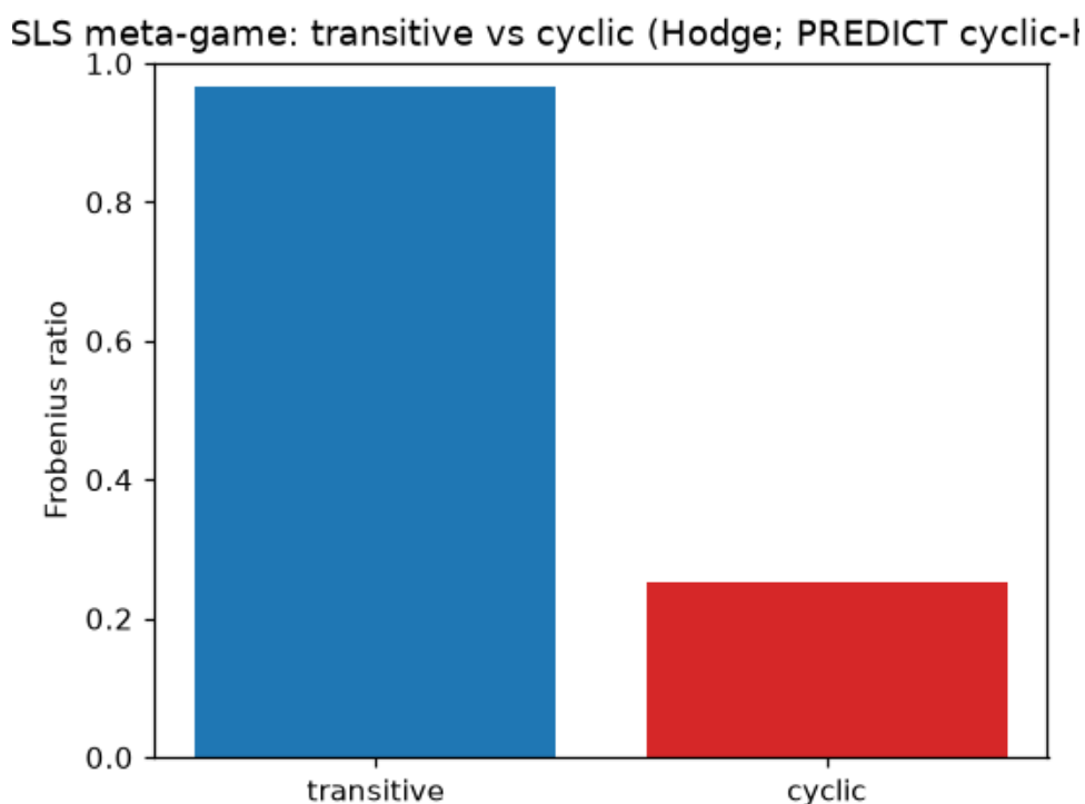
Фигура 8: Spinning-top transitive/cyclic ratios: the skill-ladder pool is transitive-dominant (cyclic \sim 0.25-0.31 ), while the coalition pool is strongly cyclic ( \sim 0.57-0.69 ). Coalition play injects large non-transitivity, confirming the Step-10 direction while staying just under strict cyclic dominance.
