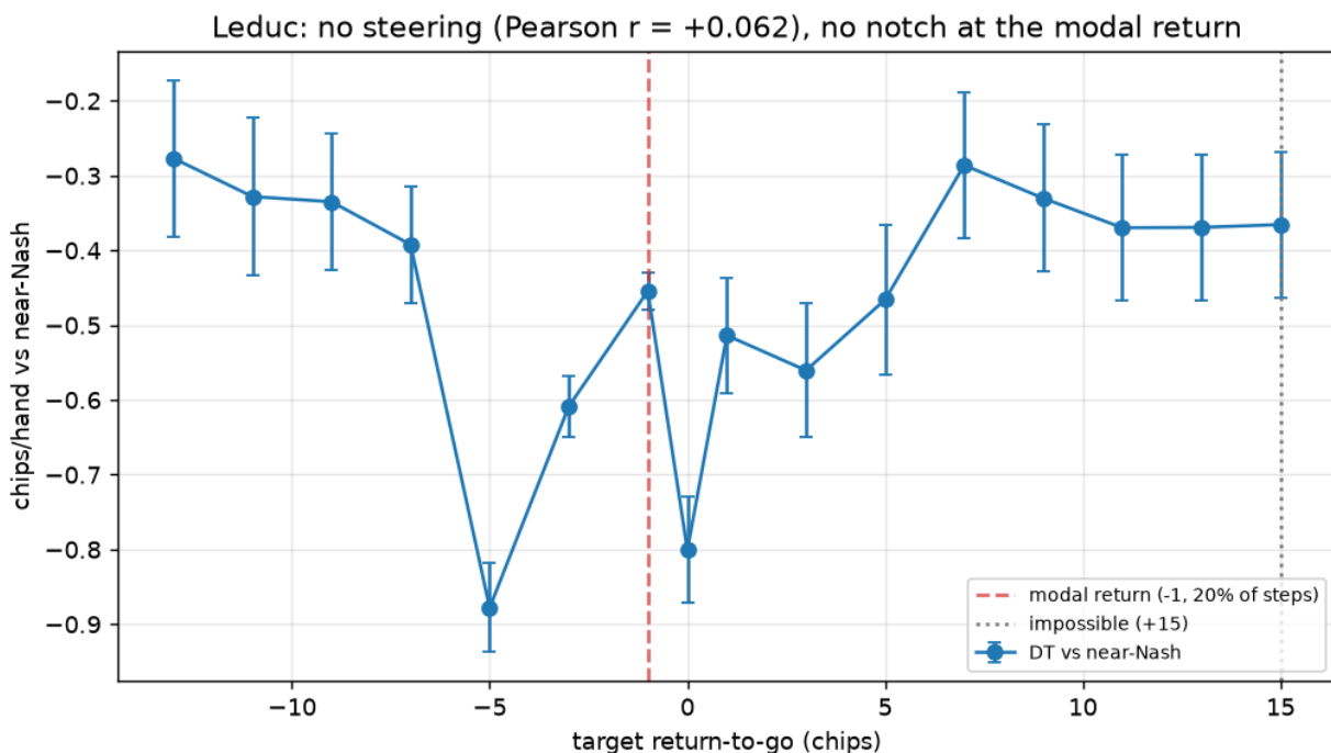
Фигура 7: DT performance against the conditioned target return on Ледюк, with standard errors. There is no collapse at the modal return and no monotone trend.
