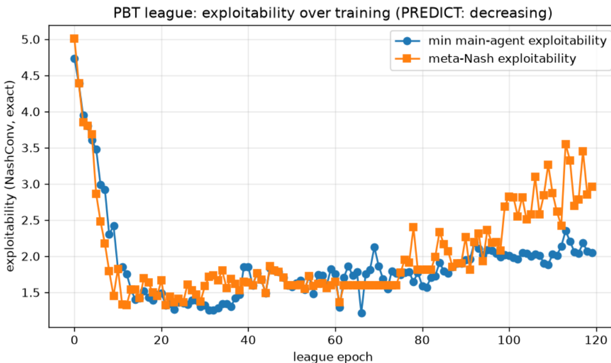
Фигура 3: League exploitability over training (scale, 120 epochs): min-main and meta-Nash exploitability both fall steeply to a minimum near epoch 60 (min-main \sim 1.21 , meta-Nash \sim 1.32 ) and then regress upward ( \sim 2.05 / \sim 2.96 ) by epoch 119. A running league is not a monotonically improving one; the best agents are frozen snapshots from mid-run.
