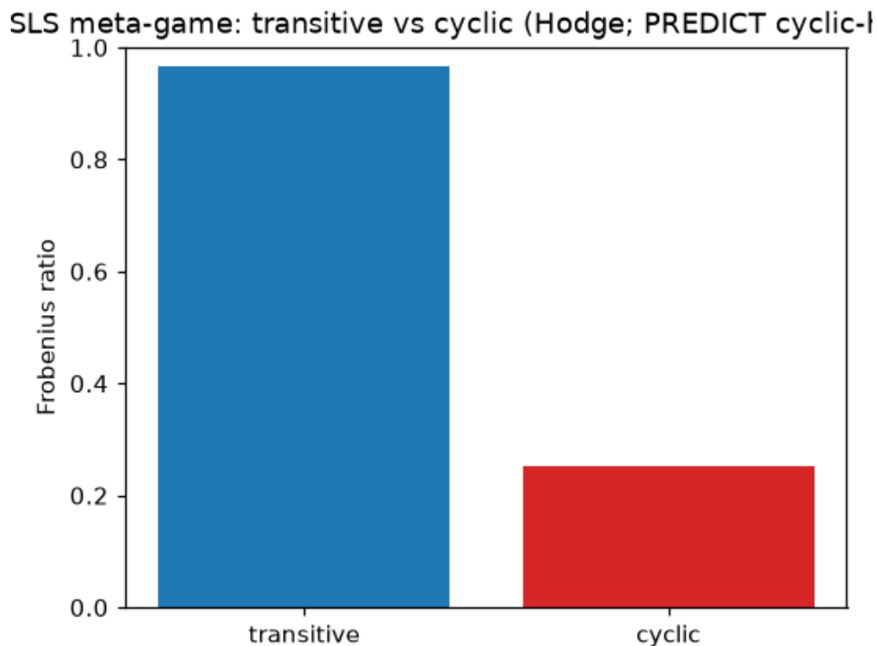
Фигура 8: Spinning-top transitive/cyclic ratios: the skill-ladder pool is transitive-dominant (cyclic ~0.25-0.31), while the coalition pool is strongly cyclic (~0.57-0.69). Coalition play injects large non-transitivity, confirming the Step-10 direction while staying just under strict cyclic dominance.
