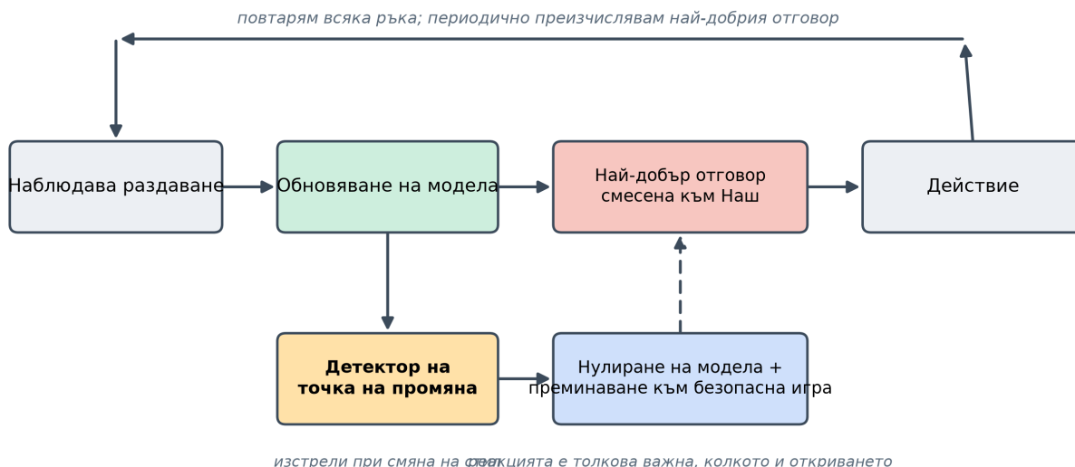
Фигура 7: The adaptive exploitation loop: observe, update the model, best-respond (blended toward Nash for safety), and act; a change-point detector can reset the model when the opponent's style shifts.
