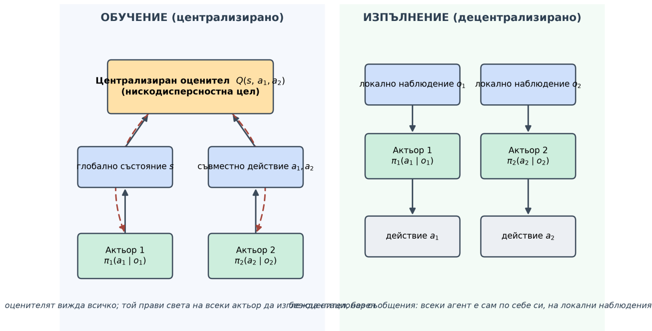
Фигура 5: CTDE architecture. During training a centralized critic (or value function) sees the global state and the joint action and produces low-variance value targets; during execution each actor acts on its own local observation with no access to the critic and no message passing. The training/execution asymmetry is what makes the world look stationary to the learner without cheating at showtime.
