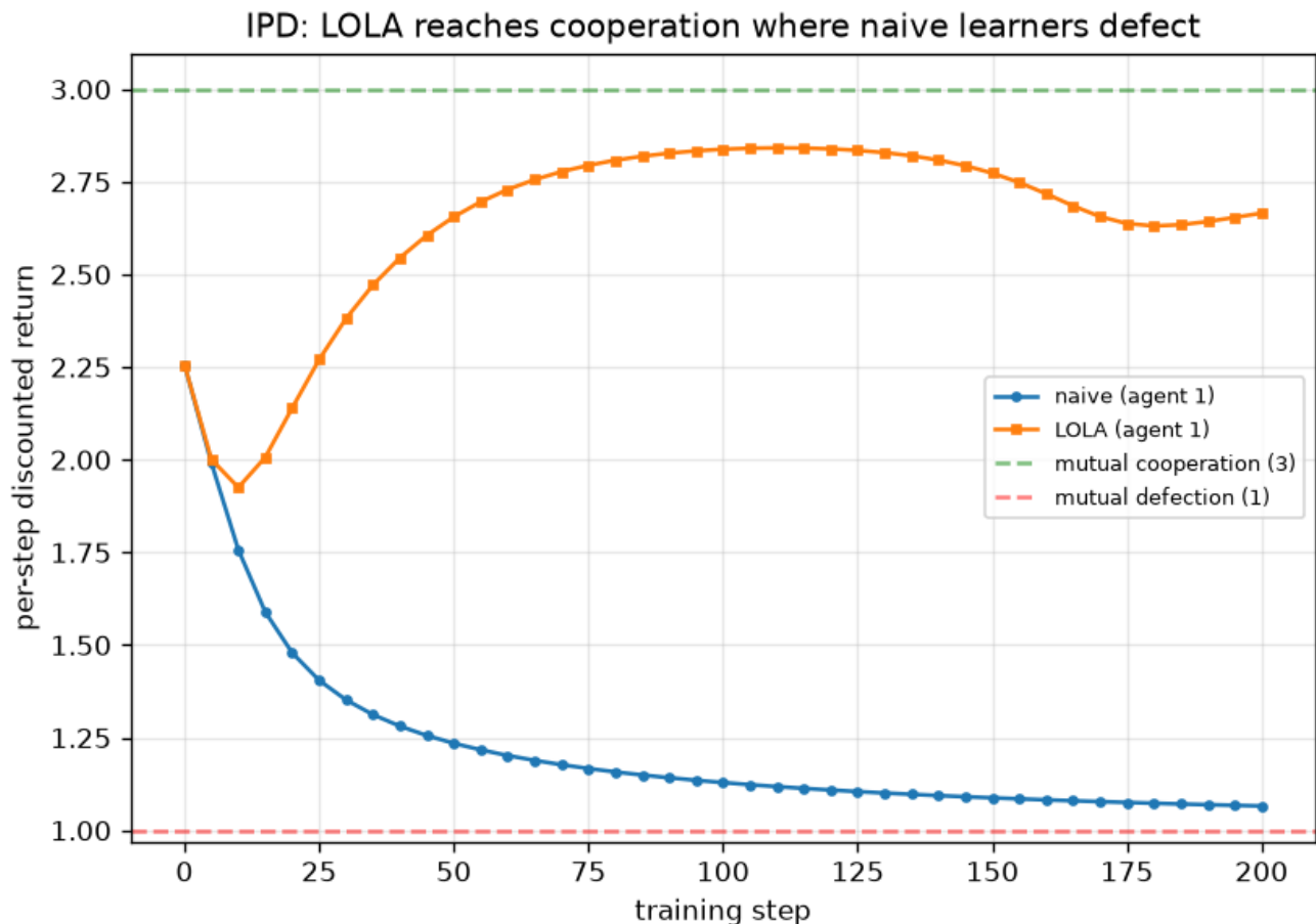
Фигура 10: LOLA vs naive learners on the Iterated Prisoner’s Dilemma: naive learners’ per-step return collapses toward mutual defection (~1), while LOLA learners’ return climbs toward mutual cooperation (~2.8). Anticipating the opponent’s next learning step is what reshapes the dynamics from defection to cooperation.
