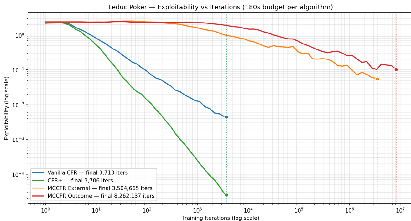
Фигура 5: Exploitability vs Iterations
