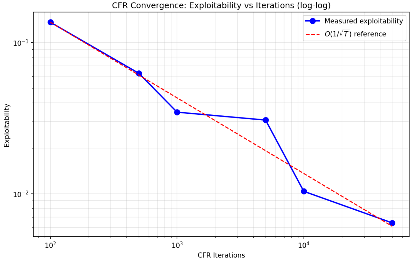
Figure 2: Exploitability Convergence
