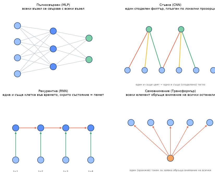
Фигура 1: Connectivity of the four layer families: a fully connected MLP, a convolution that reuses one filter across local windows, a recurrent cell reused across time, and self-attention.
