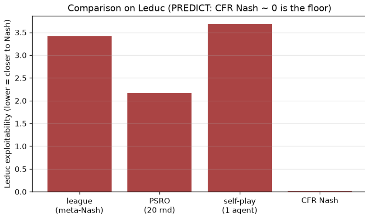
Фигура 9: Final Ледюк exploitability by method (scale): CFR-Nash floor \sim 0.01 ; the league's best individual (1.31) beats PSRO (2.16) and self-play (3.68); the league's meta-Nash mixture (3.42) is the weakest learned result.
