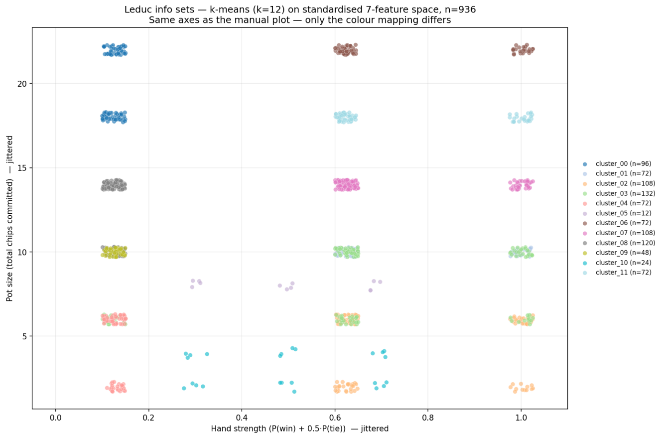
Figure 1: Infoset grouping via K-means
