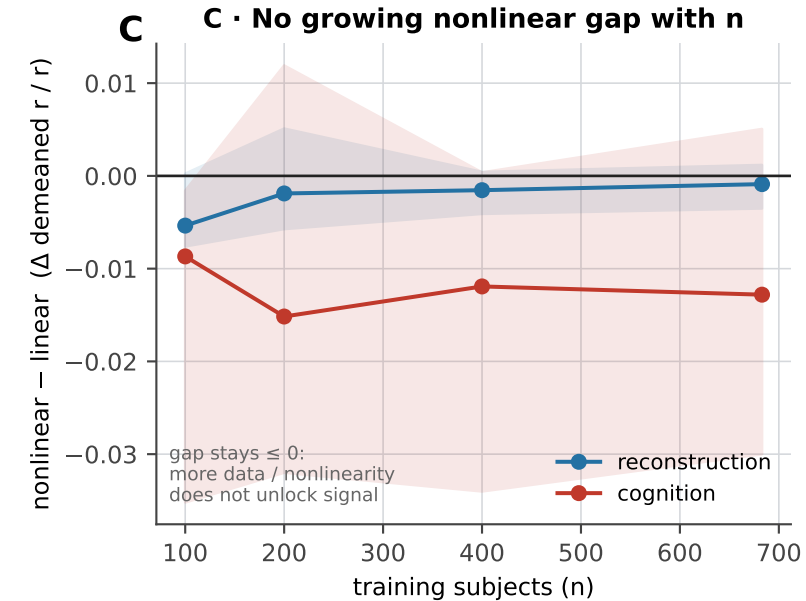
Figure 4 · The missing utility is not recovered by reduction, model class, structural detail, sample size, or FC denoising
