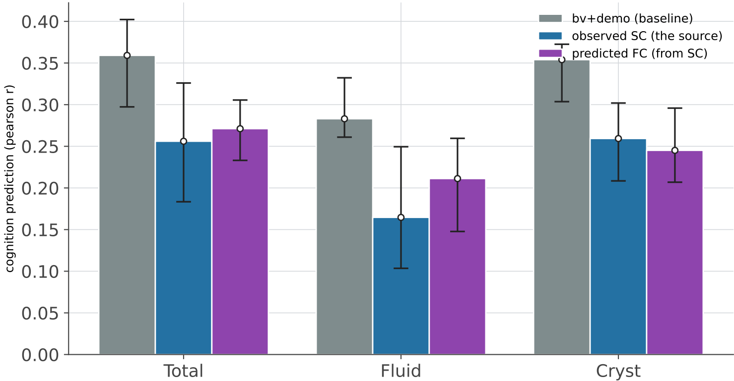
Cognition: baseline vs SC vs predicted FC (BayesianRidge, 4S456Parcels (456 regions))
