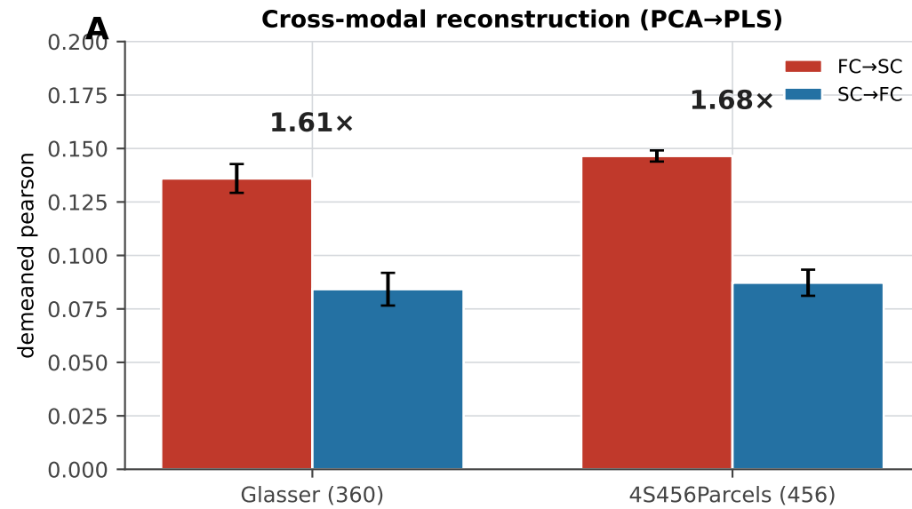
Figure 2 · Cross-modal connectome prediction is directional: FC predicts SC better than SC predicts FC
