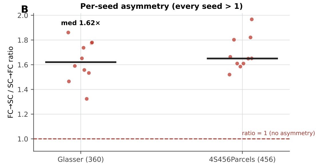
Figure 2 · Cross-modal connectome prediction is directional: FC predicts SC better than SC predicts FC
