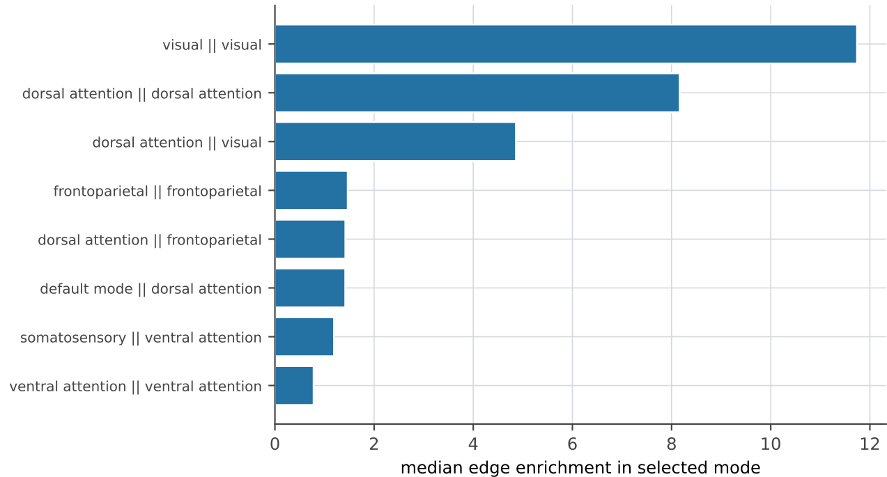
Glasser: network-pair enrichment (top 8, visual/DAN dominate)
