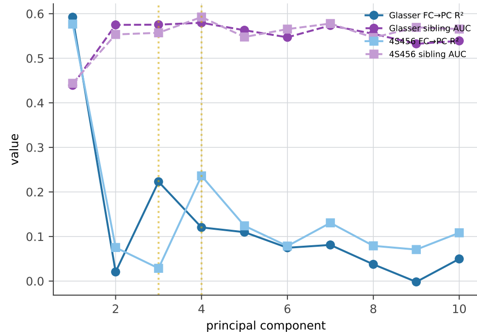
FC-predictability & family AUC per PC (gold = selected mode)
