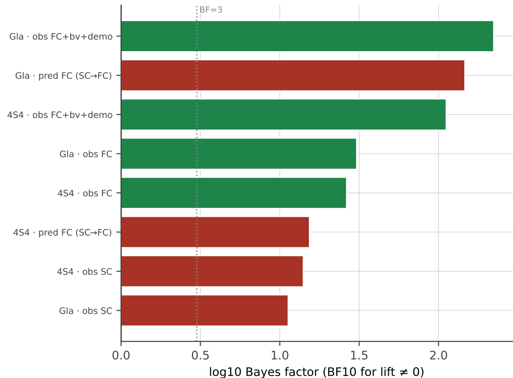
B · Strength of evidence for a lift (CogCryst) green = helps, red = harms; length = evidence
