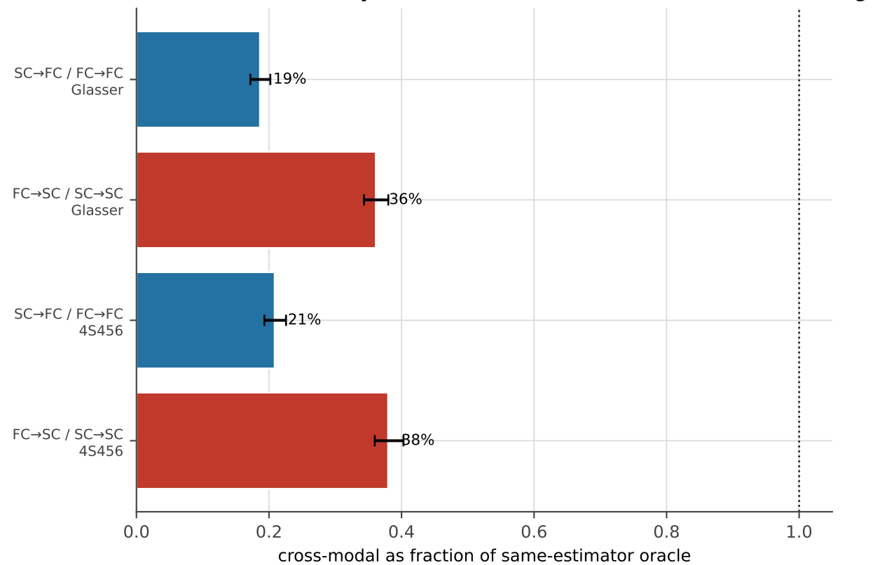
B · Cross-modal loss: only ~20% (→FC) / ~37% (→SC) of the model ceiling
