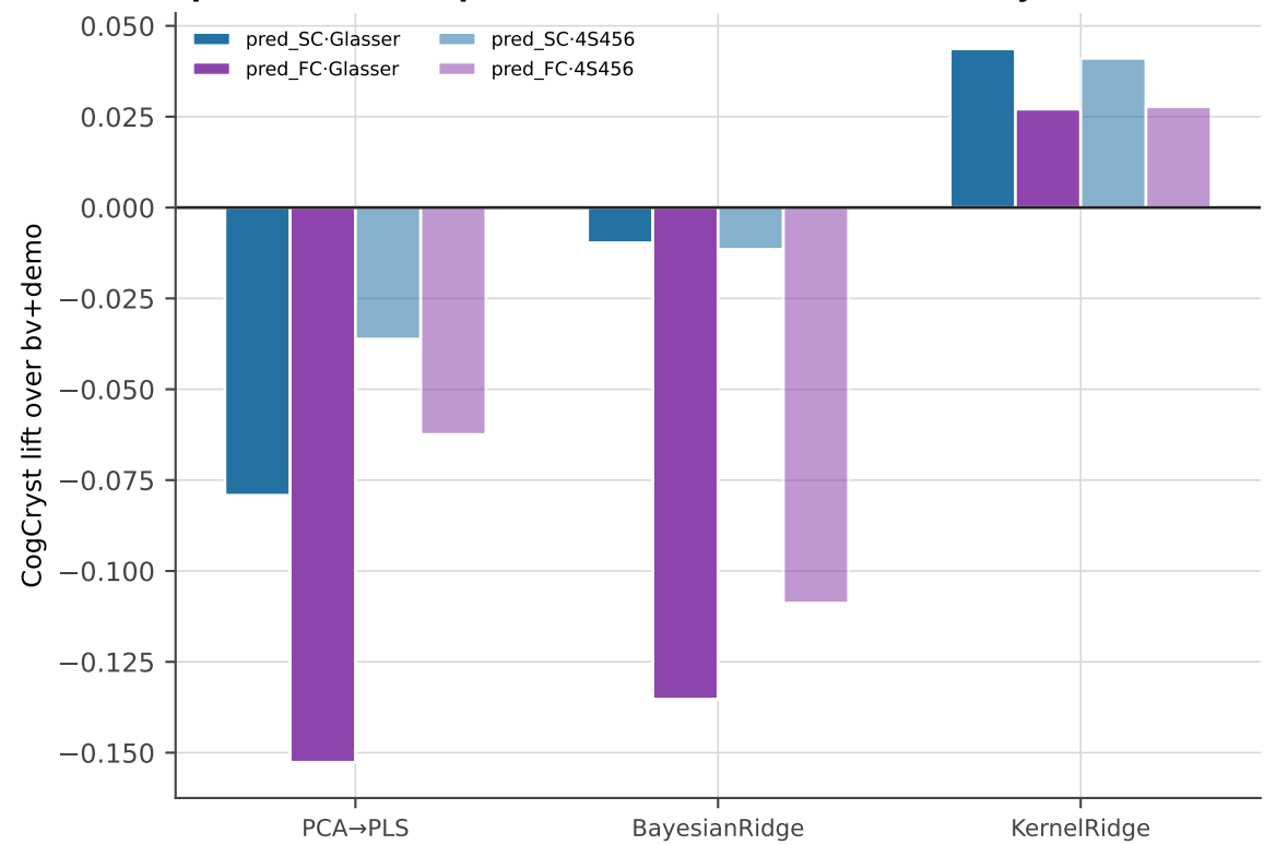
A · pred FC harm > pred SC at matched dimensionality (all estimators)
