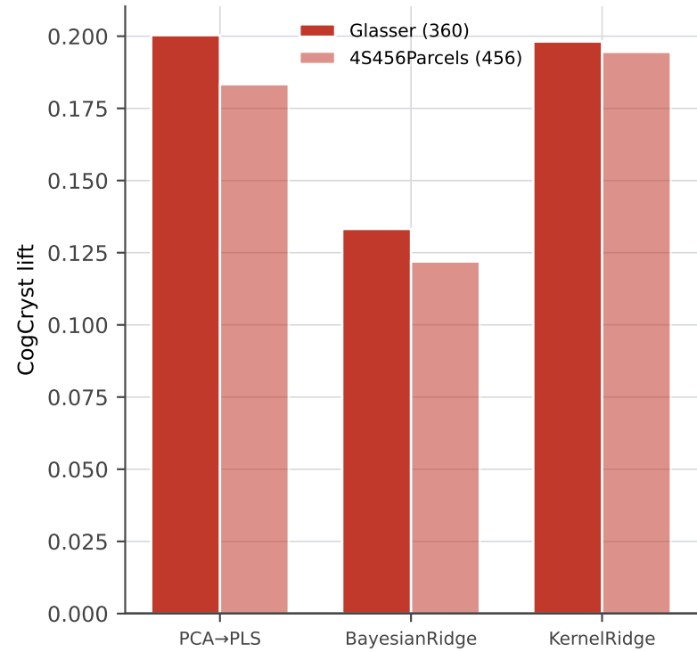
C C · obs FC lift across estimators
