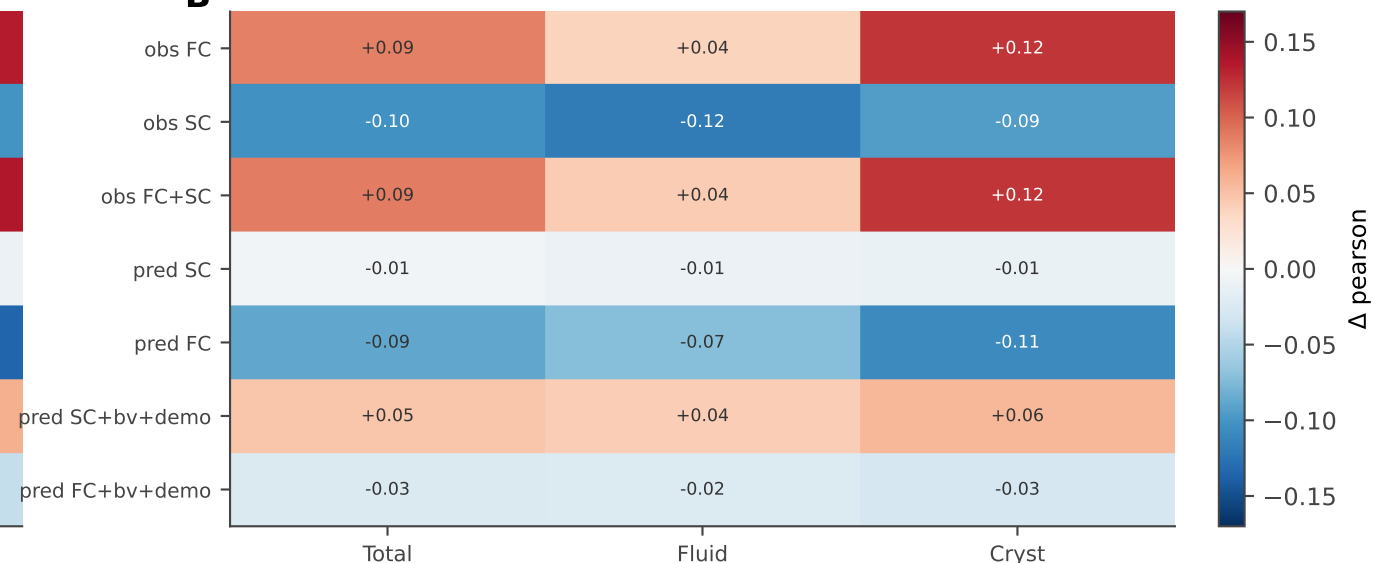
B · lift over bv+demo — 4S456Parcels (456)
