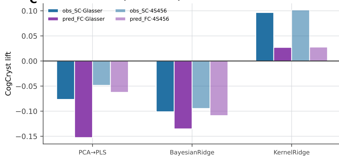
C · SC underperforms & pred FC harms (all estimators)
