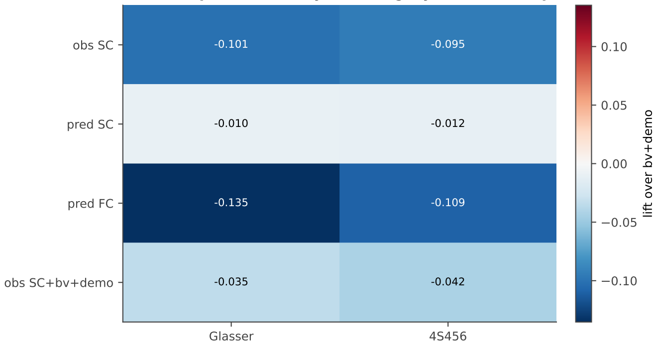
F5 SC/imputation utility wall (CogCryst) — heatmap
