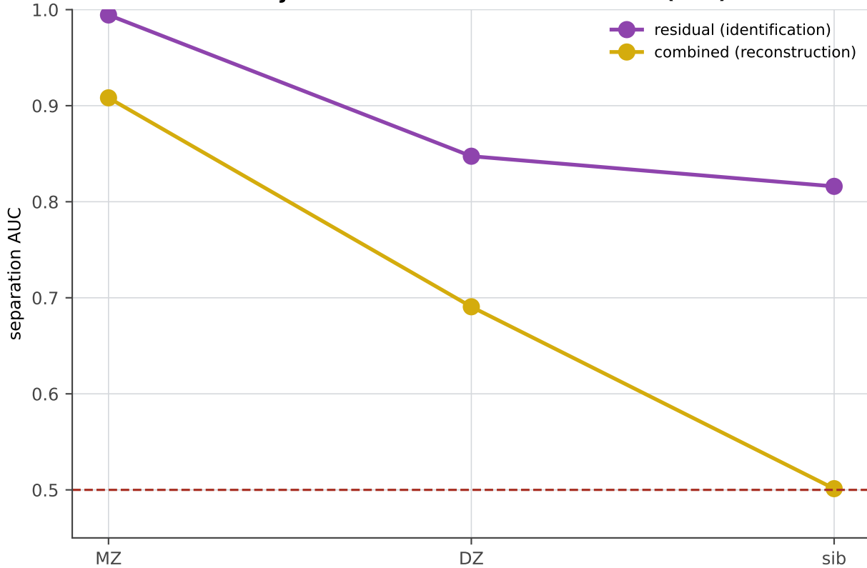
F7 objective tradeoff — 4S456Parcels (456)
