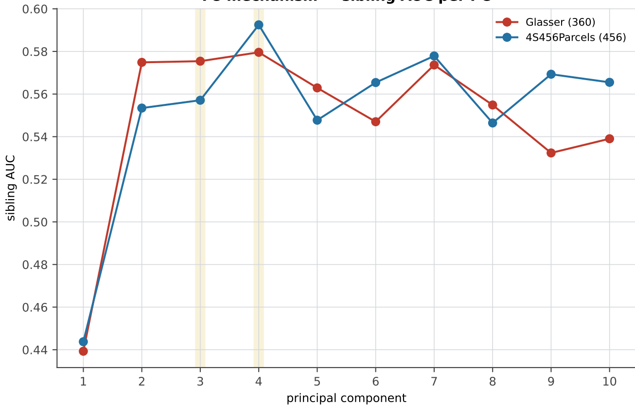
F8 mechanism — sibling AUC per PC
