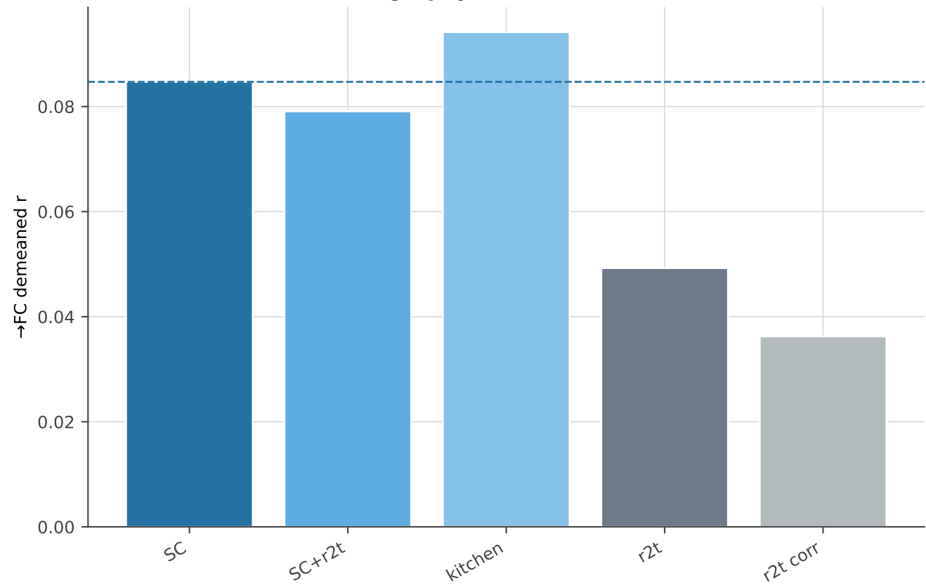
F9 tractography → FC (Glasser) — bars
