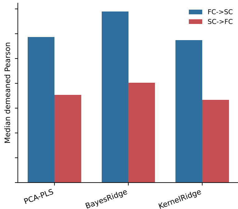
F1: FC->SC exceeds SC->FC across parcellations and model families
