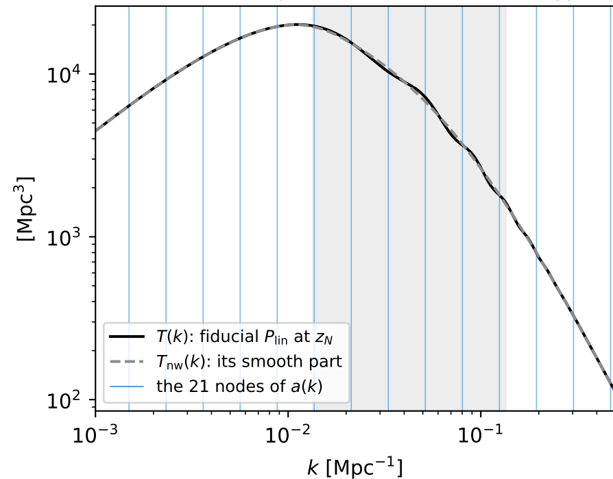
(a) fixed template (fiducial cosmology)
