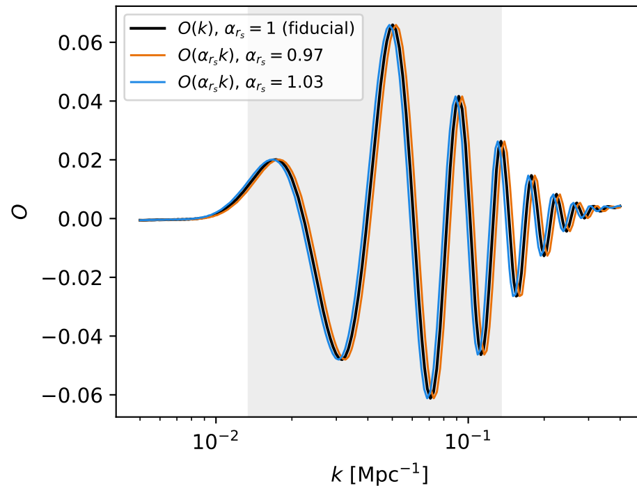
(b) \alpha_{r_s} slides the wiggles
