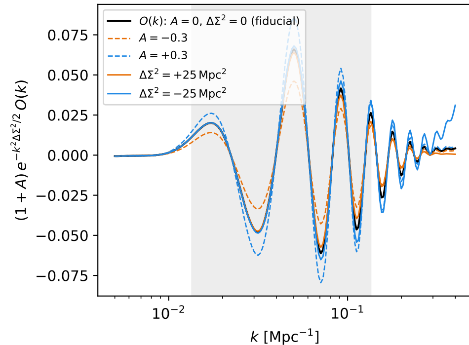
(c) amplitude A (dashed), damping \Delta\Sigma^2 (solid)
