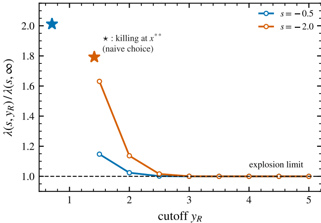
(a) the killing boundary matters
