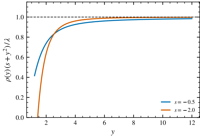
(b) flux tail \rho \rightarrow \lambda/(s + y^2)
