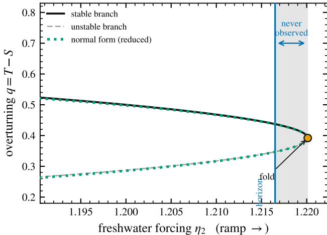
(b) the reduction, and where observation ends
