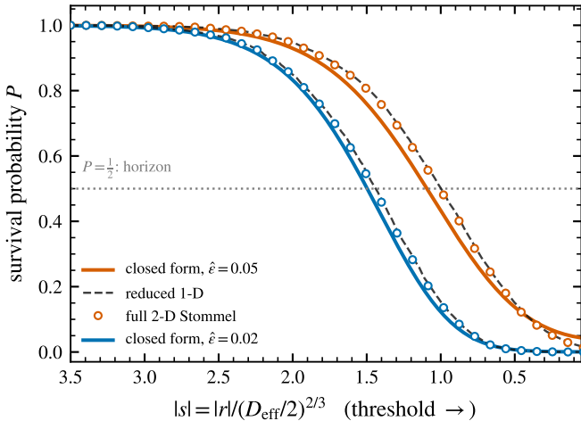
(a) prediction vs. the full two-dimensional model
