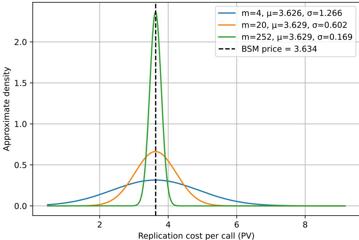
Approximate Distributions of Replication Cost for Different Hedge Frequencies
