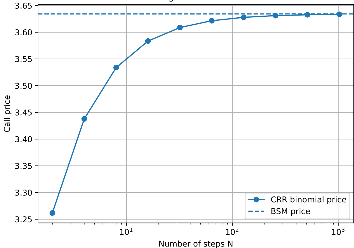
CRR Convergence to Black-Scholes
