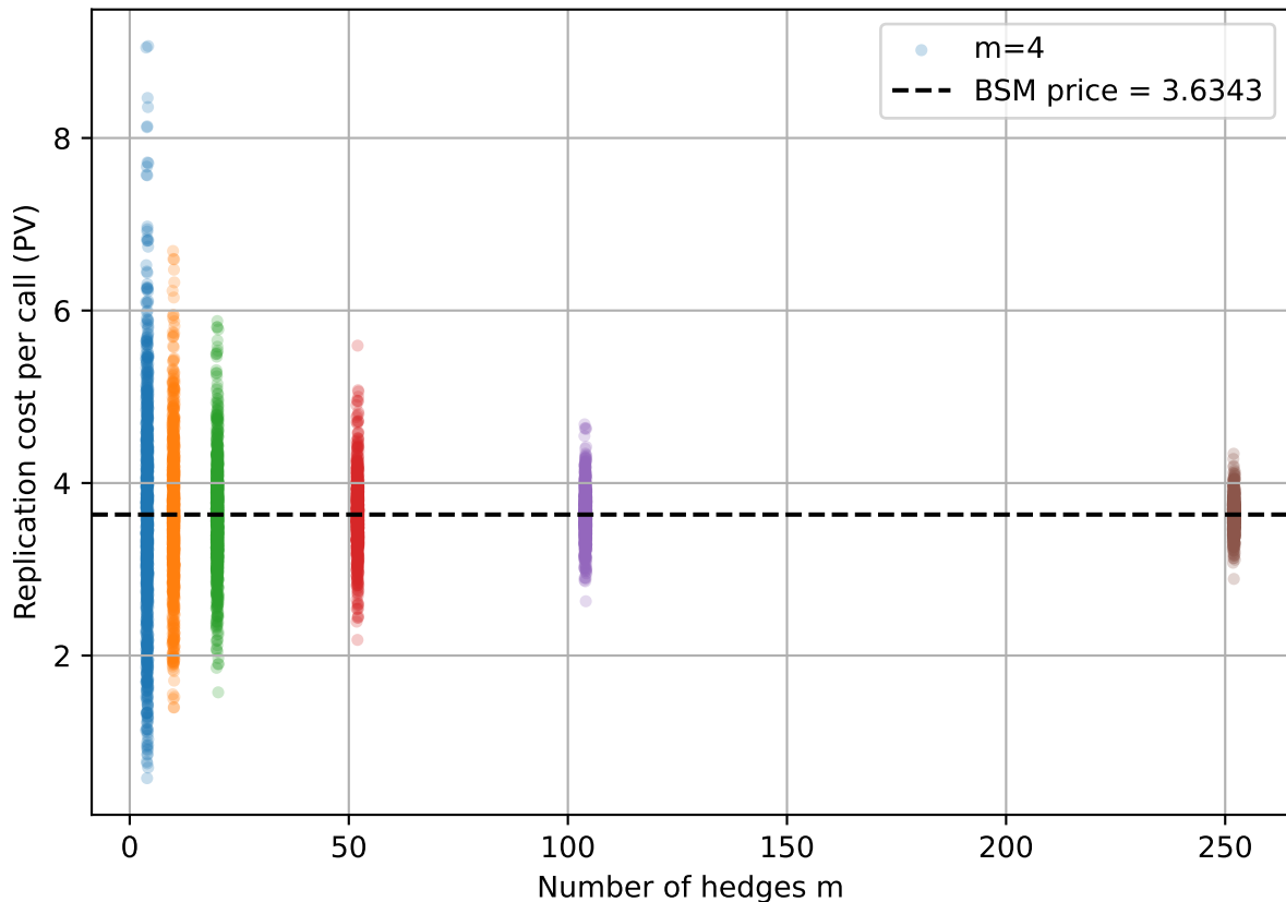
Per-path Replication Costs vs Hedge Frequency
