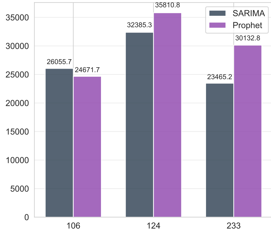
RMSE
