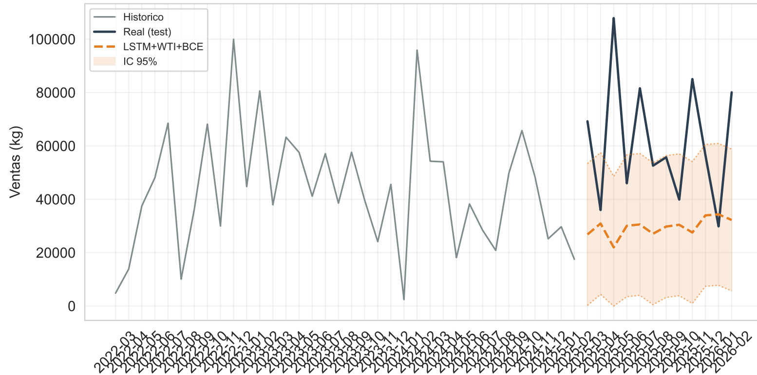
LSTM — 124 RMSE=40,412 SMAPE=64.28%
