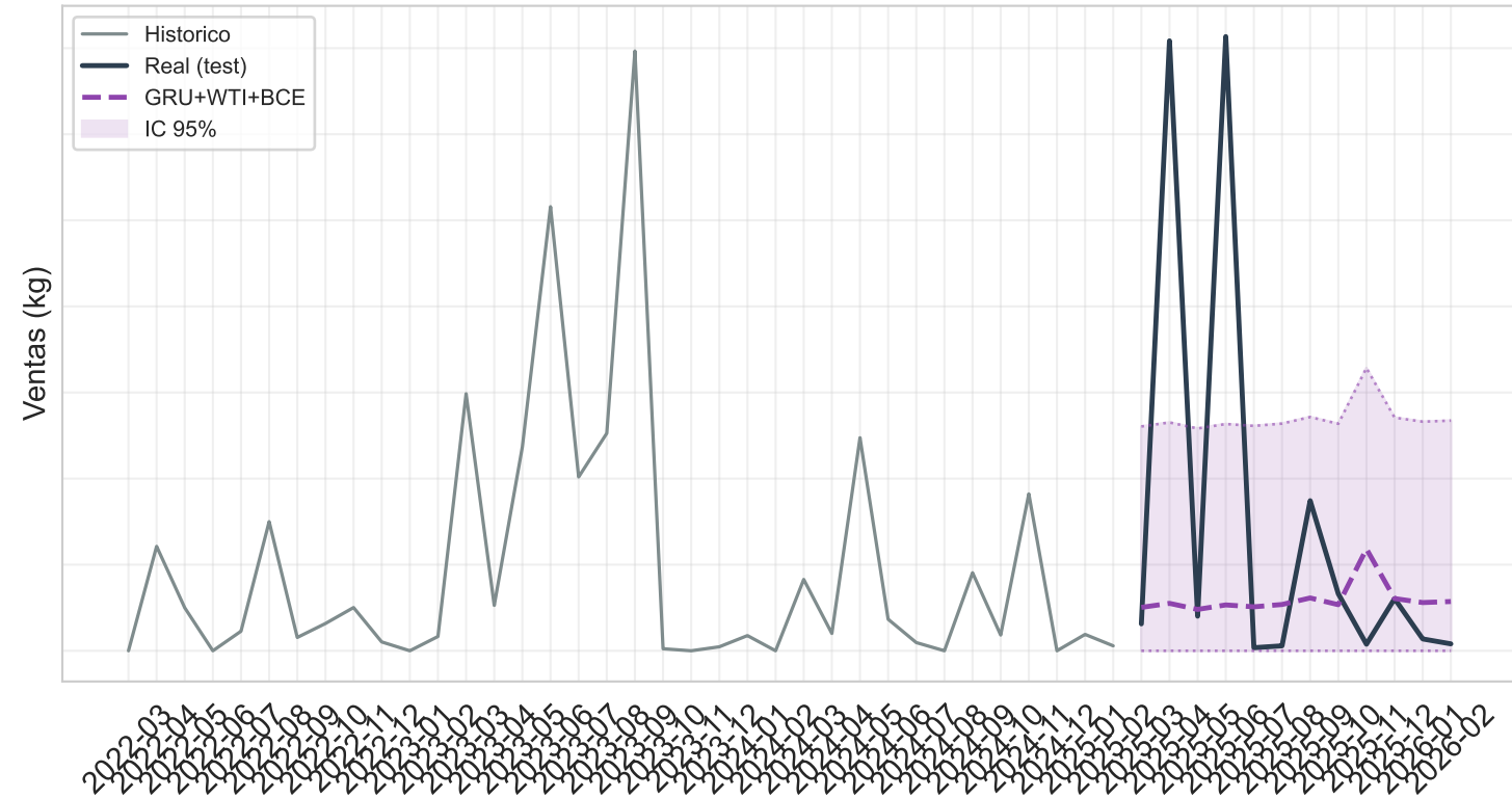
GRU — 106 RMSE=27,344 SMAPE=109.03%
