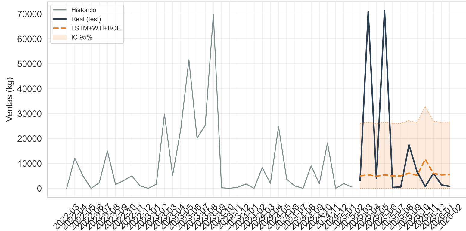
LSTM — 106 RMSE=27,323 SMAPE=108.85%
