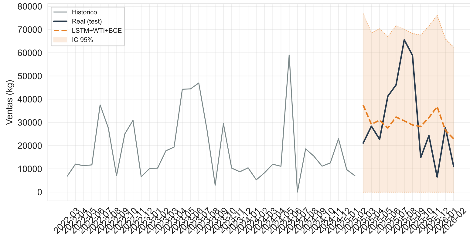
LSTM — 233 RMSE=18,554 SMAPE=50.73%
