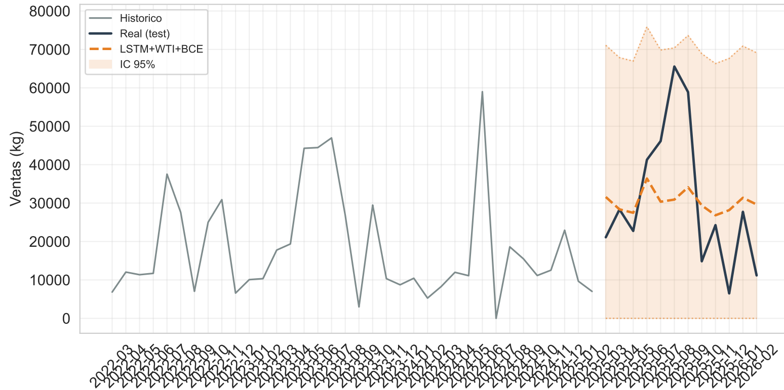
LSTM — 233 RMSE=16,486 SMAPE=45.12%
