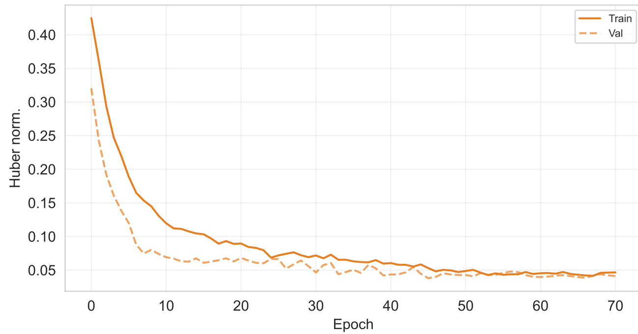
LSTM — 233 (71 epochs)
