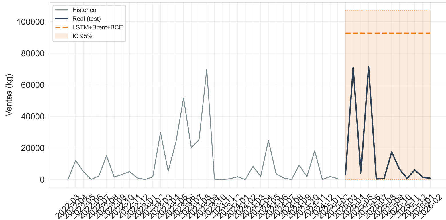
LSTM — 106 RMSE=81,523 SMAPE=157.69%
