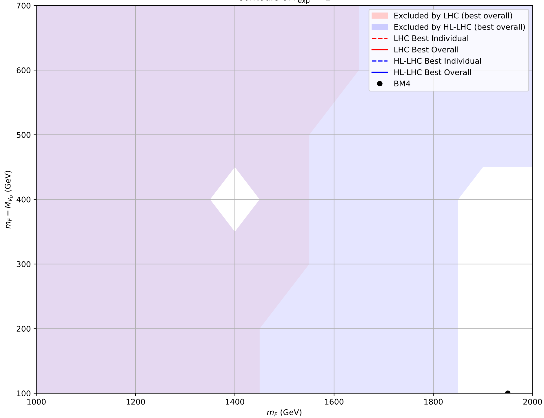
Contours of r_{\text{exp}}^{\text{cons}} = 1
