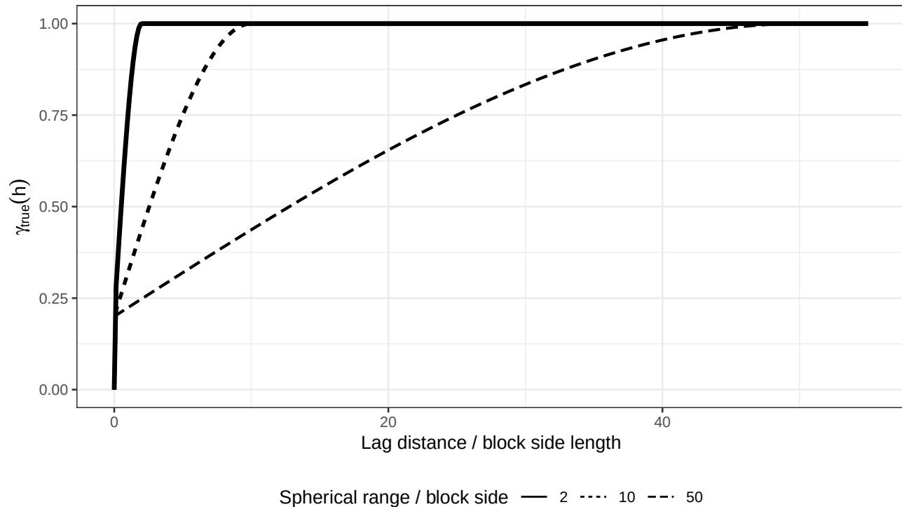
Latent true spherical semivariograms used in the core simulation setup
