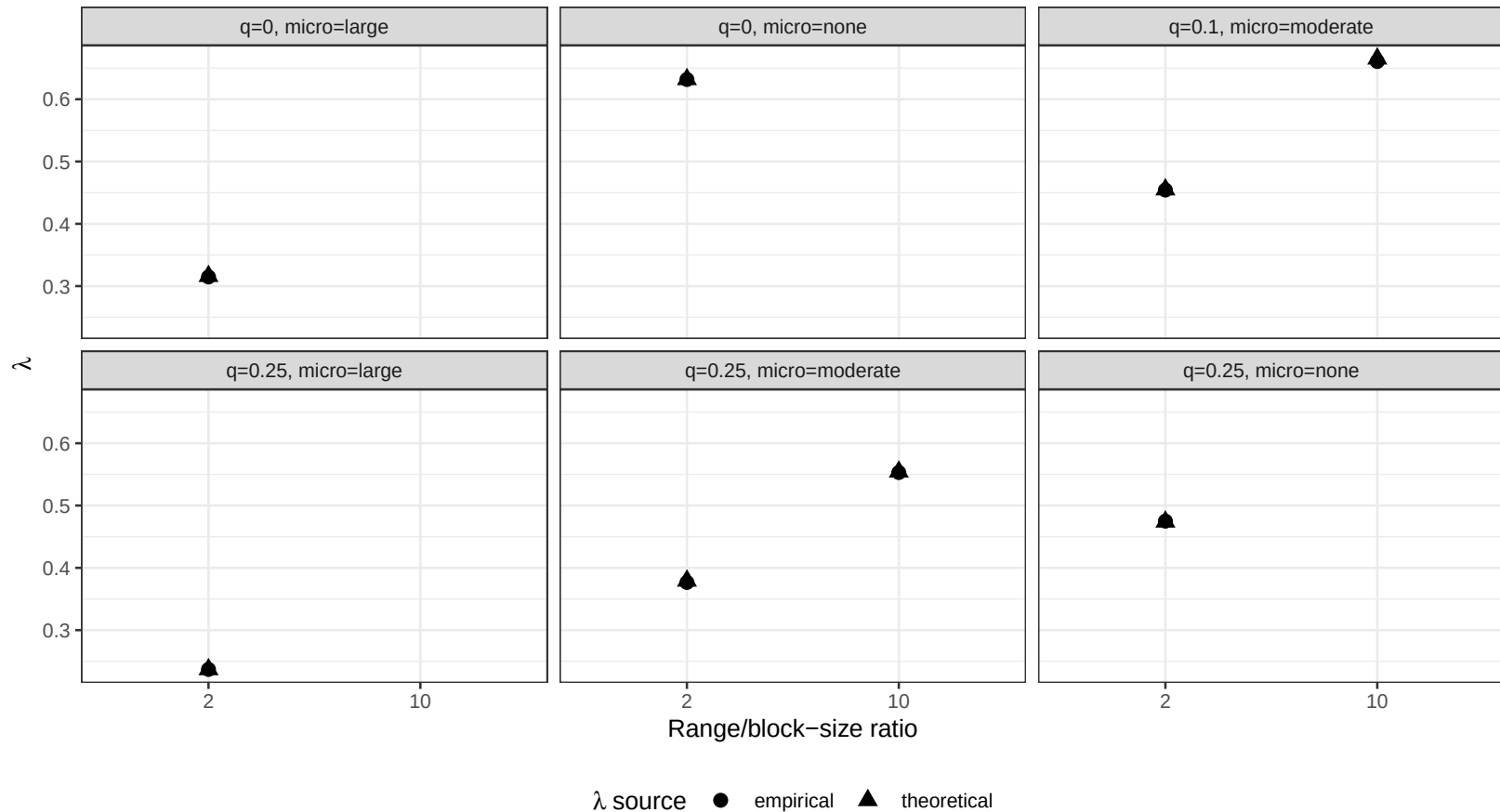
Diagnostic: theoretical versus empirical representativeness in additional scenarios
