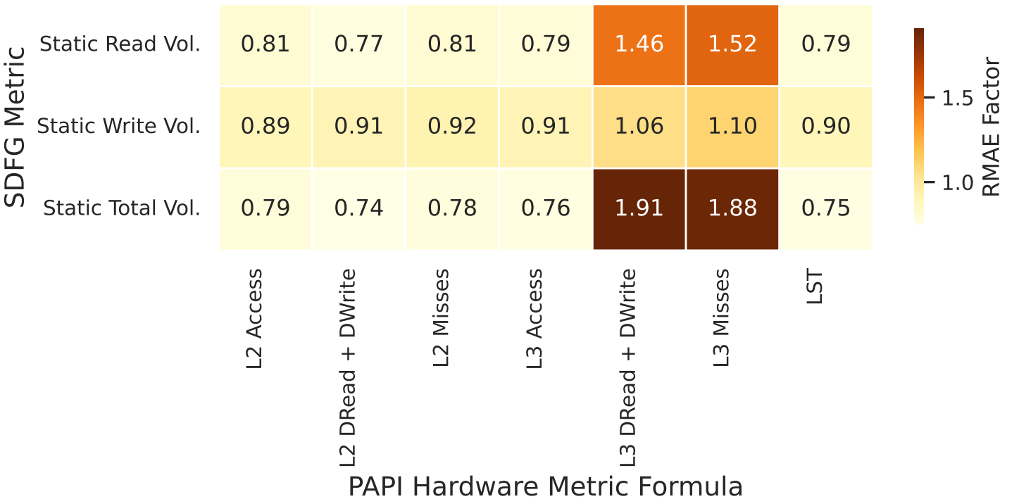
Prediction Error: RMAE
