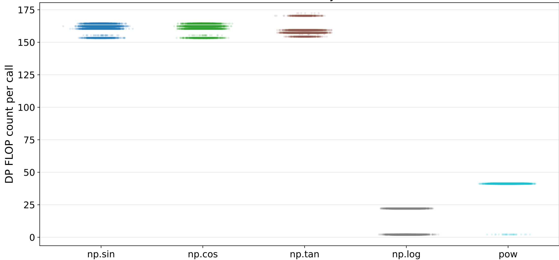
Discrete FLOP-count variability of math functions
