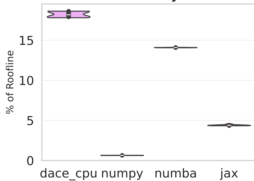
cholesky
