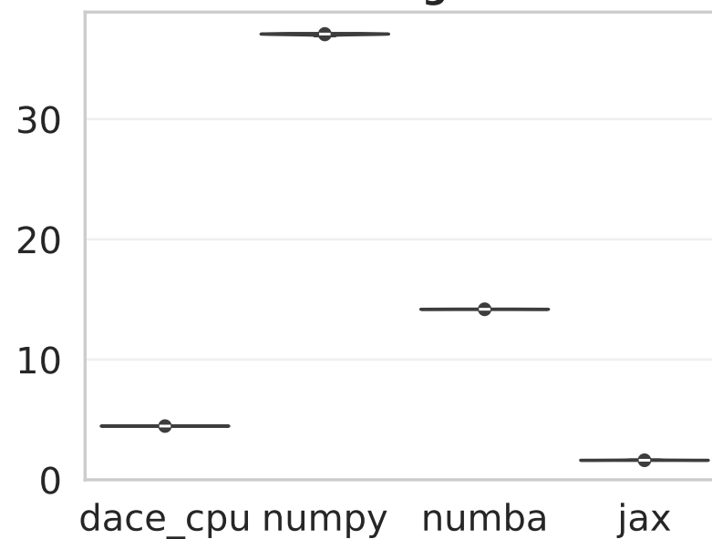
compute
