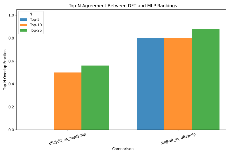
Figure 5.3: Top- N overlap for Si interfaces.
