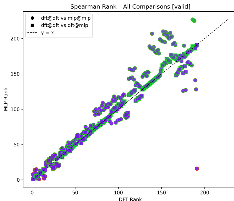
Figure 5.2: Spearman correlation for Ge interfaces.
