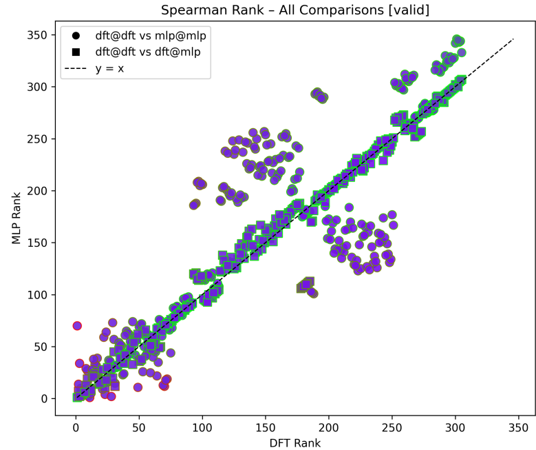
Figure 5.1: Spearman rank correlation for Si interfaces.
