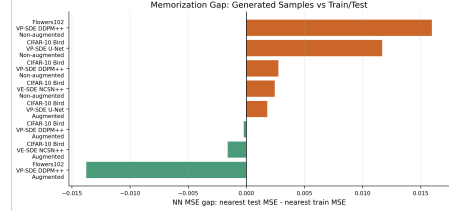
Figure 2: Memorization gap.
