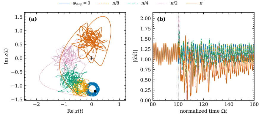
Figure S3. Complex-plane step response of the anomalous pair mode. The pump phase is switched at \Omega t = 100 from zero to \varphi_{\text{step}} = 0, \pi/8, \pi/4, \pi/2 , and \pi . Left: trajectories of z(t) = \langle \hat{a}\hat{a} \rangle \exp(2i\Omega t) in the complex plane. Right: pair-correlation amplitude across the step. The final phase transfer is nearly one-to-one for all tested steps. For \pi/2 and \pi , however, the pair amplitude collapses close to zero, so the instantaneous phase is temporarily ill-defined and phase and amplitude are not dynamically decoupled. The black dot marks the state at the step and the cross marks the origin; the dotted line in the right panel marks the step. Curves are smoothed over a quarter drive period, as in the analysis of Supplement 5.
