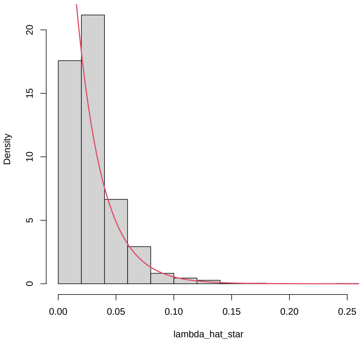
Bootstrap density vs Exp(lambda_hat)
